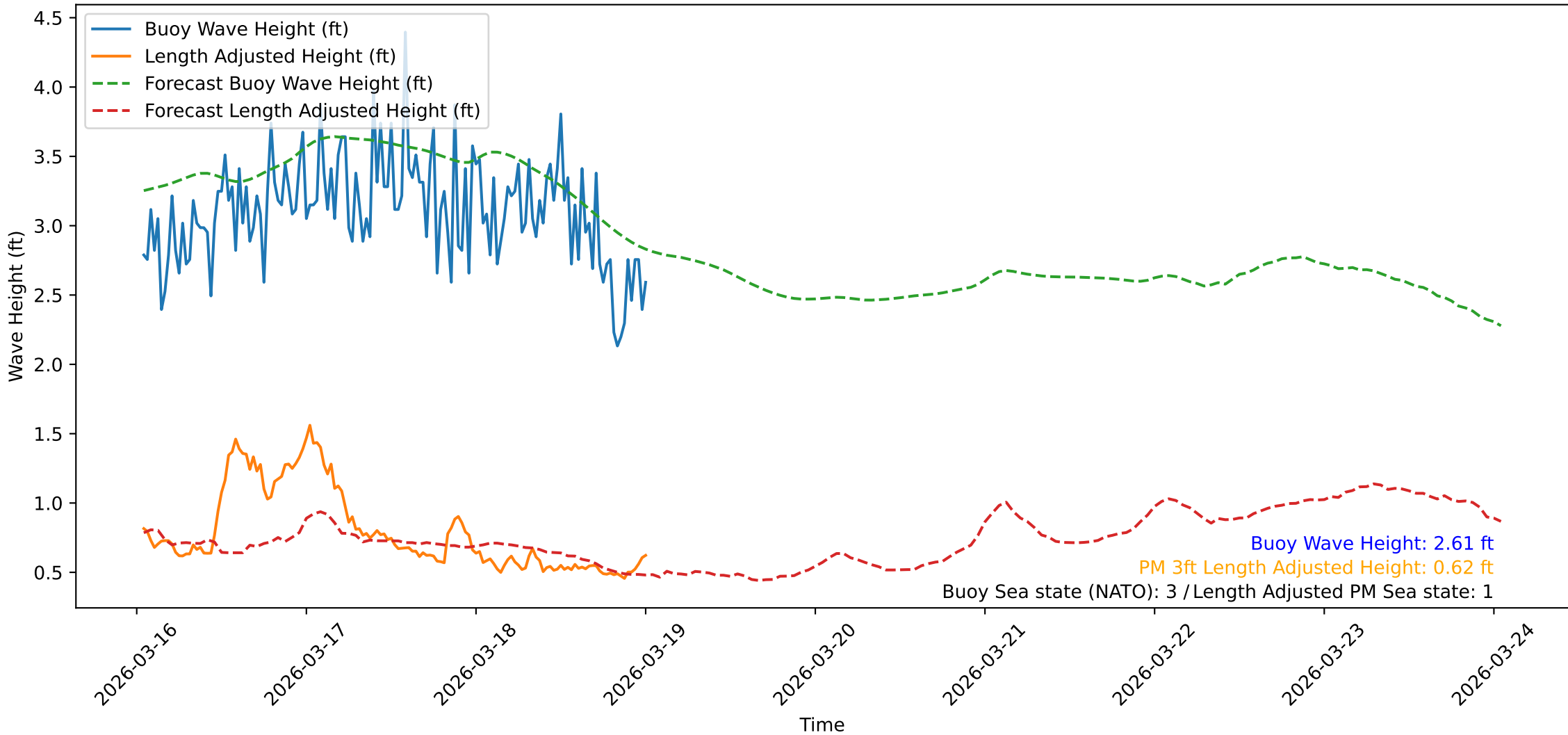
Wave Heights over Time for Oceanside Harbor at 2026-03-19 01:10:32
