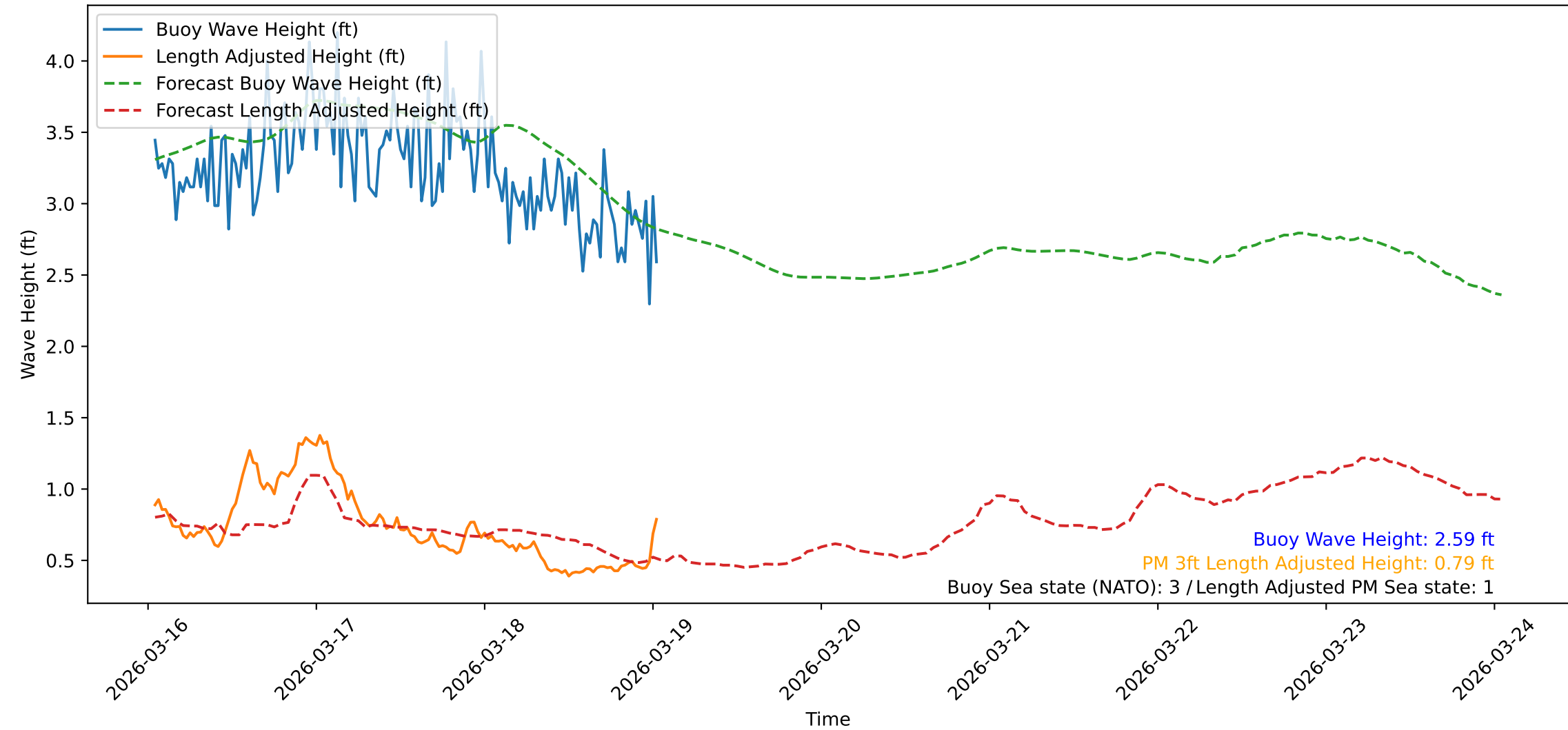
Wave Heights over Time for Green Beach at 2026-03-19 01:11:10
