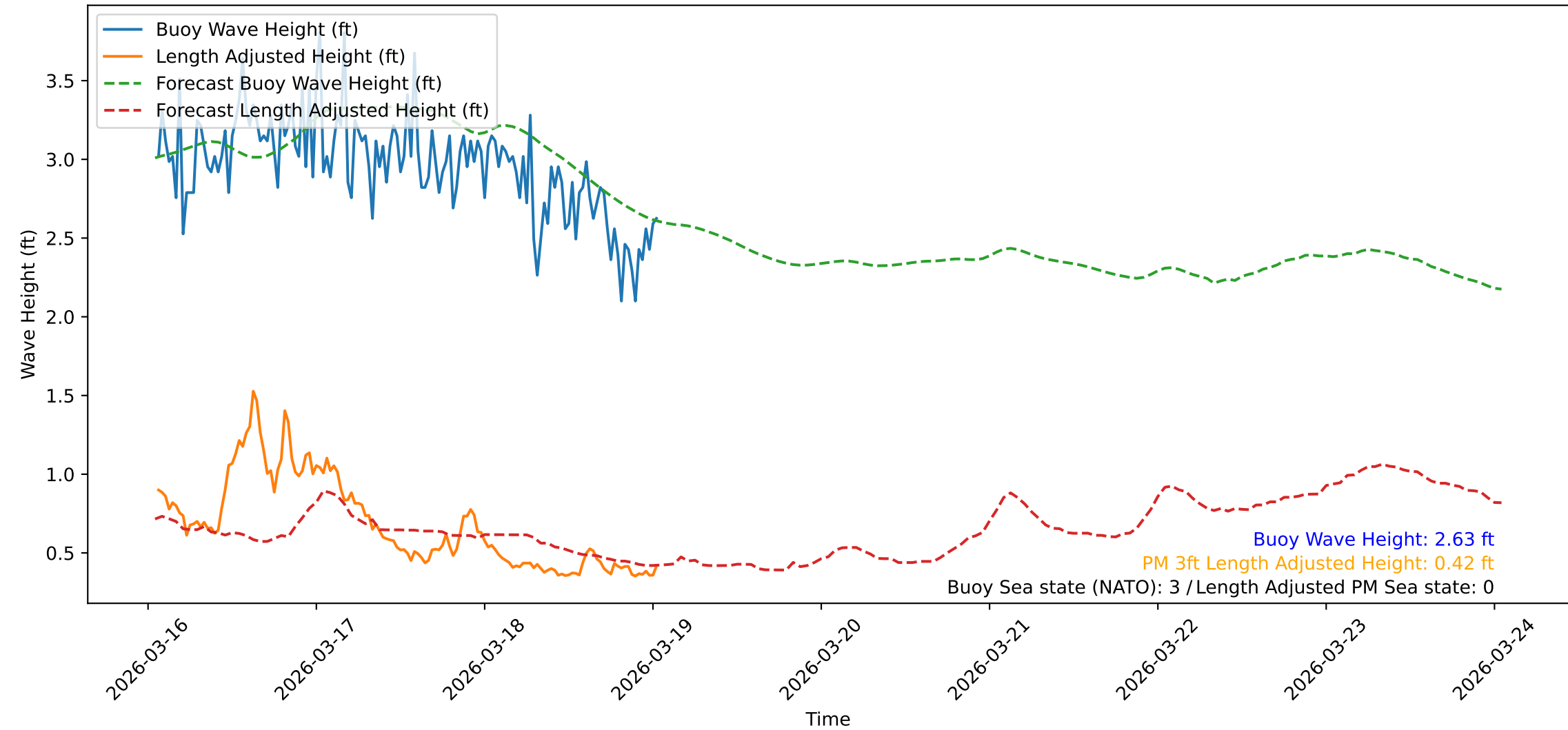
Wave Heights over Time for Red Beach at 2026-03-19 01:10:48
