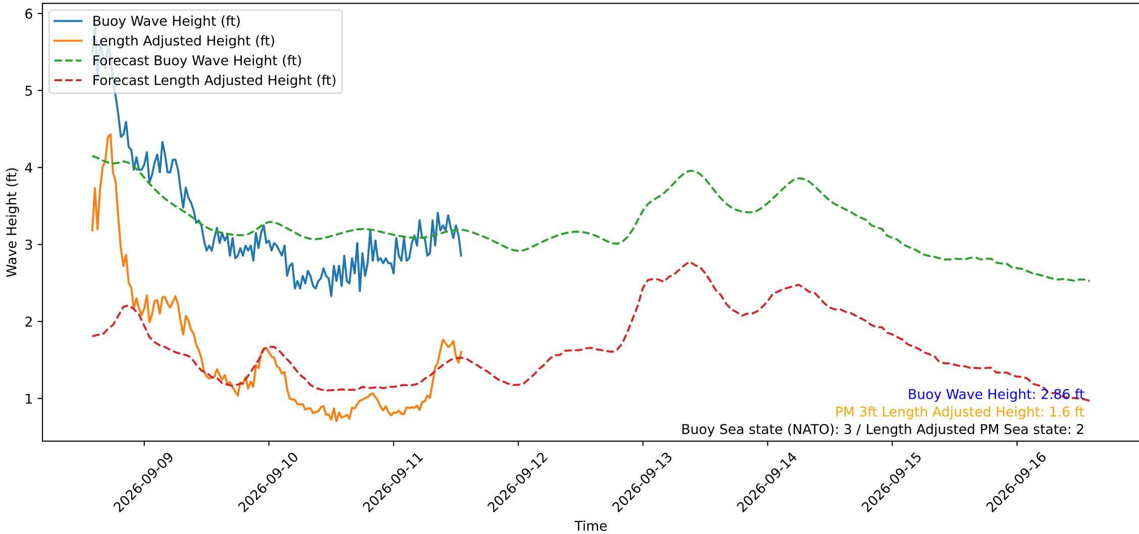
Wave Heights over Time for Red Beach at 2026-09-11 13:50:51
