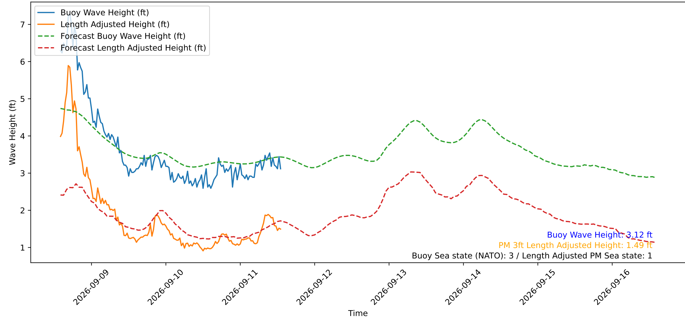
Wave Heights over Time for Green Beach at 2026-09-11 13:51:15
