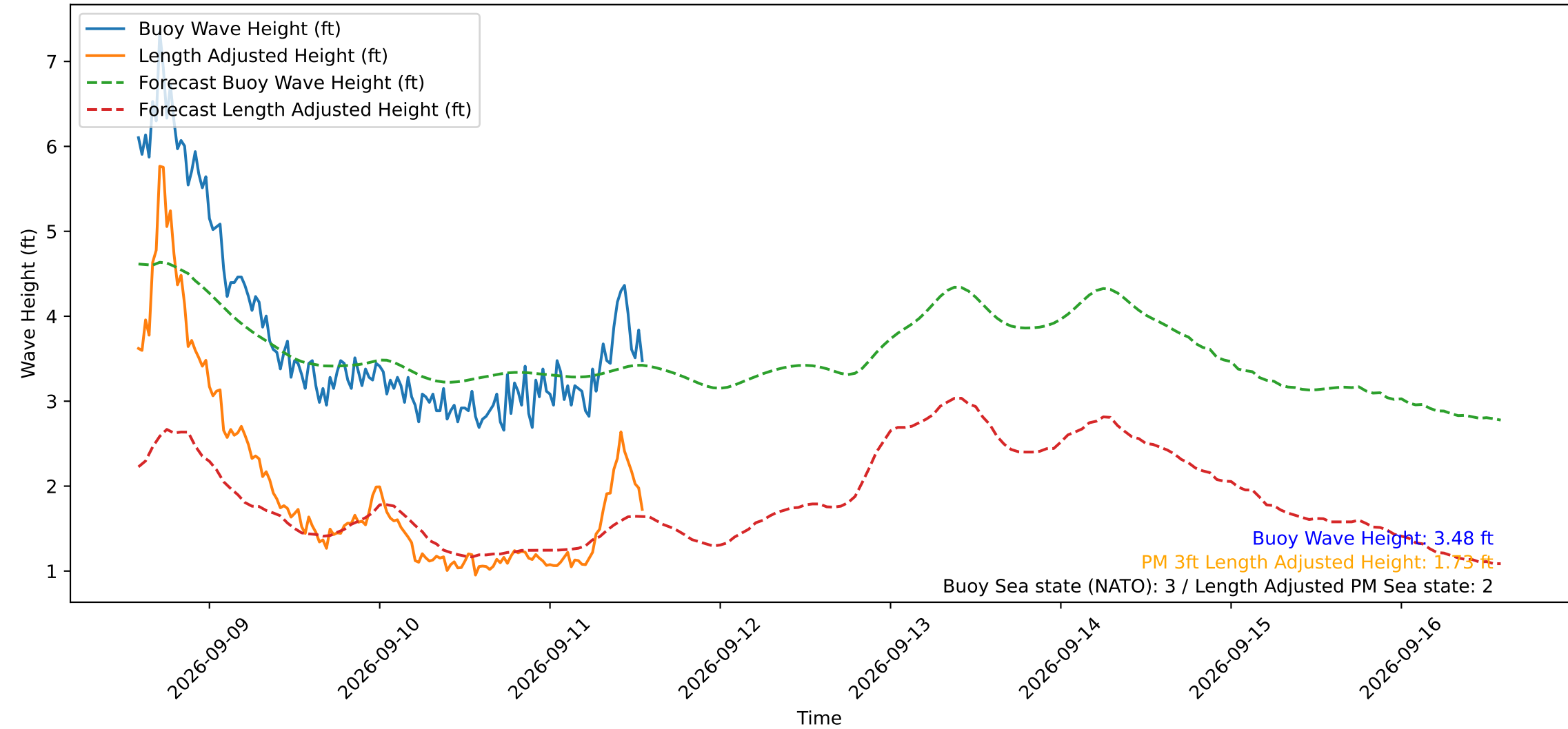
Wave Heights over Time for Oceanside Harbor at 2026-09-11 13:50:30
