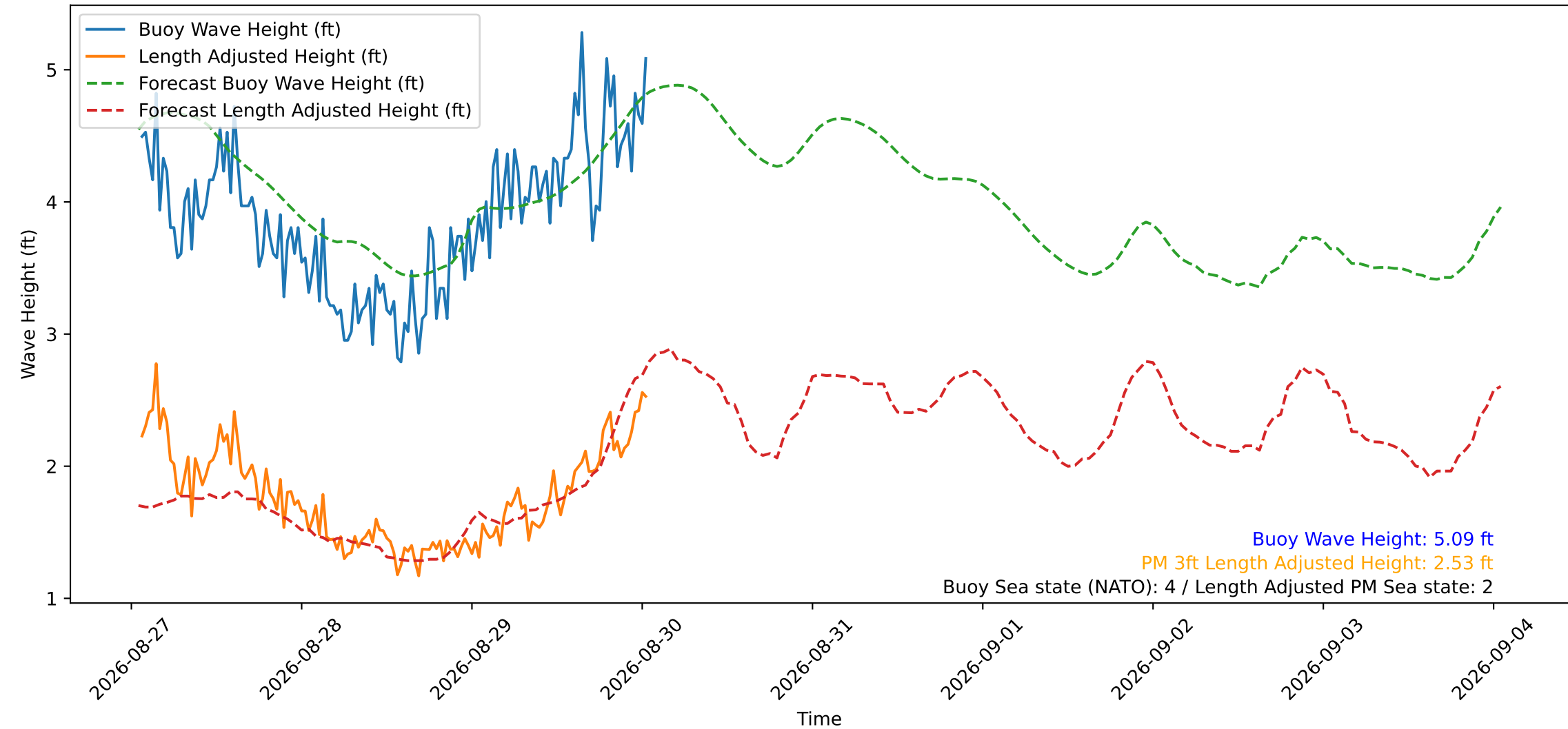
Wave Heights over Time for Oceanside Harbor at 2026-08-30 01:20:29
