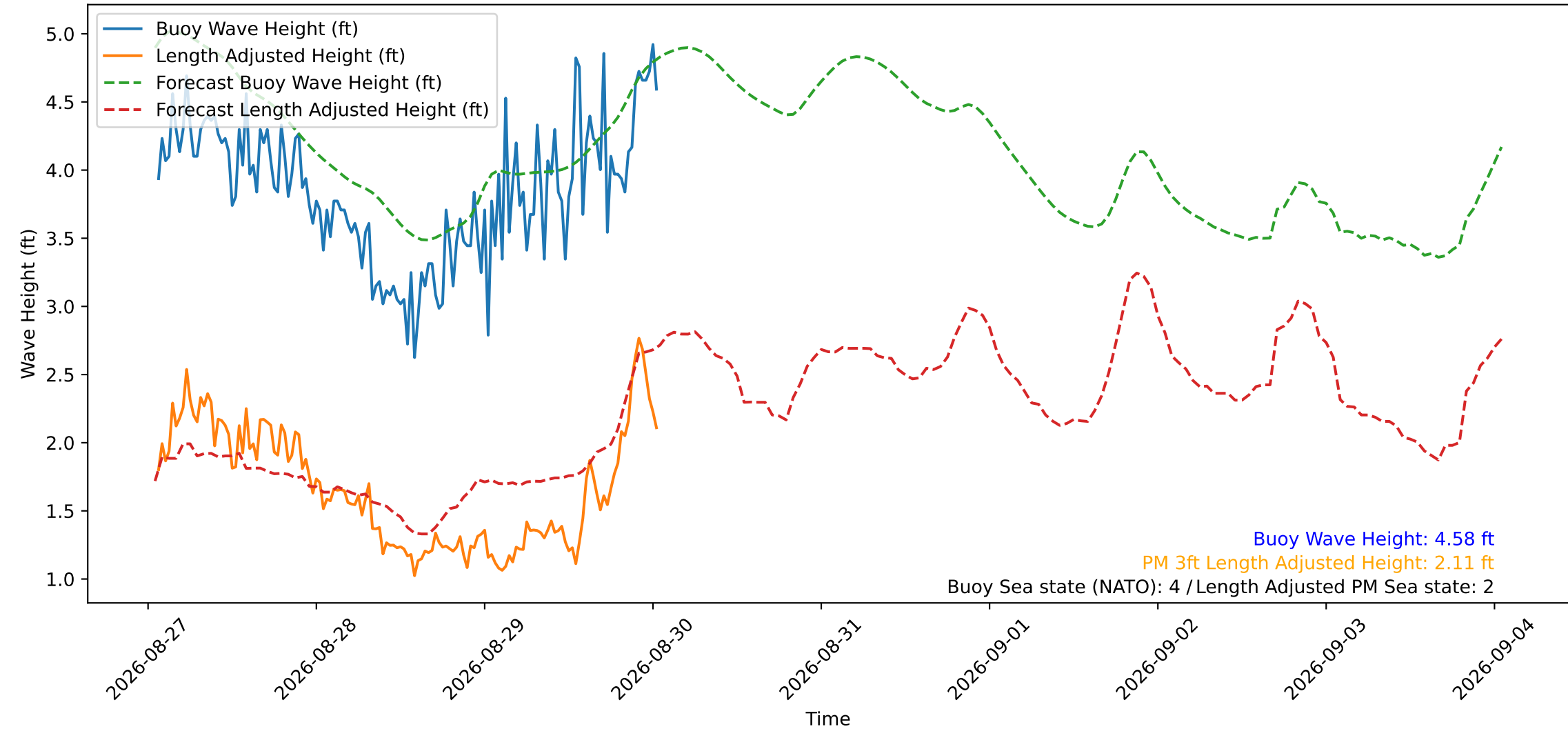
Wave Heights over Time for Green Beach at 2026-08-30 01:21:15
