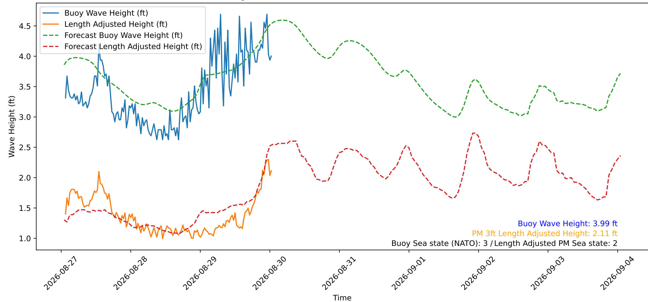
Wave Heights over Time for Red Beach at 2026-08-30 01:20:50
