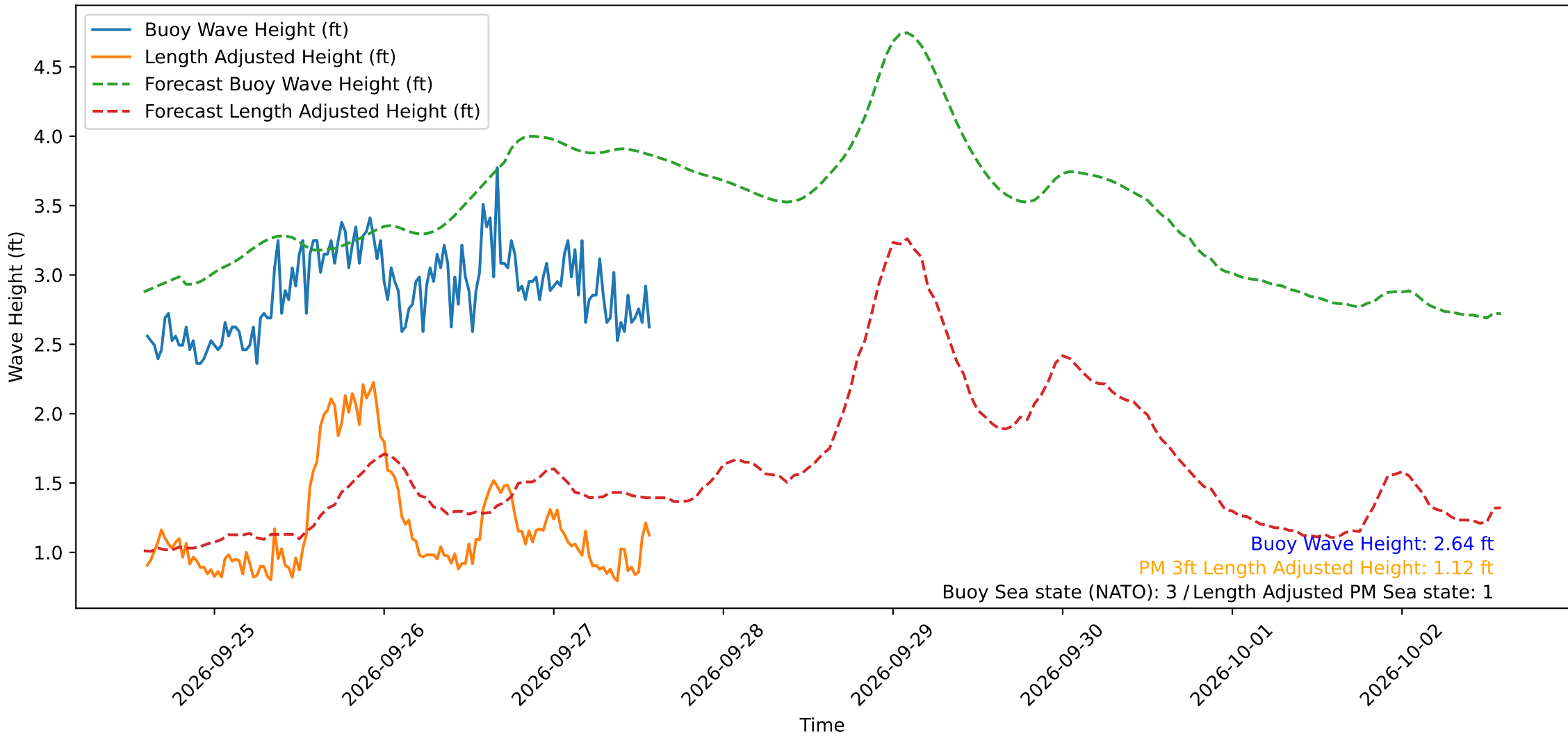
Wave Heights over Time for Oceanside Harbor at 2026-09-27 14:20:30
