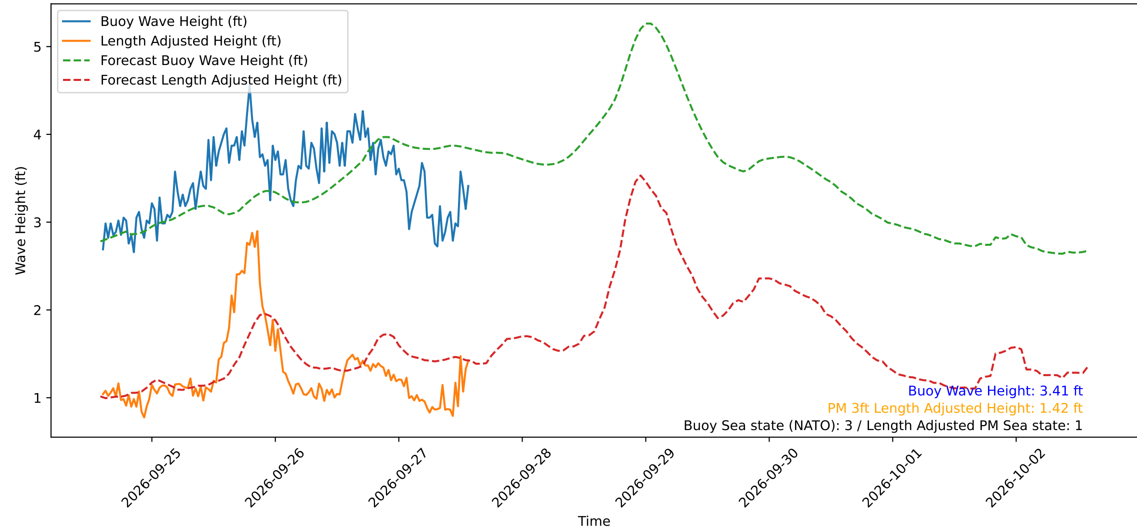
Wave Heights over Time for Green Beach at 2026-09-27 14:21:15
