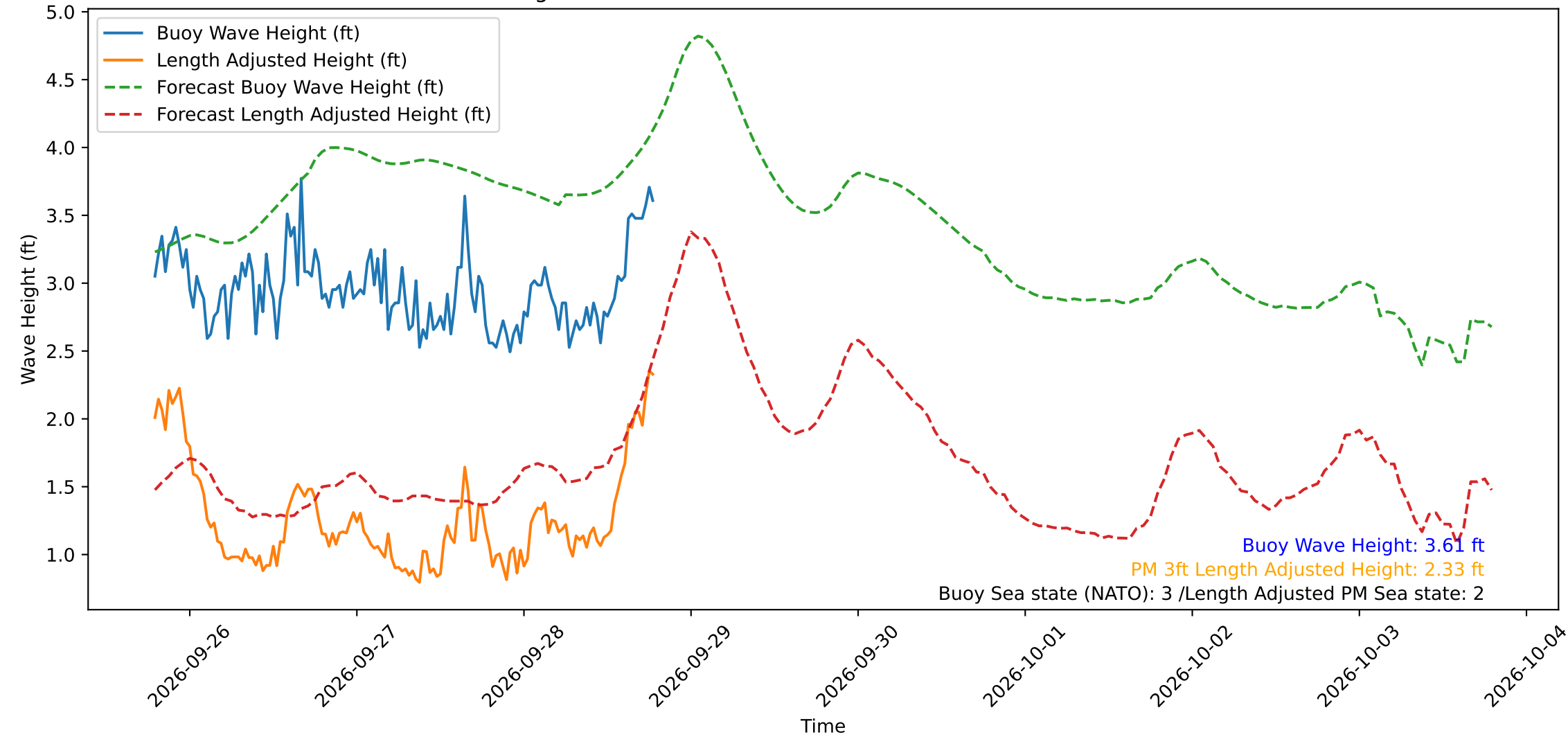
Wave Heights over Time for Oceanside Harbor at 2026-09-28 19:10:30
