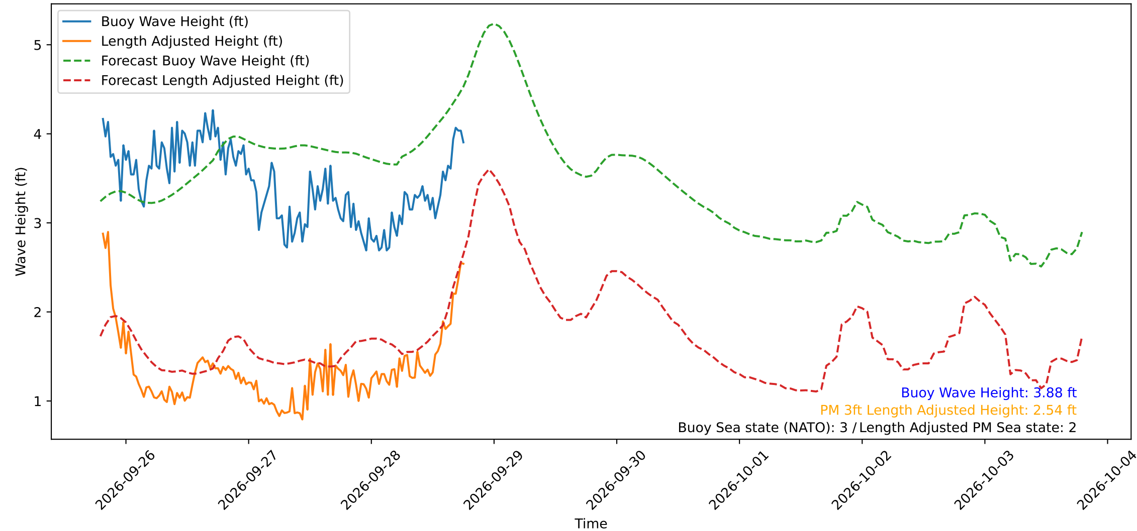
Wave Heights over Time for Green Beach at 2026-09-28 19:11:12
