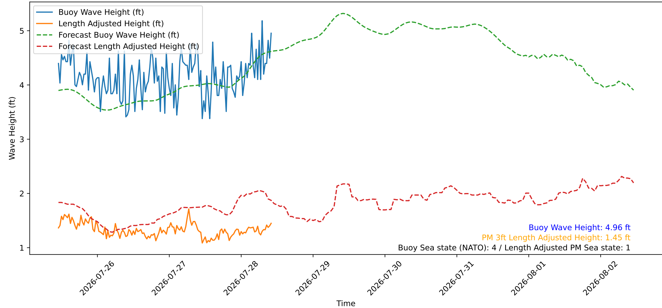
Wave Heights over Time for Green Beach at 2026-07-28 11:01:08
