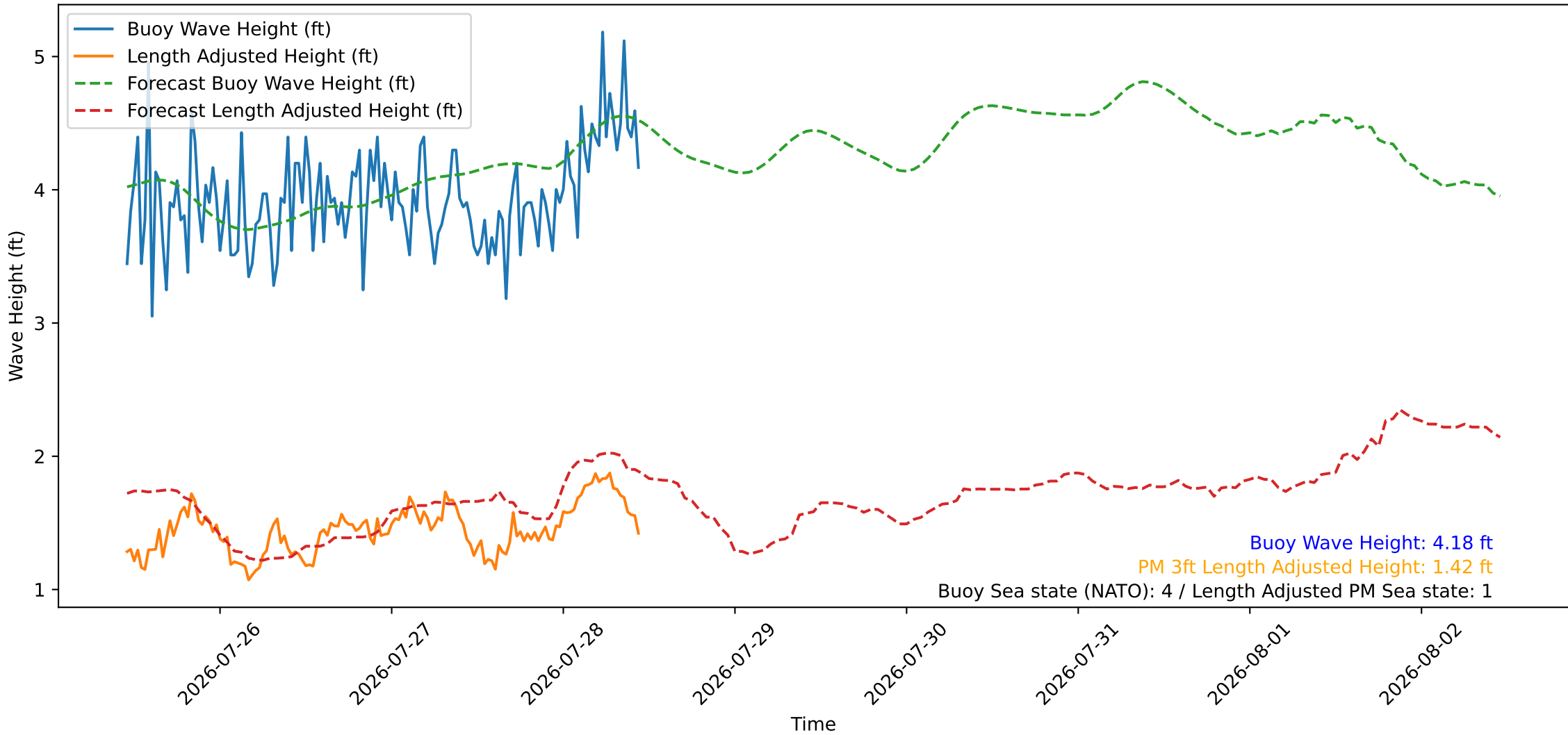
Wave Heights over Time for Oceanside Harbor at 2026-07-28 11:00:26
