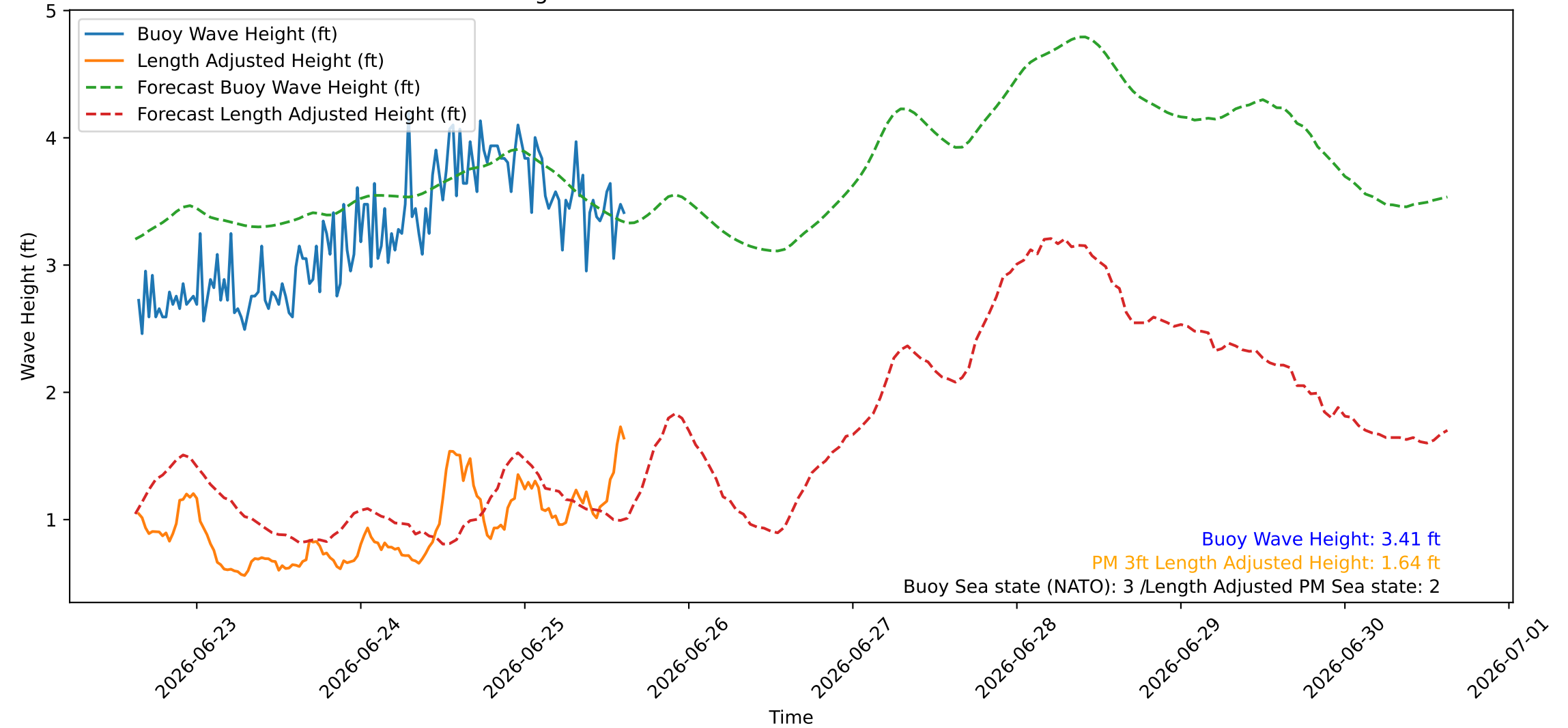
Wave Heights over Time for Green Beach at 2026-06-25 15:21:08
