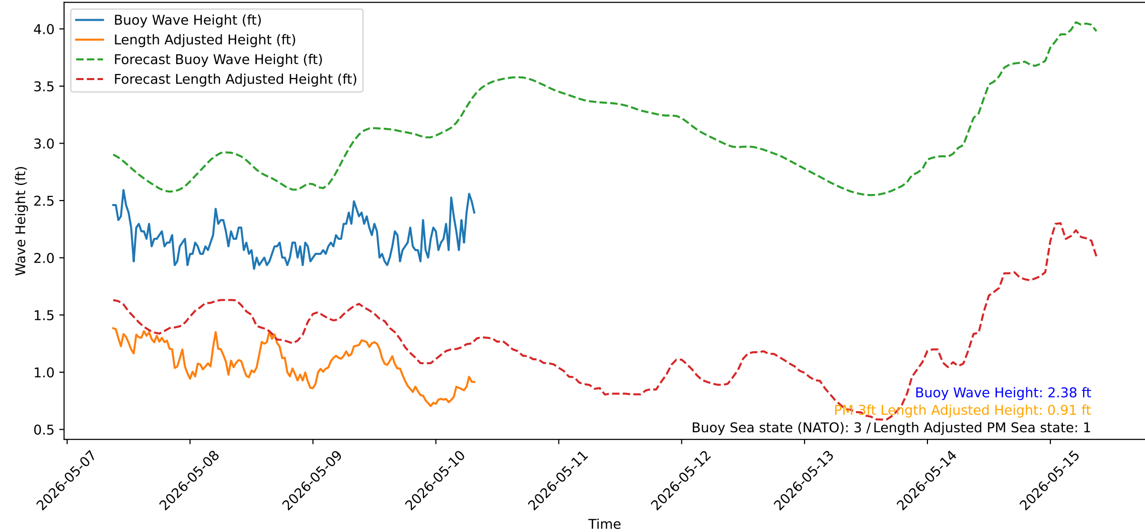
Wave Heights over Time for Red Beach at 2026-05-10 08:40:51
