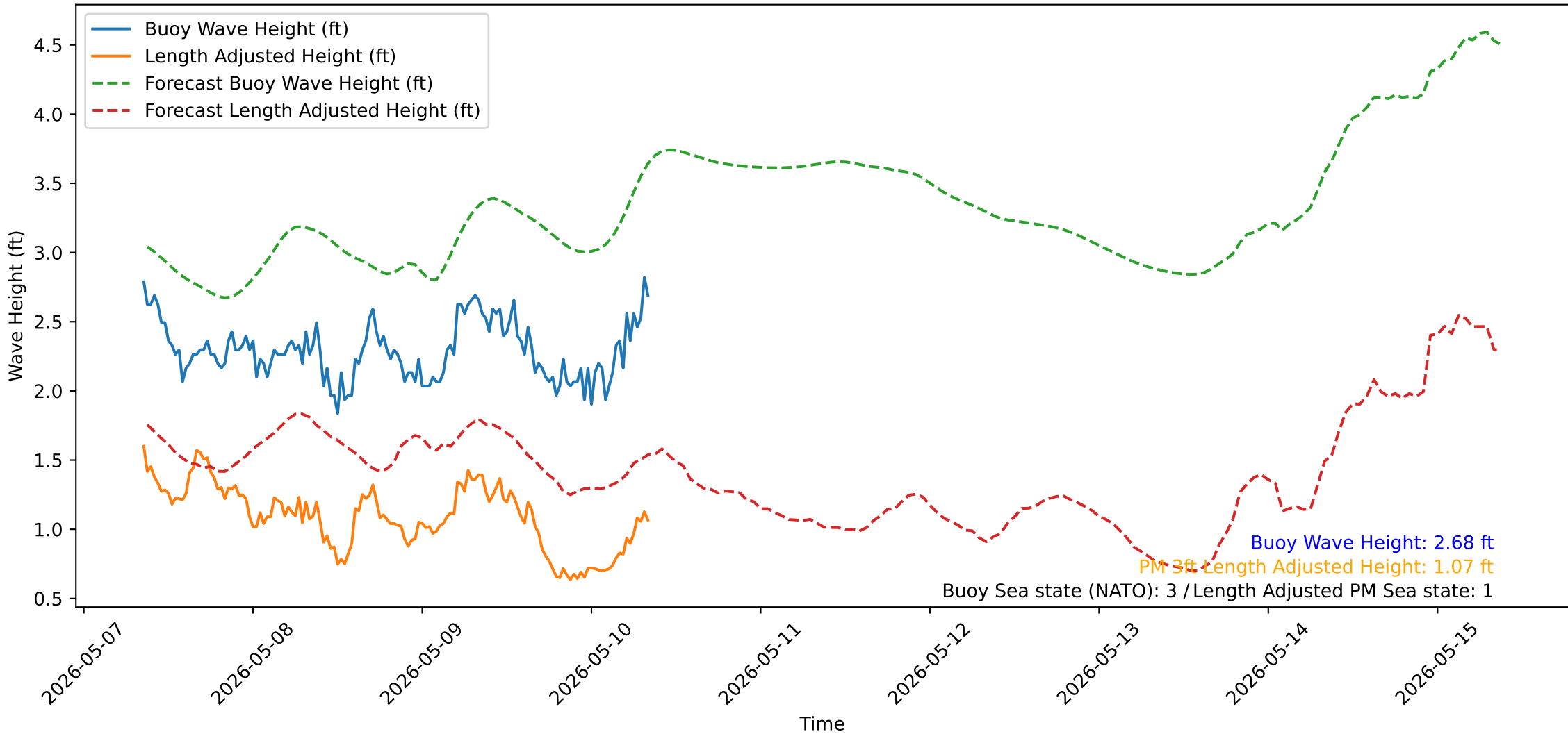
Wave Heights over Time for Green Beach at 2026-05-10 08:41:14
