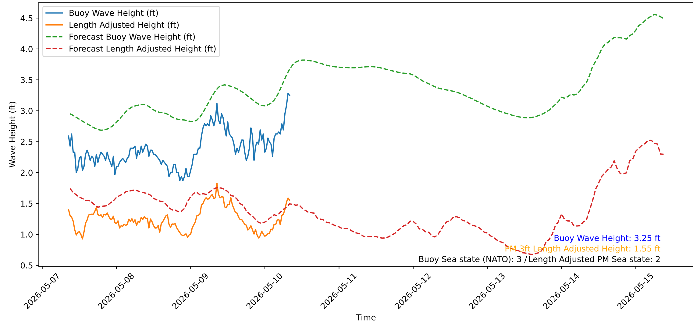
Wave Heights over Time for Oceanside Harbor at 2026-05-10 08:40:32
