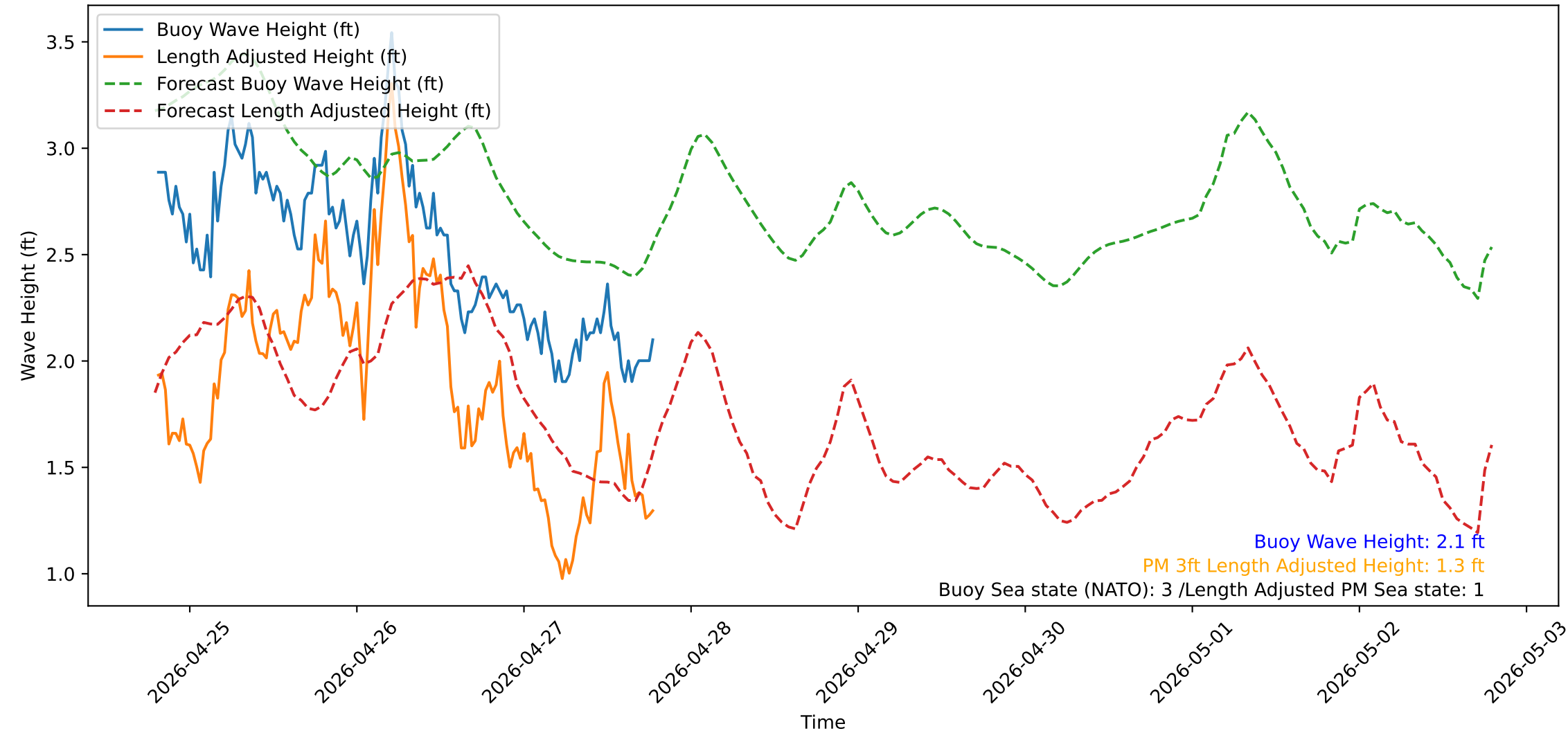
Wave Heights over Time for Red Beach at 2026-04-27 19:20:51
