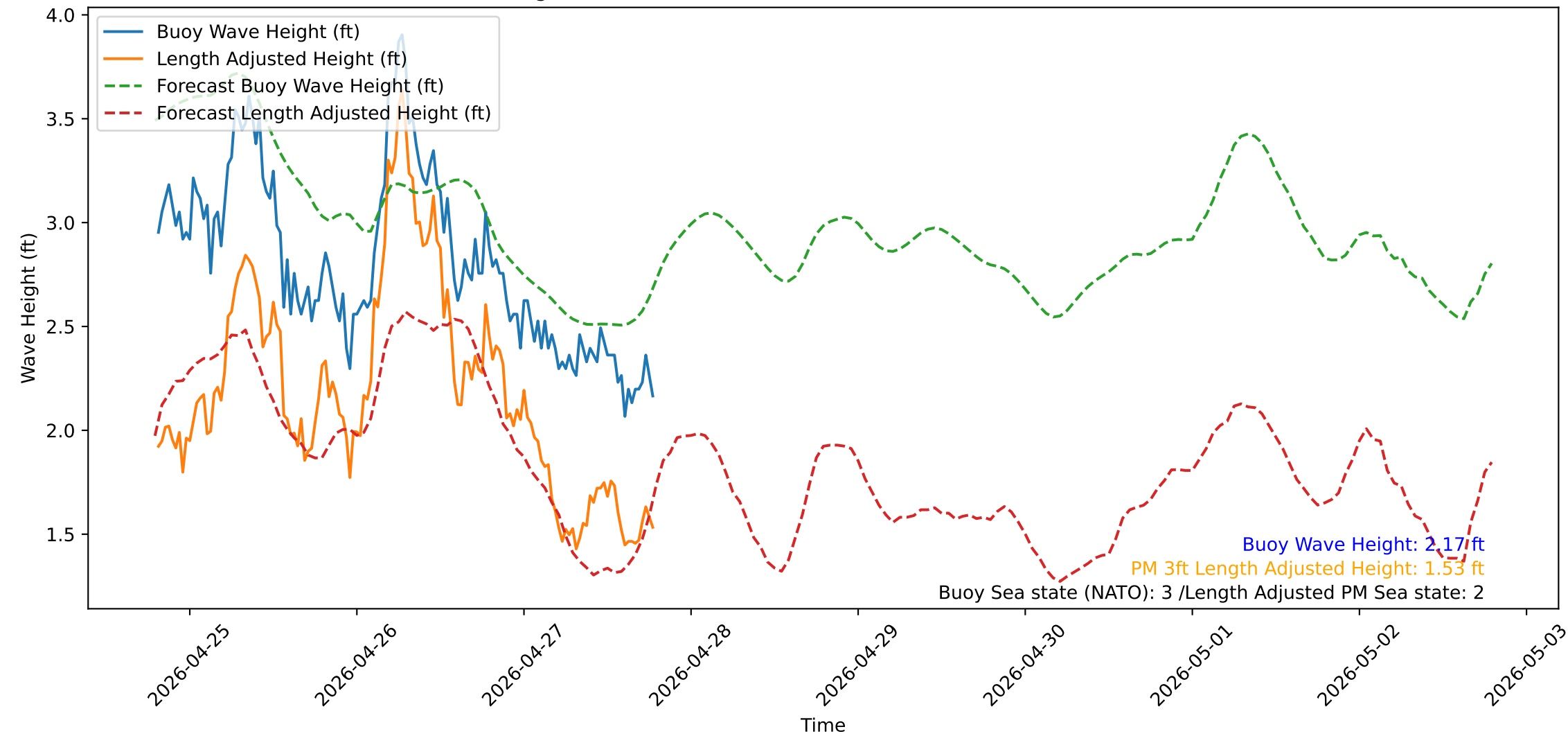
Wave Heights over Time for Oceanside Harbor at 2026-04-27 19:20:31
