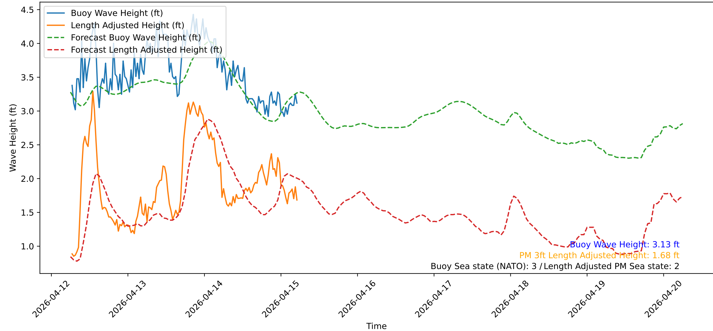
Wave Heights over Time for Red Beach at 2026-04-15 06:00:51
