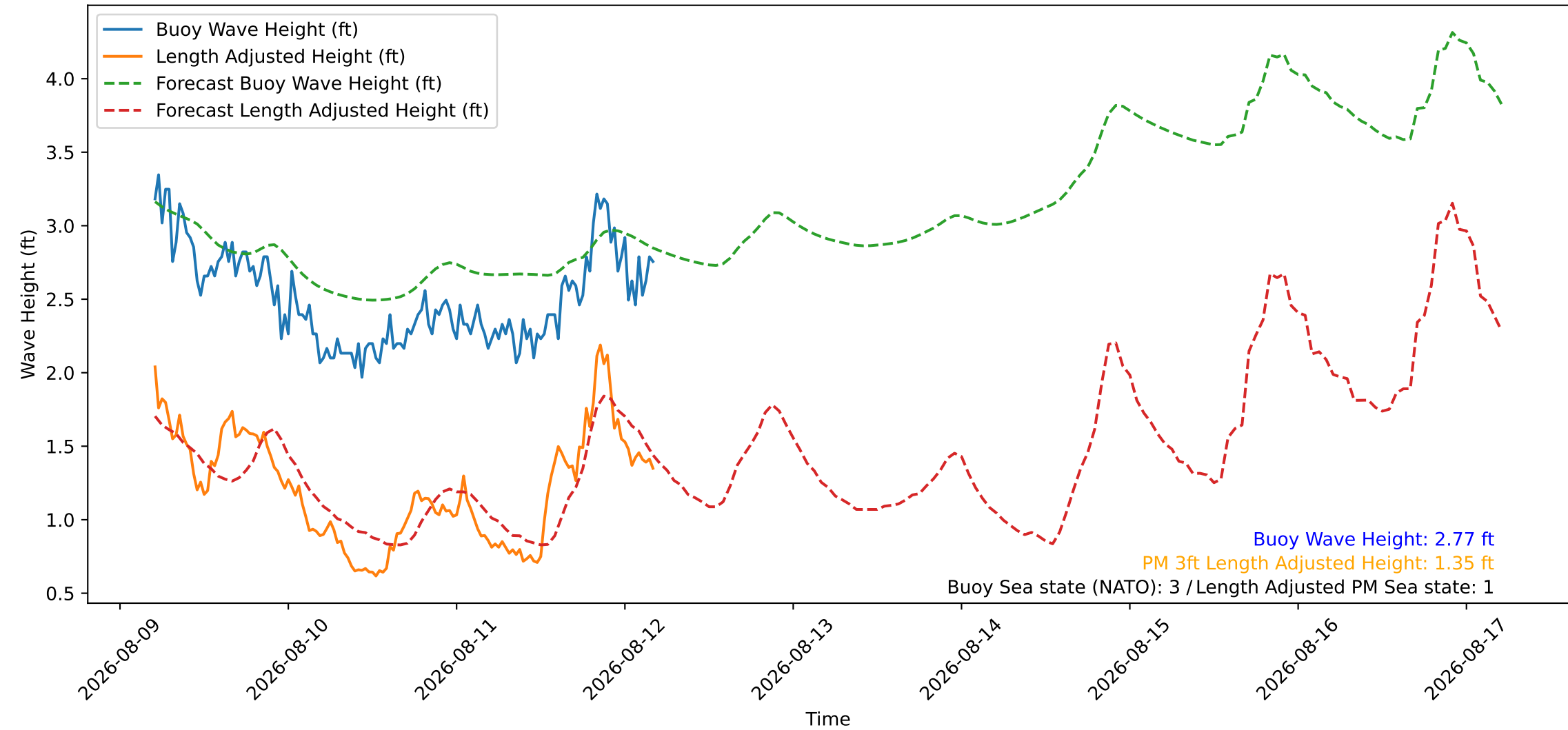
Wave Heights over Time for Green Beach at 2026-08-12 04:51:08
