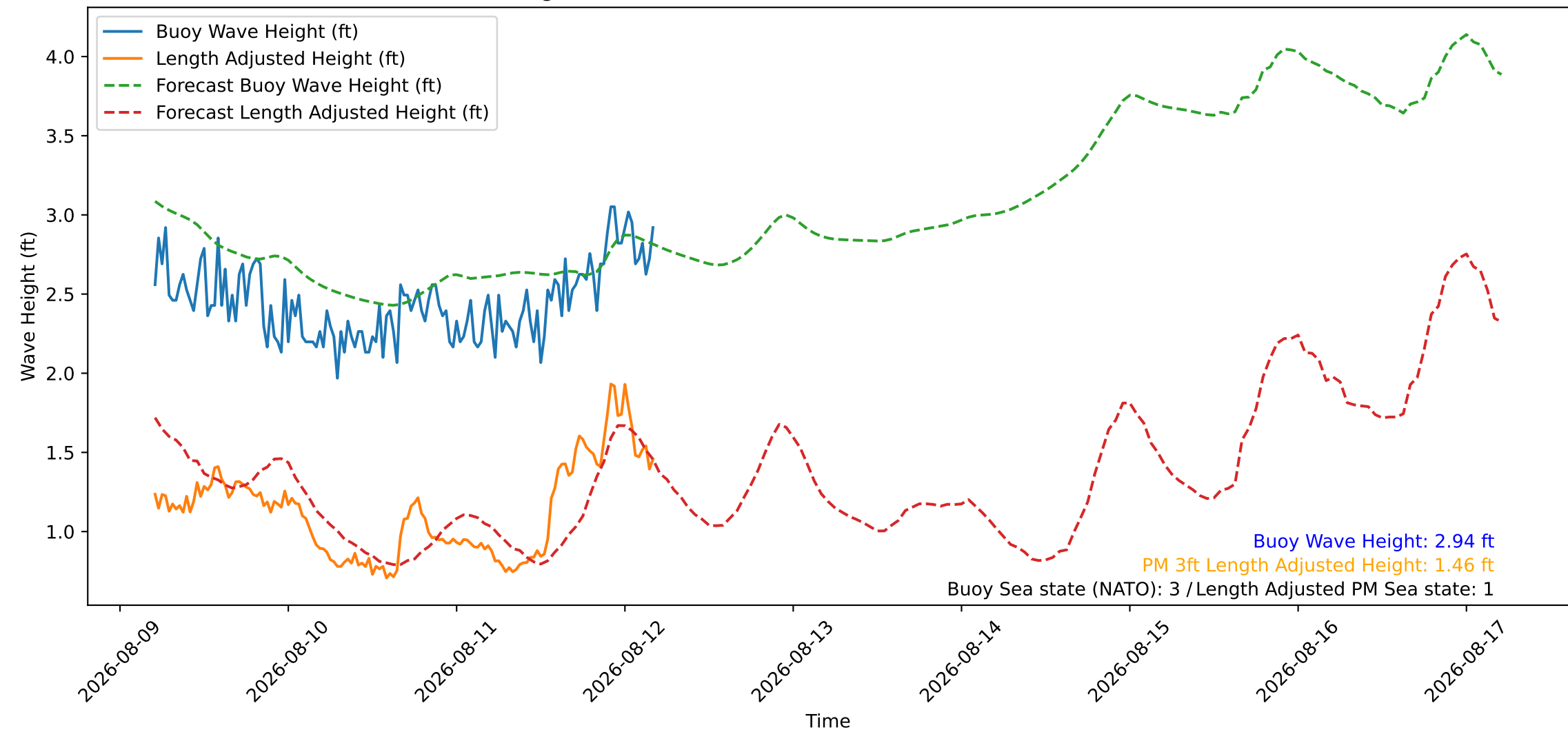
Wave Heights over Time for Oceanside Harbor at 2026-08-12 04:50:26
