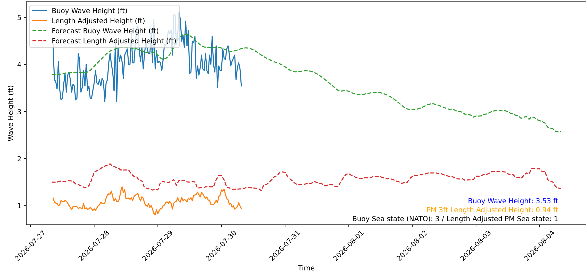
Wave Heights over Time for Red Beach at 2026-07-30 08:20:48
