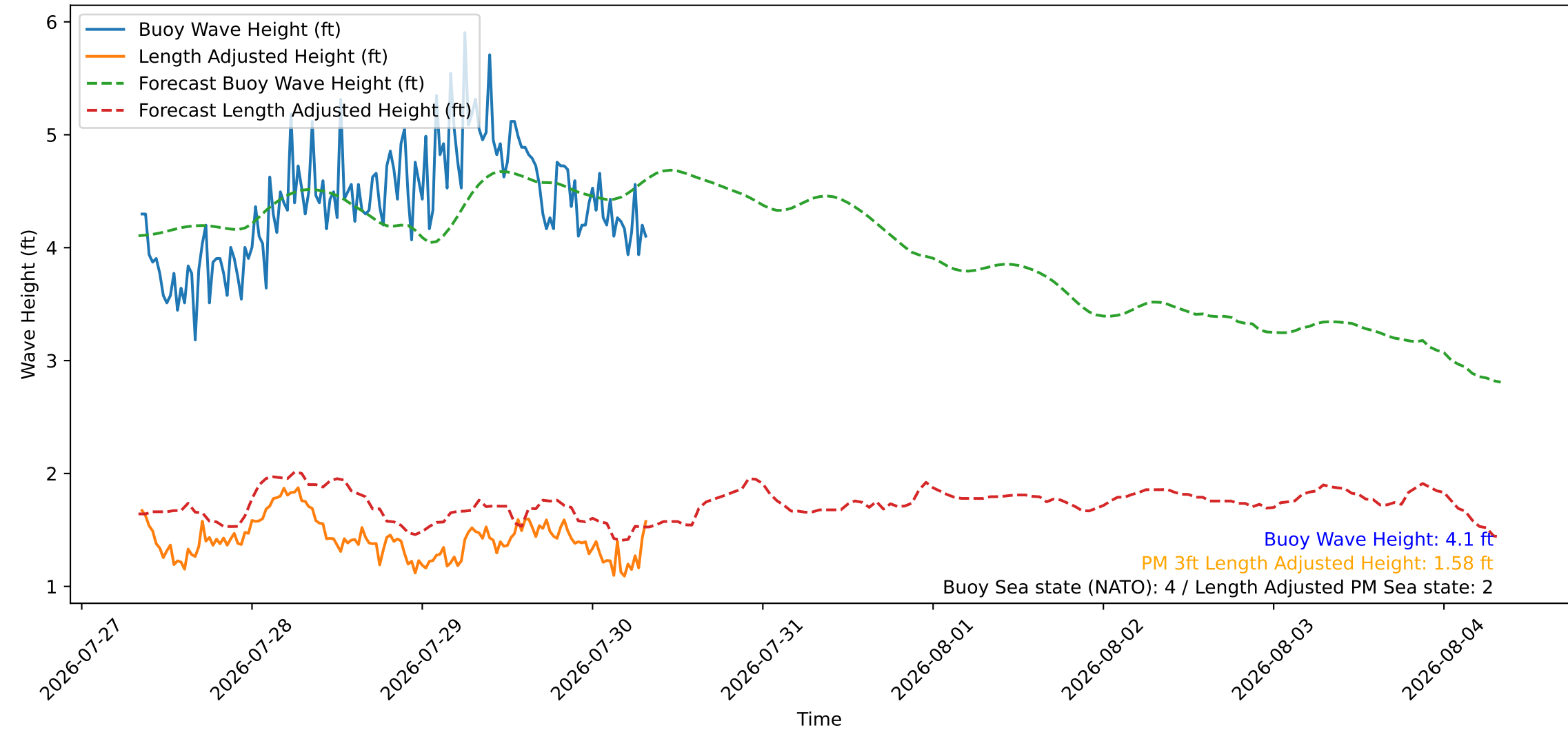
Wave Heights over Time for Oceanside Harbor at 2026-07-30 08:20:26
