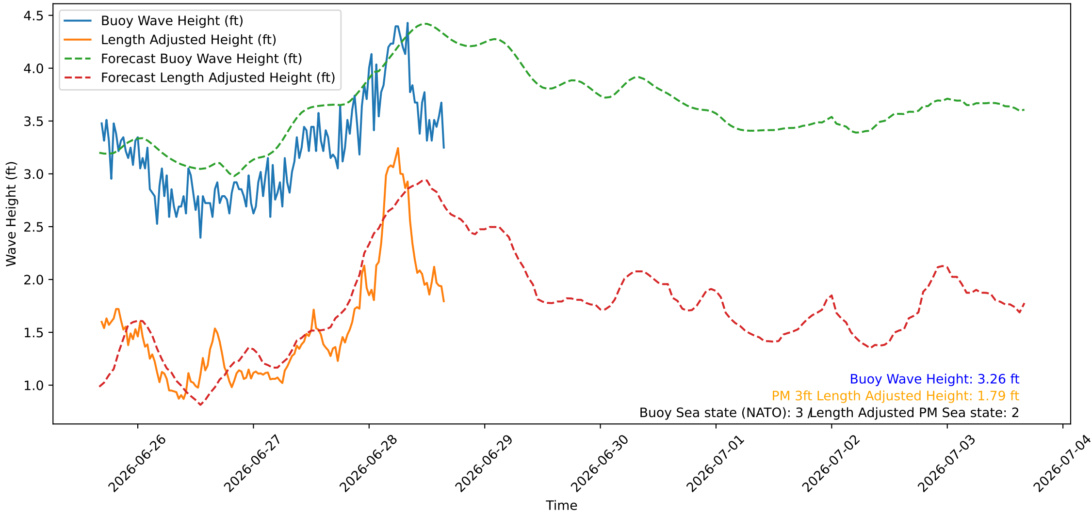
Wave Heights over Time for Oceanside Harbor at 2026-06-28 16:20:26
