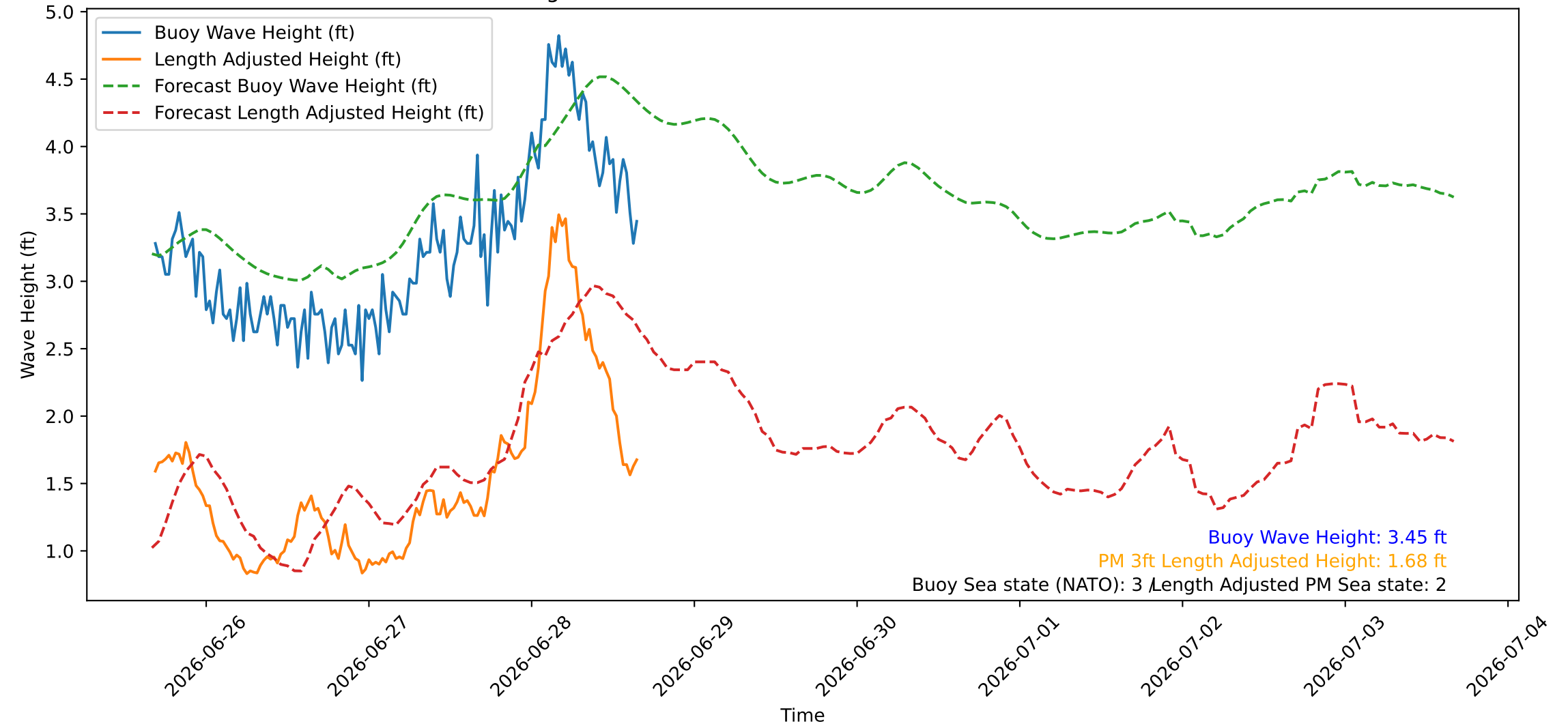
Wave Heights over Time for Green Beach at 2026-06-28 16:21:08
