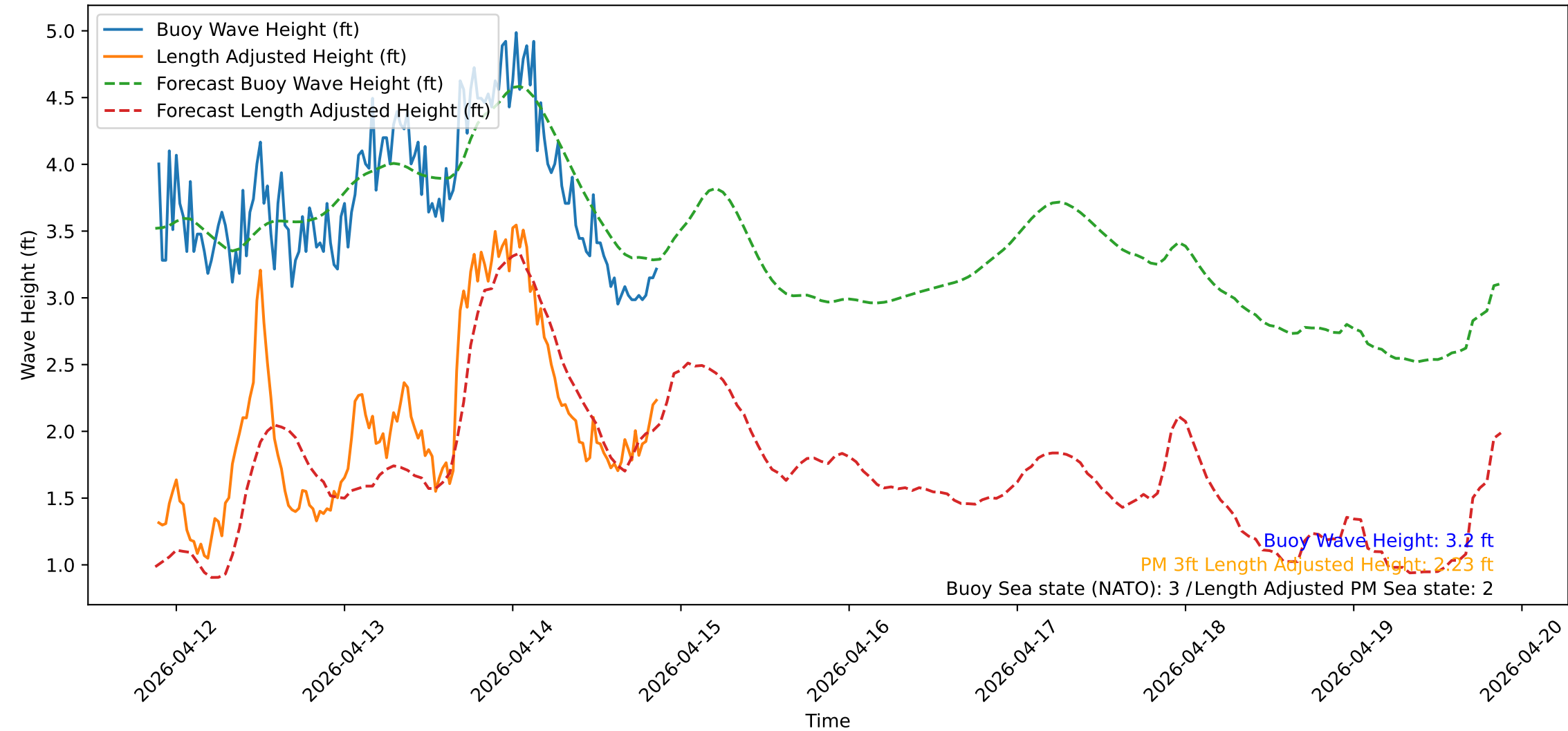
Wave Heights over Time for Green Beach at 2026-04-14 21:21:14
