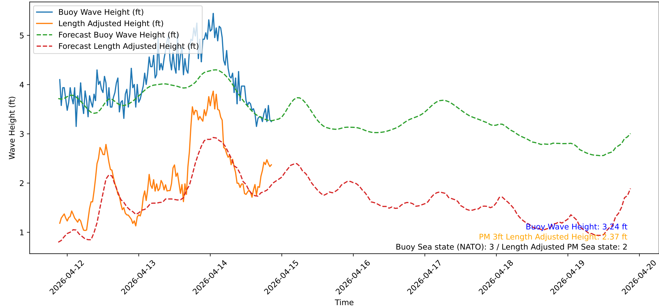
Wave Heights over Time for Oceanside Harbor at 2026-04-14 21:20:31
