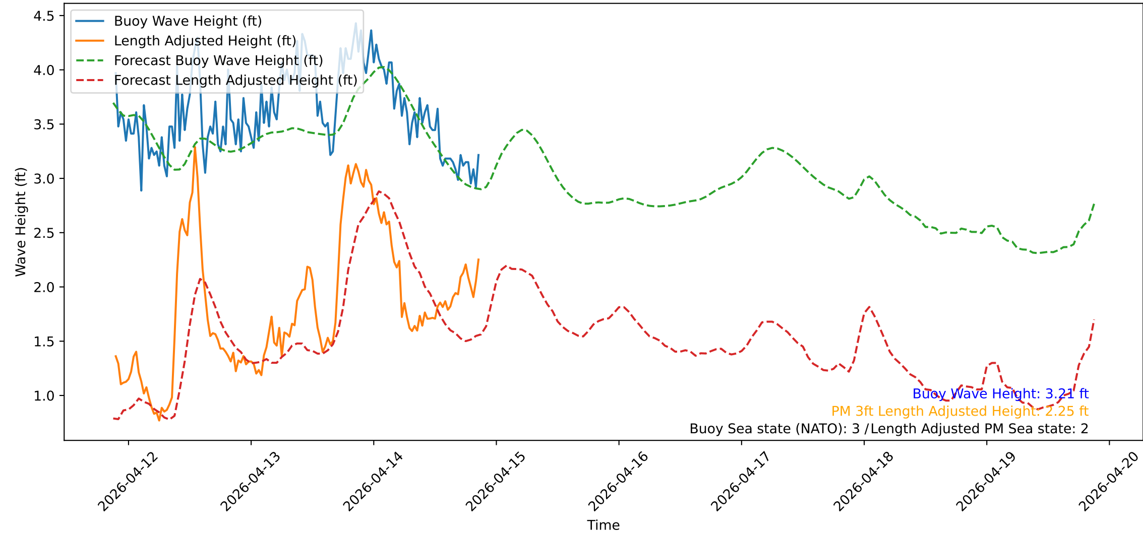
Wave Heights over Time for Red Beach at 2026-04-14 21:20:52
