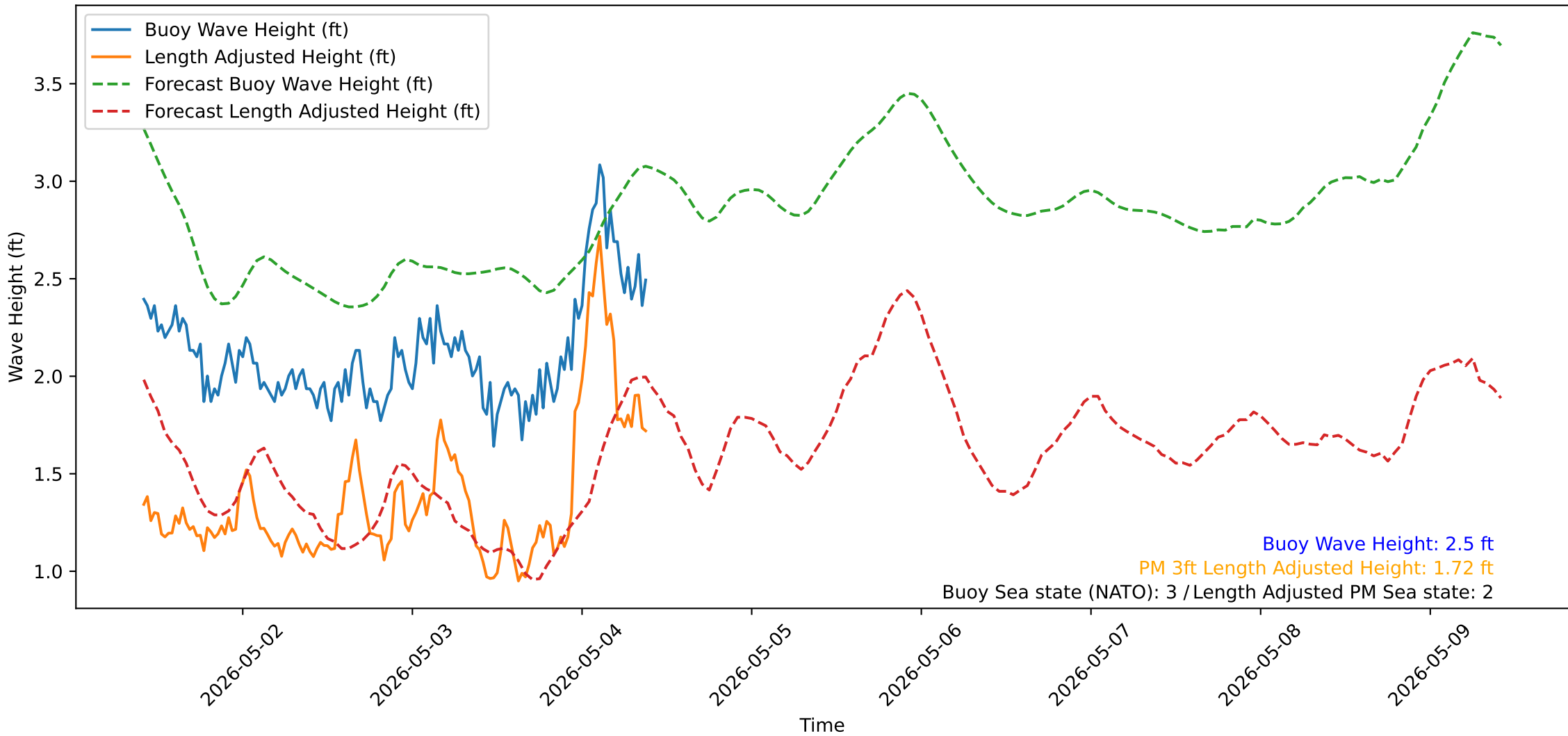
Wave Heights over Time for Oceanside Harbor at 2026-05-04 09:50:31
