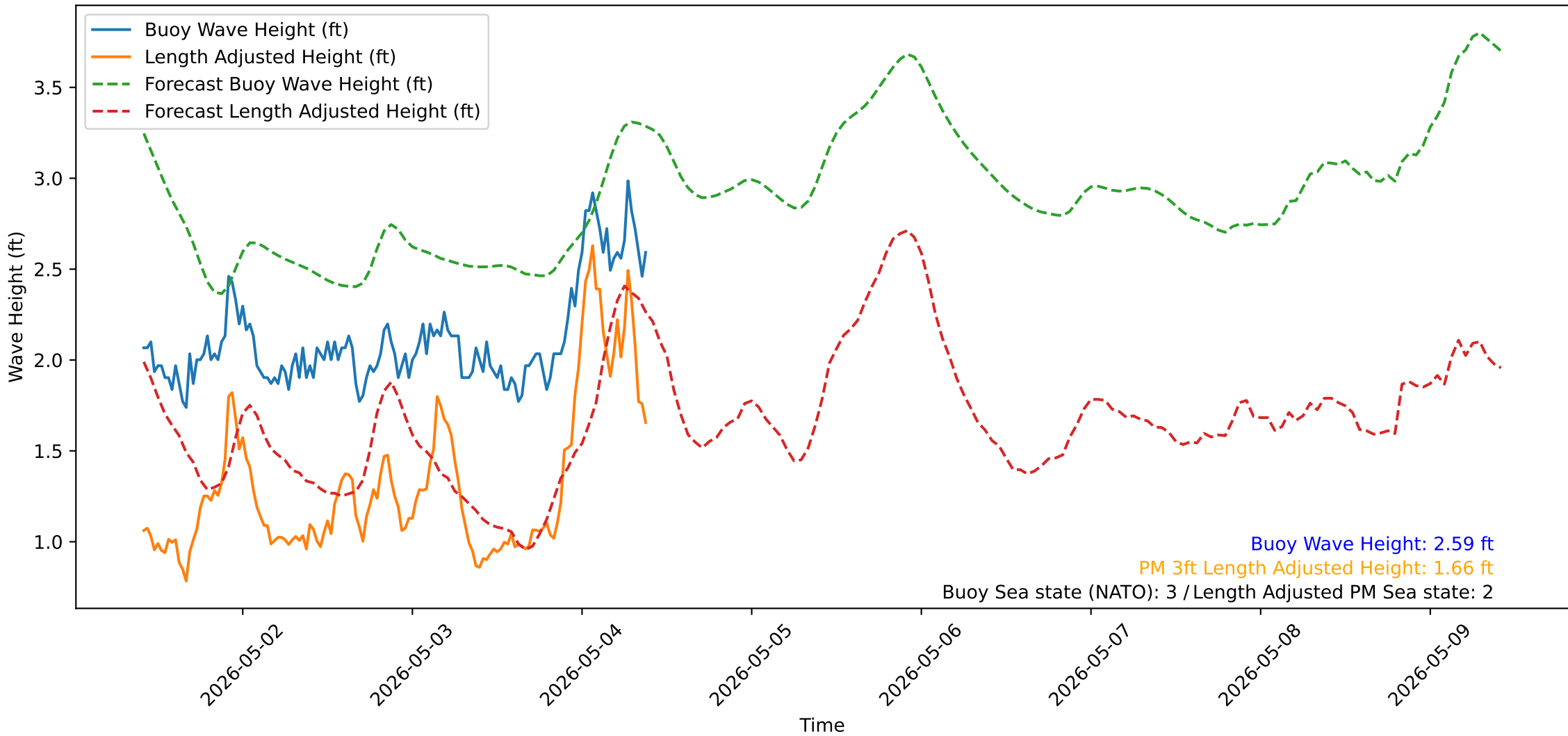
Wave Heights over Time for Green Beach at 2026-05-04 09:51:15
