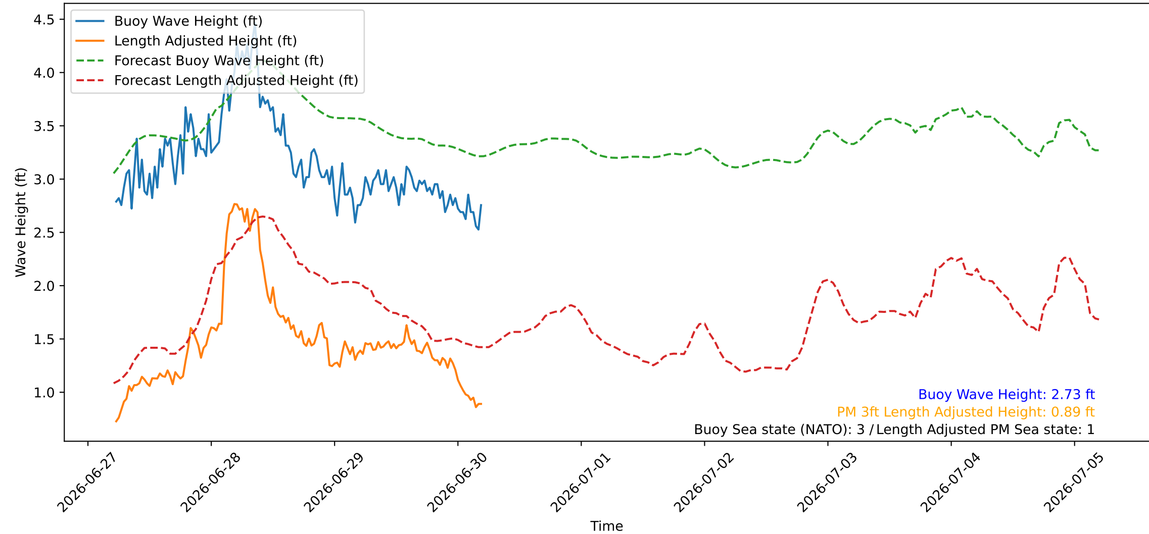
Wave Heights over Time for Red Beach at 2026-06-30 05:10:45
