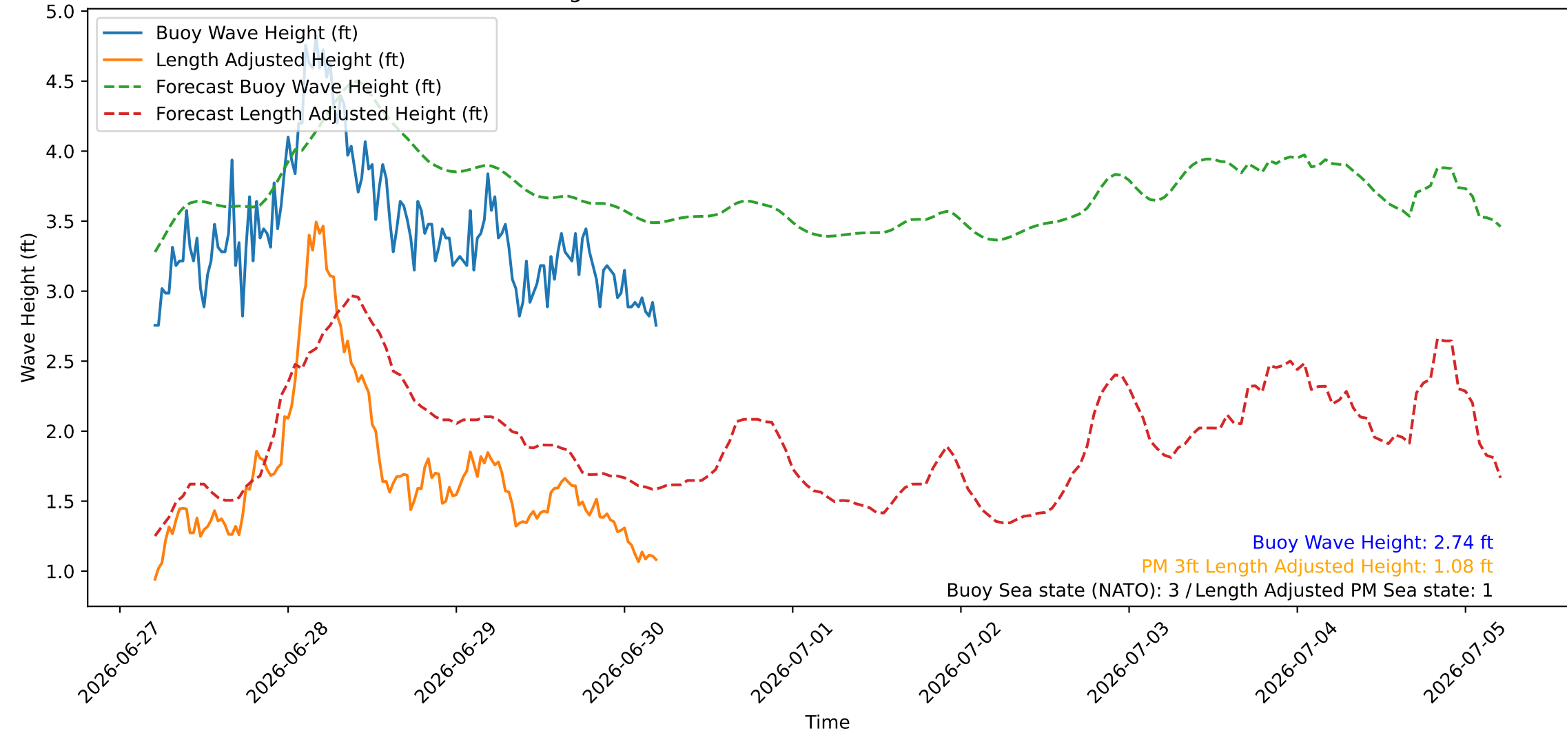
Wave Heights over Time for Green Beach at 2026-06-30 05:11:08
