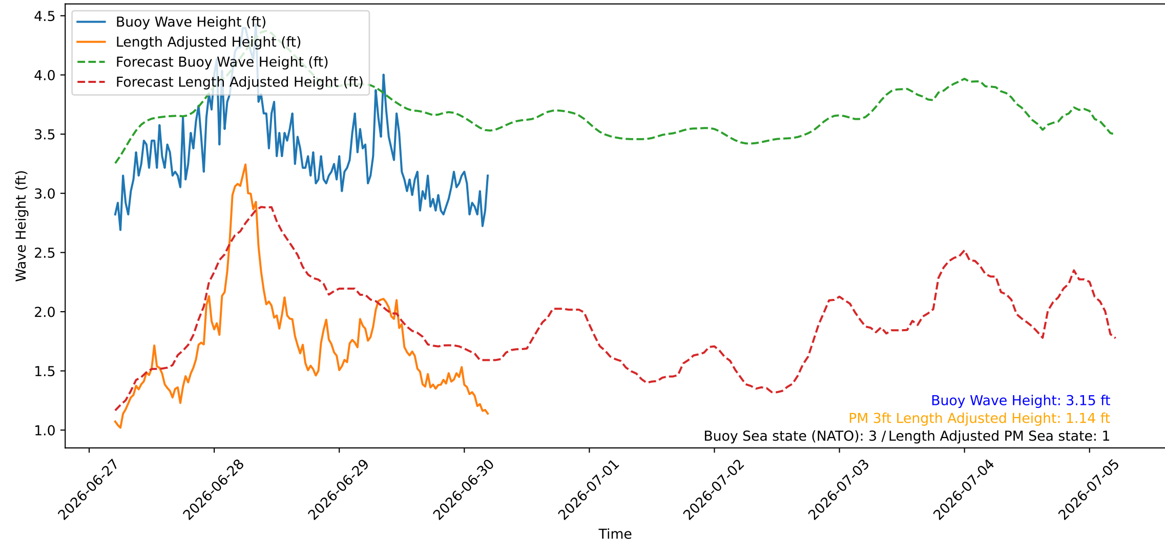
Wave Heights over Time for Oceanside Harbor at 2026-06-30 05:10:26
