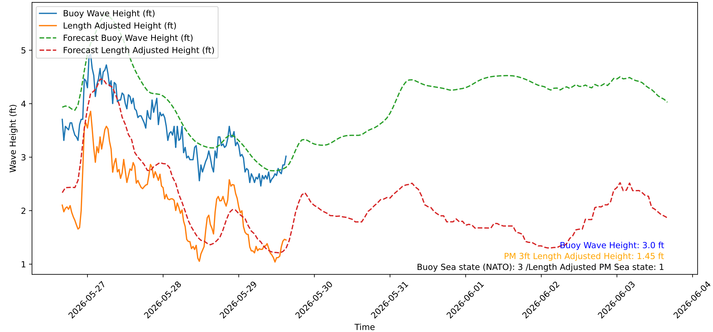
Wave Heights over Time for Green Beach at 2026-05-29 15:51:06
