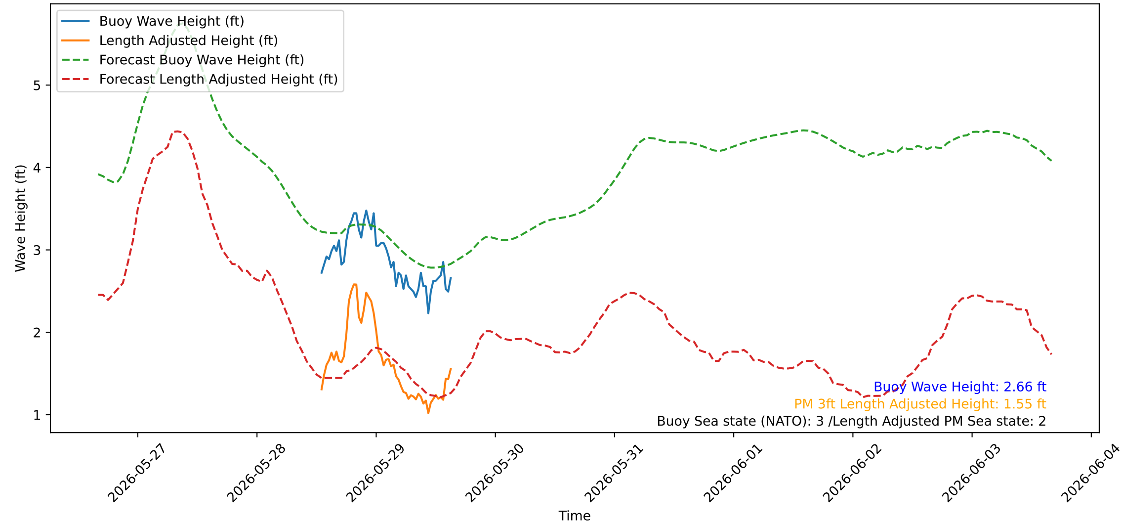
Wave Heights over Time for Oceanside Harbor at 2026-05-29 15:50:22
