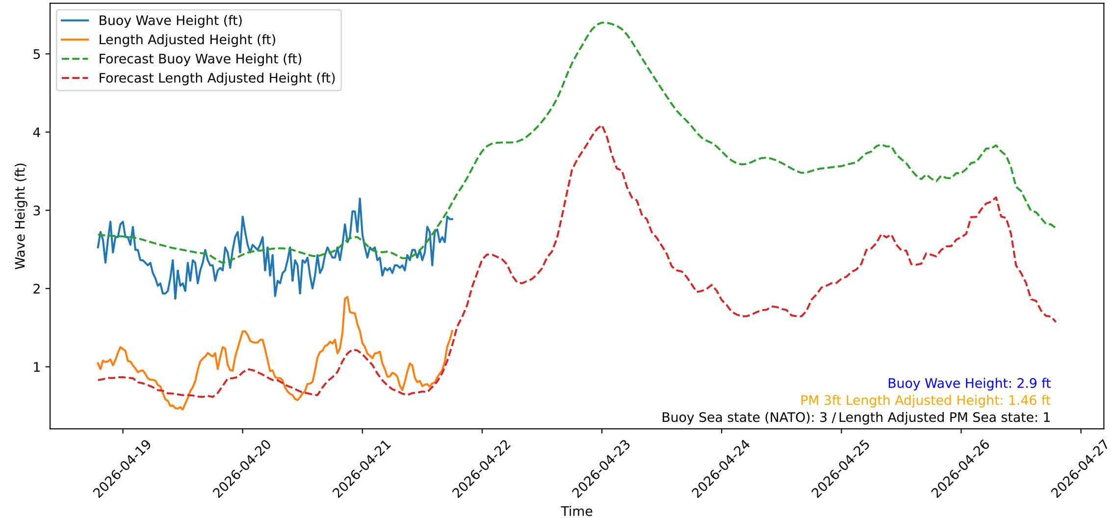
Wave Heights over Time for Green Beach at 2026-04-21 19:01:14
