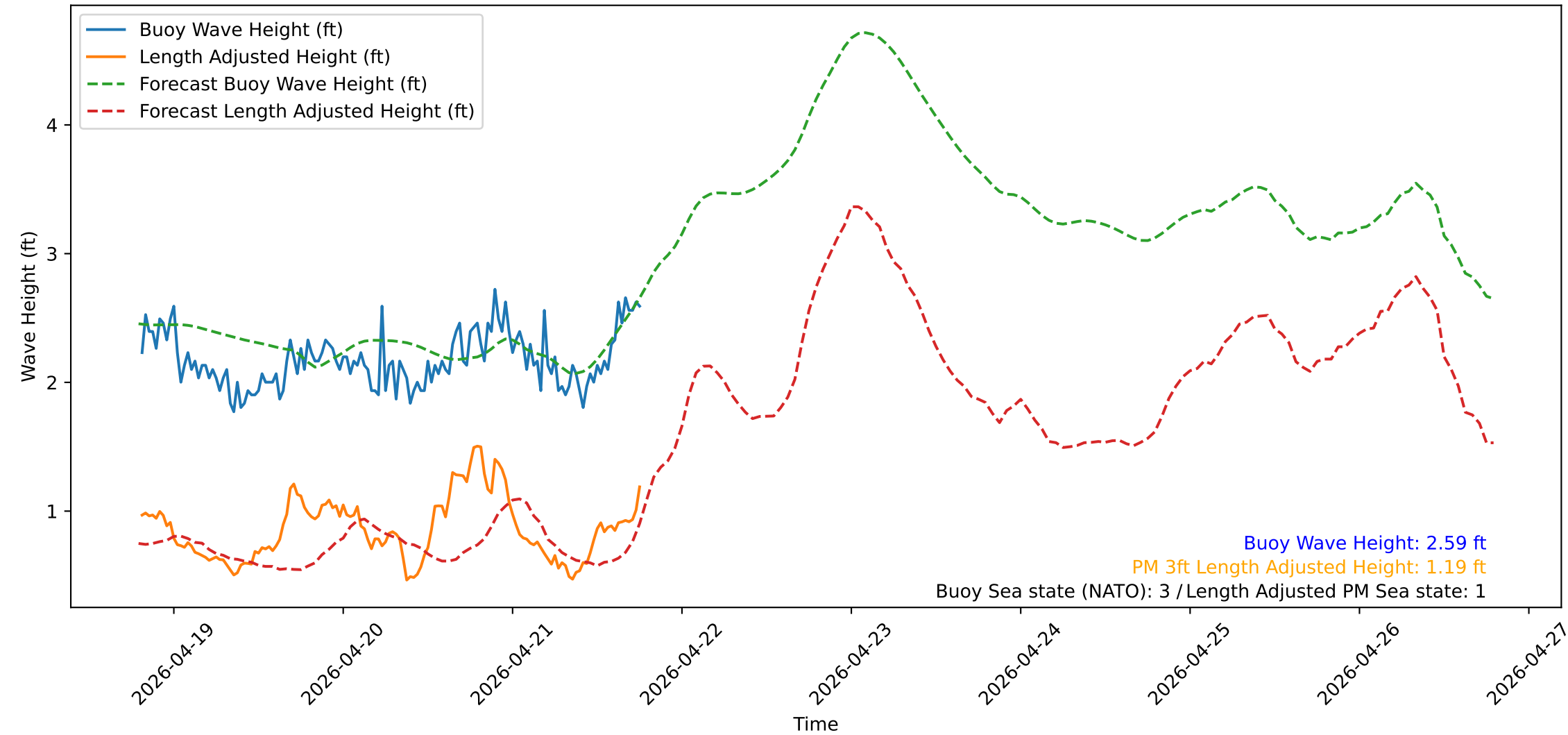
Wave Heights over Time for Red Beach at 2026-04-21 19:00:51
