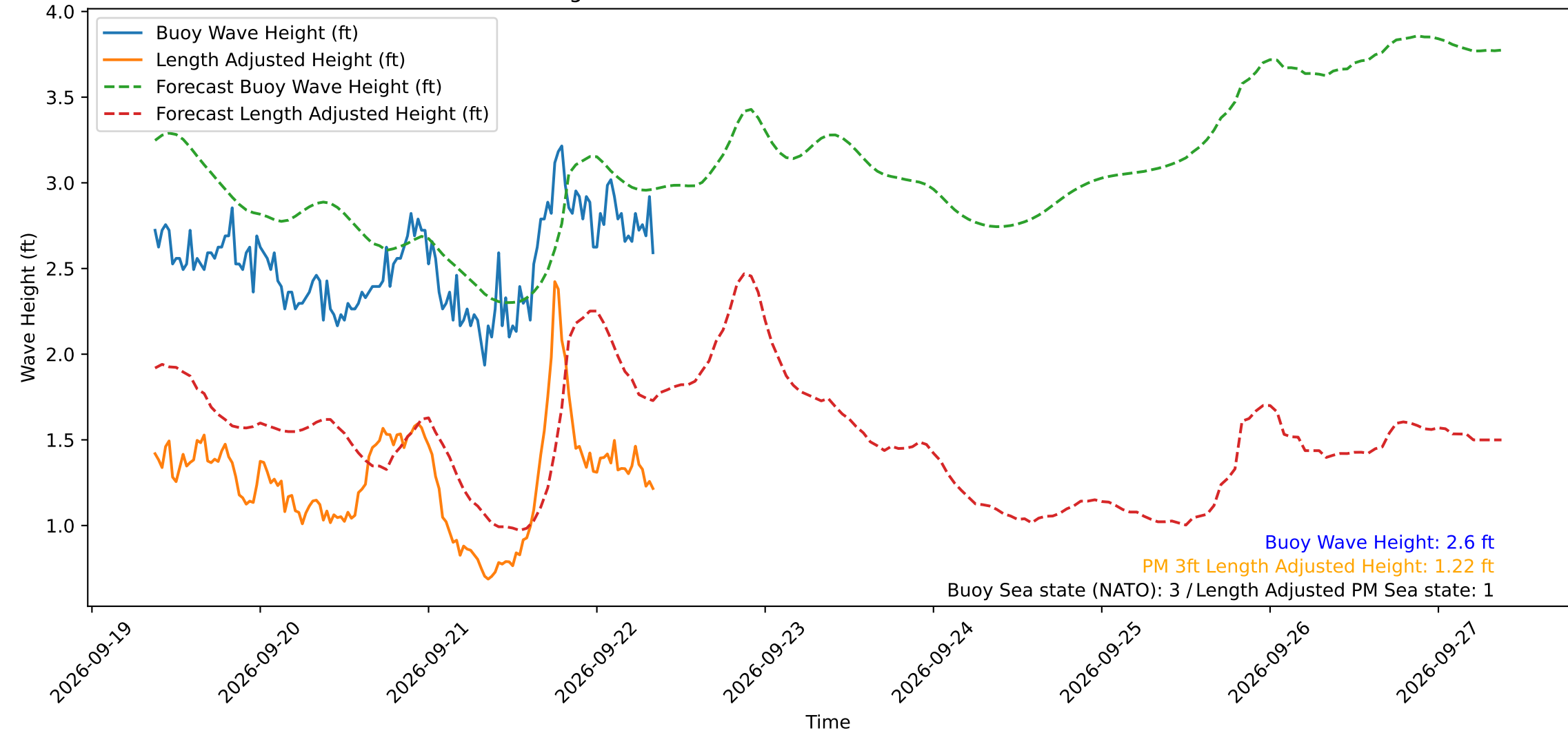
Wave Heights over Time for Green Beach at 2026-09-22 08:41:11
