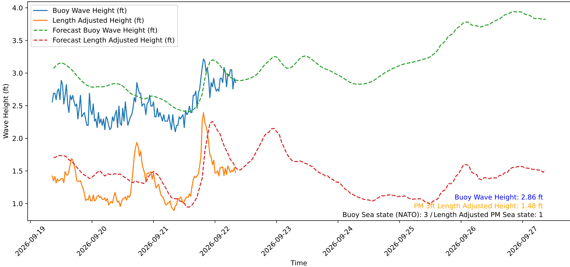
Wave Heights over Time for Oceanside Harbor at 2026-09-22 08:40:30
