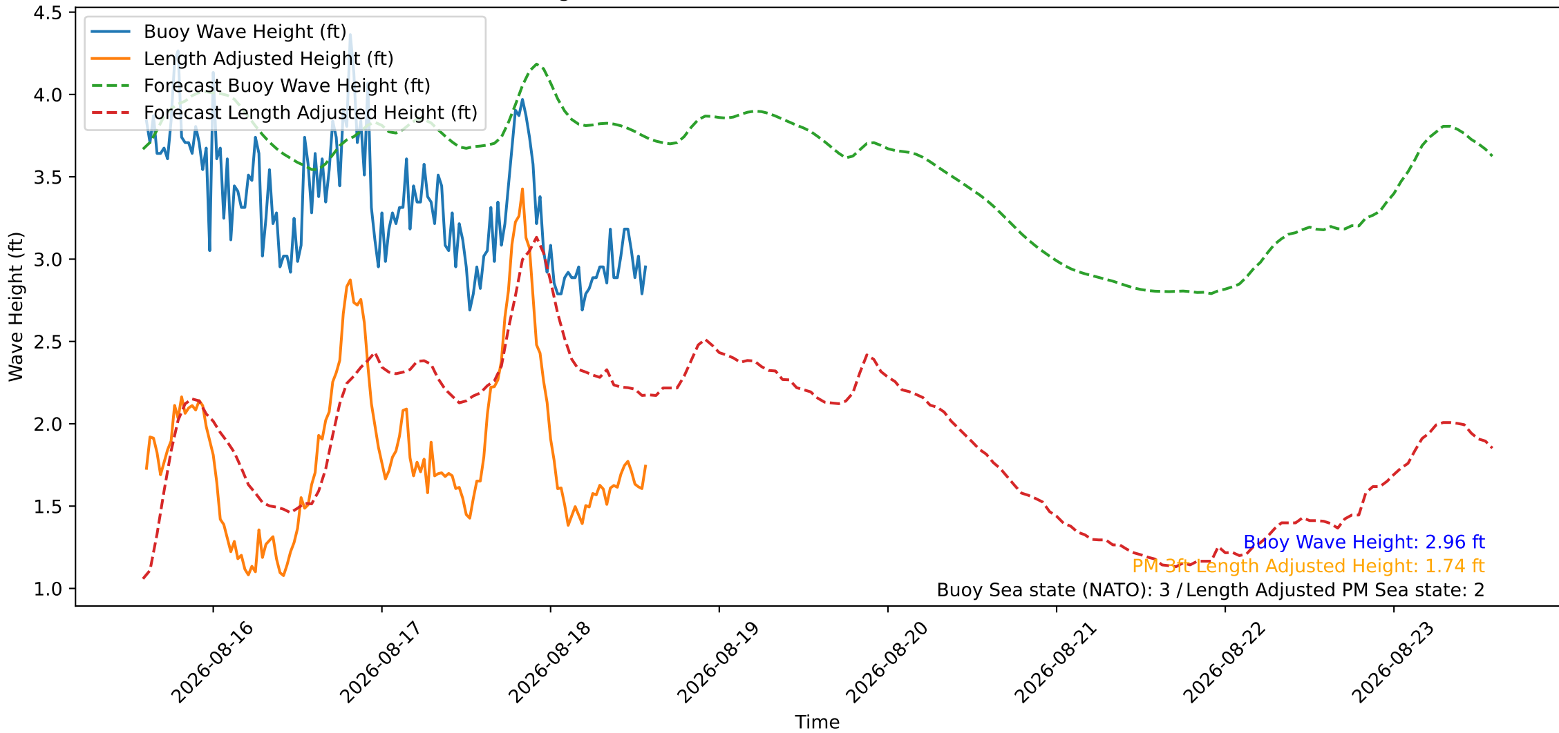
Wave Heights over Time for Green Beach at 2026-08-18 14:21:11
