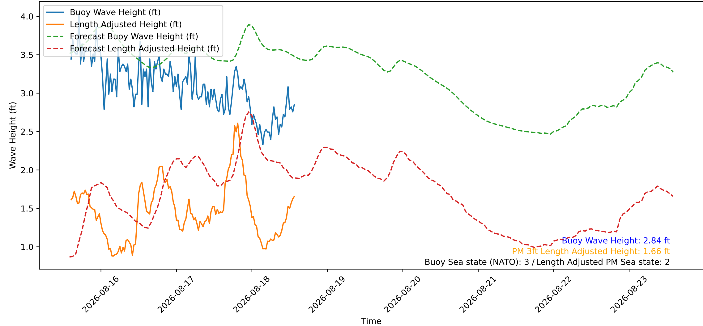
Wave Heights over Time for Red Beach at 2026-08-18 14:20:47
