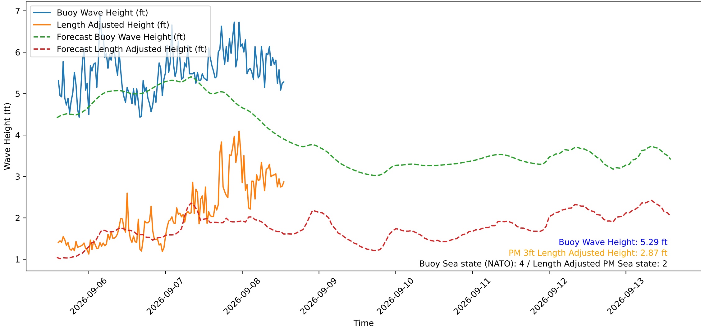
Wave Heights over Time for Red Beach at 2026-09-08 14:00:49
