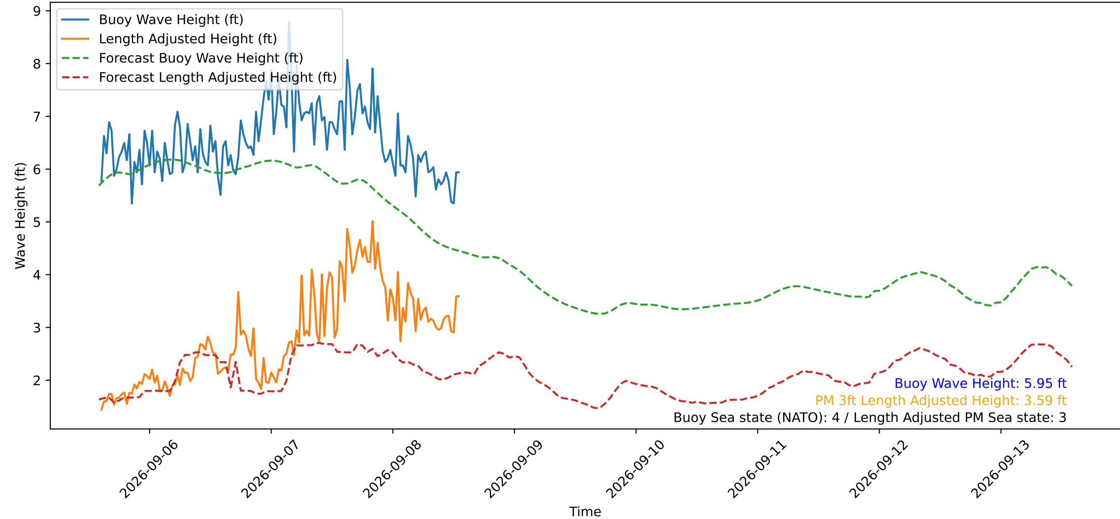
Wave Heights over Time for Green Beach at 2026-09-08 14:01:12
