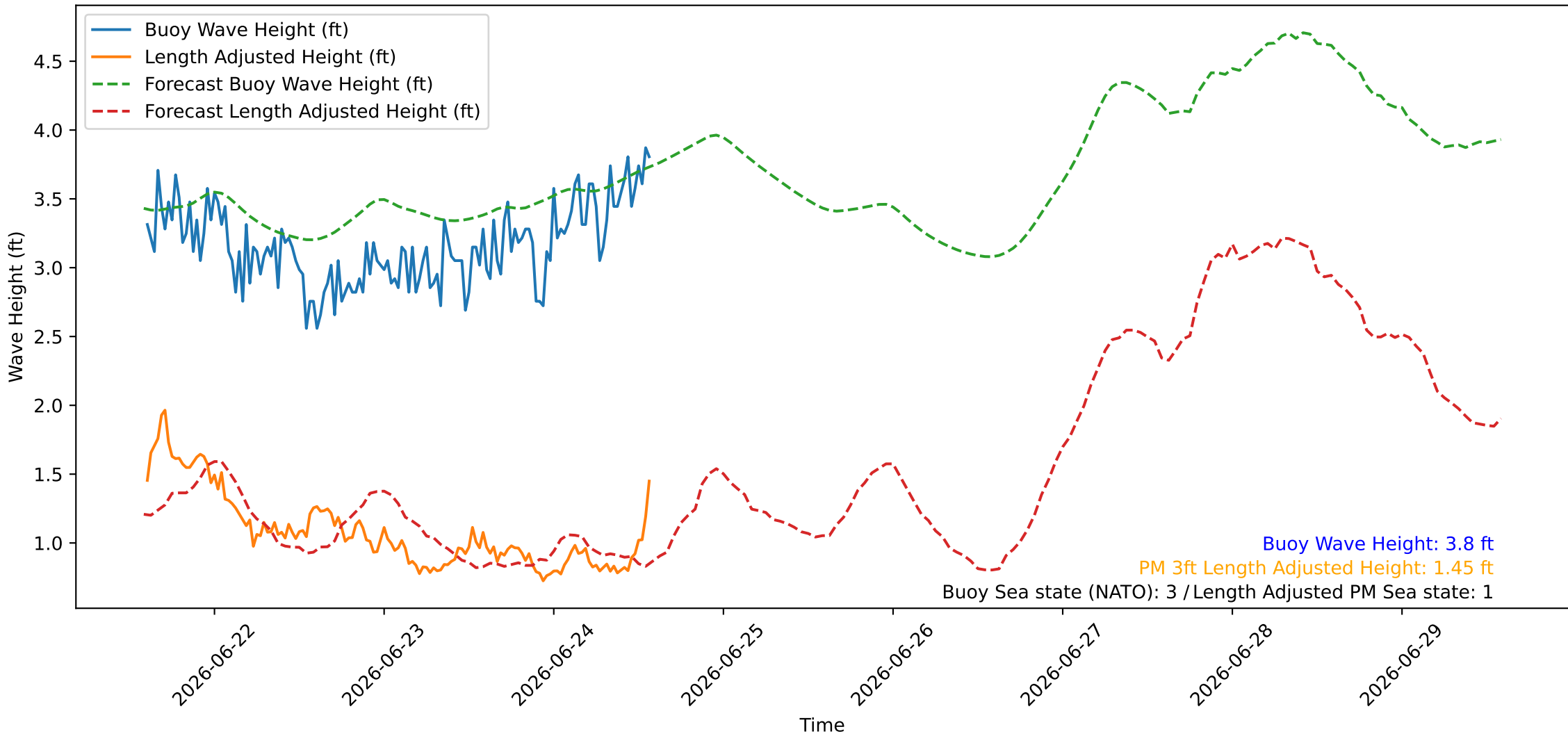
Wave Heights over Time for Oceanside Harbor at 2026-06-24 14:20:26
