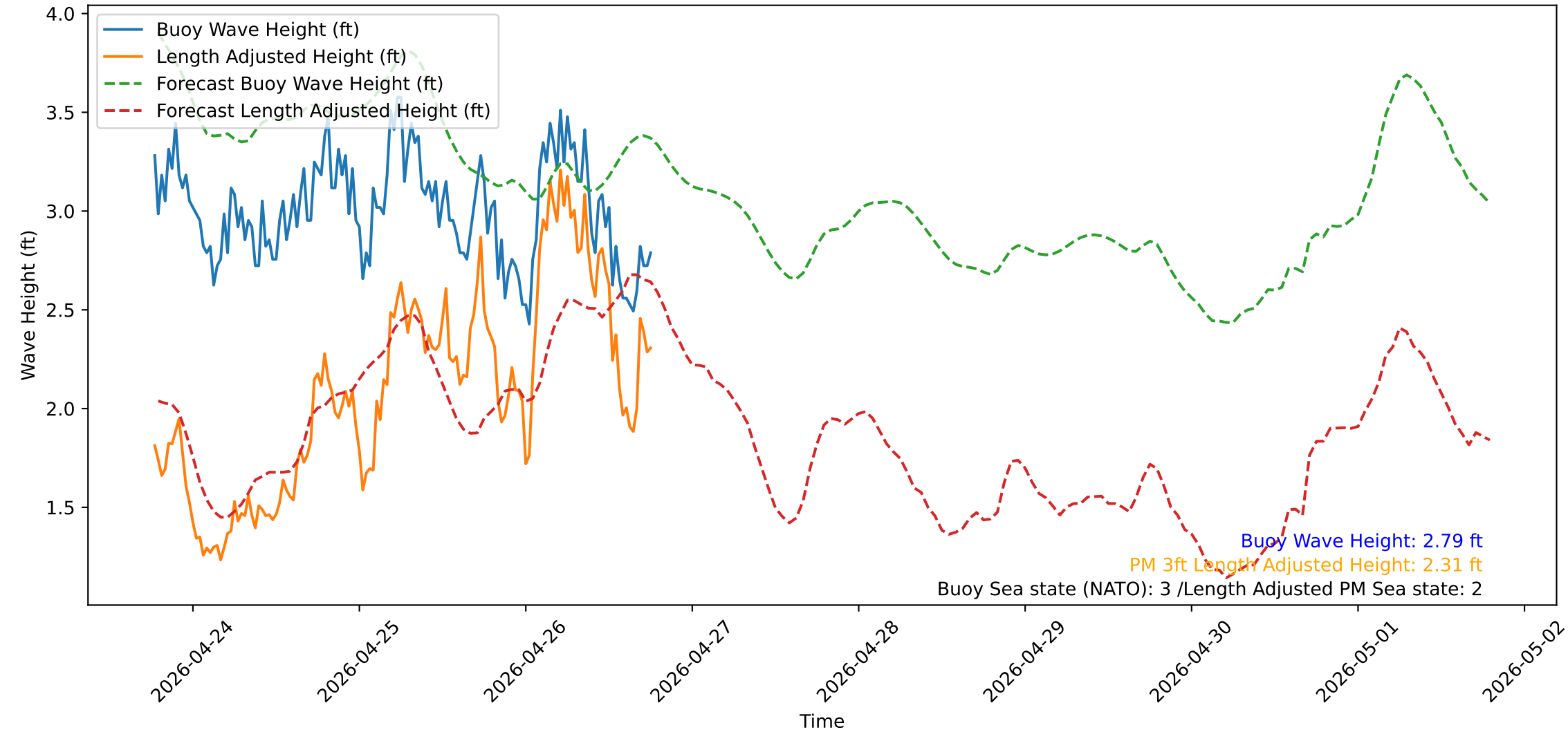
Wave Heights over Time for Green Beach at 2026-04-26 18:41:12
