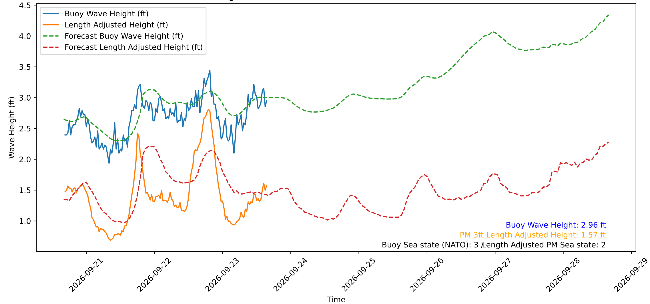
Wave Heights over Time for Green Beach at 2026-09-23 16:21:15
