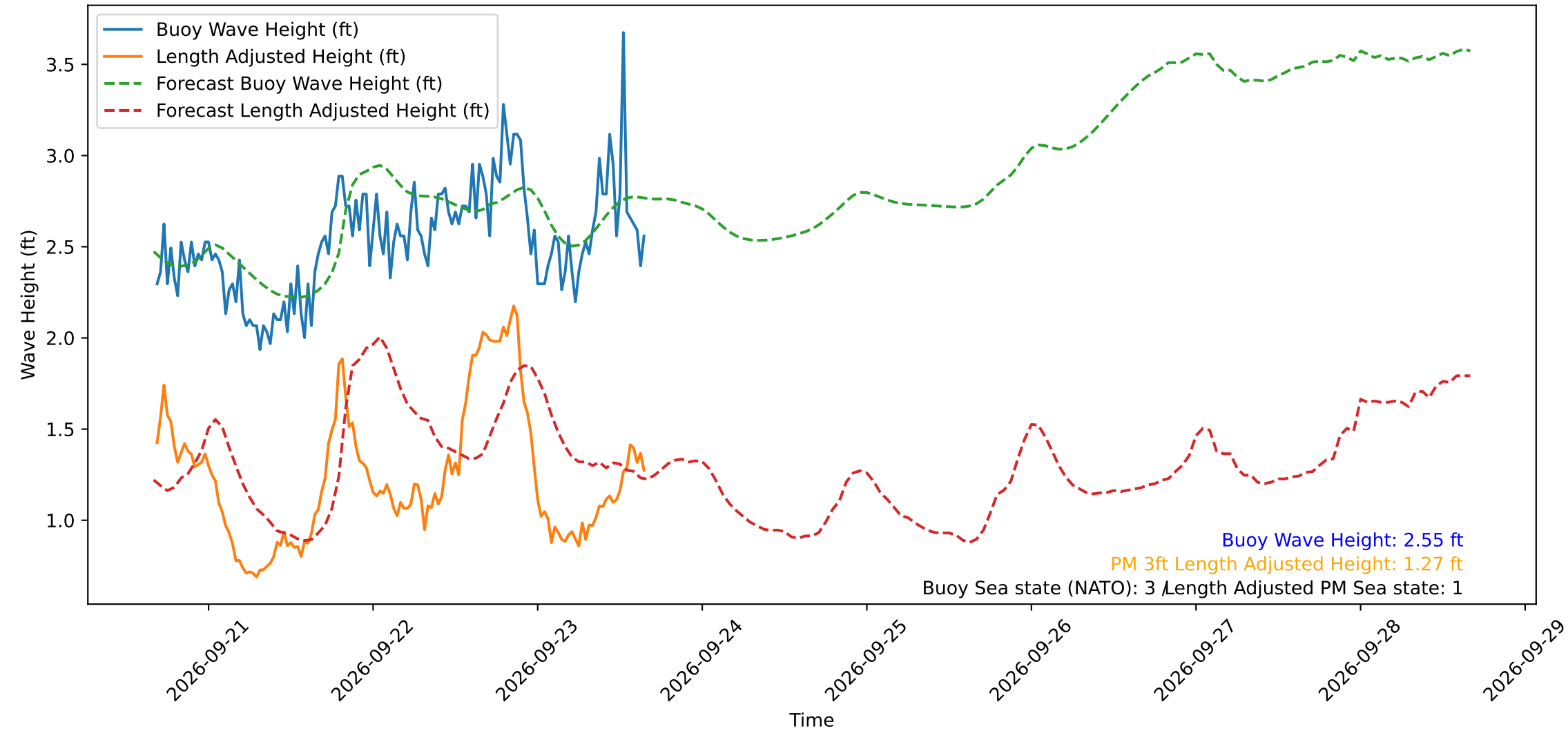
Wave Heights over Time for Red Beach at 2026-09-23 16:20:51
