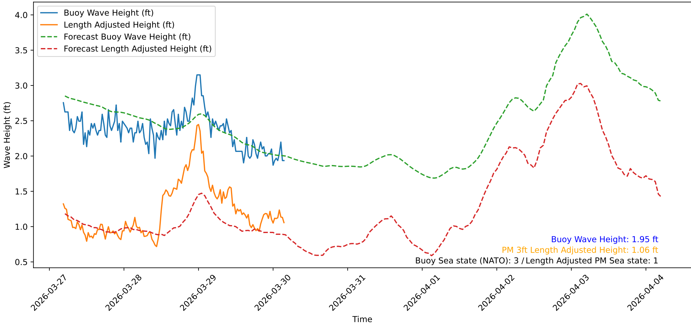
Wave Heights over Time for Oceanside Harbor at 2026-03-30 04:40:31
