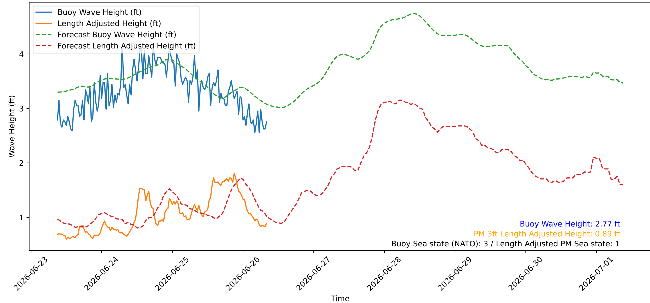
Wave Heights over Time for Green Beach at 2026-06-26 08:51:09
