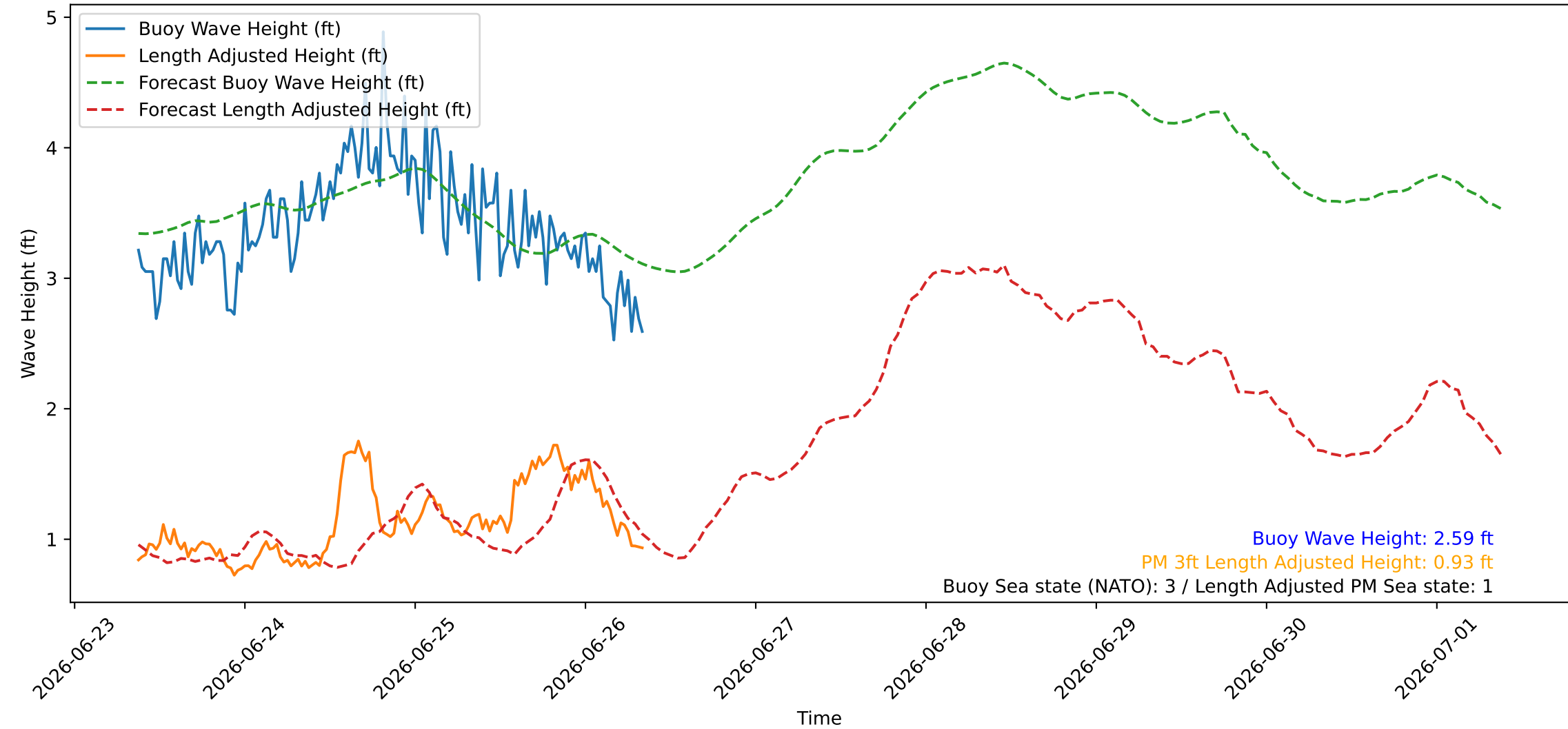
Wave Heights over Time for Oceanside Harbor at 2026-06-26 08:50:27
