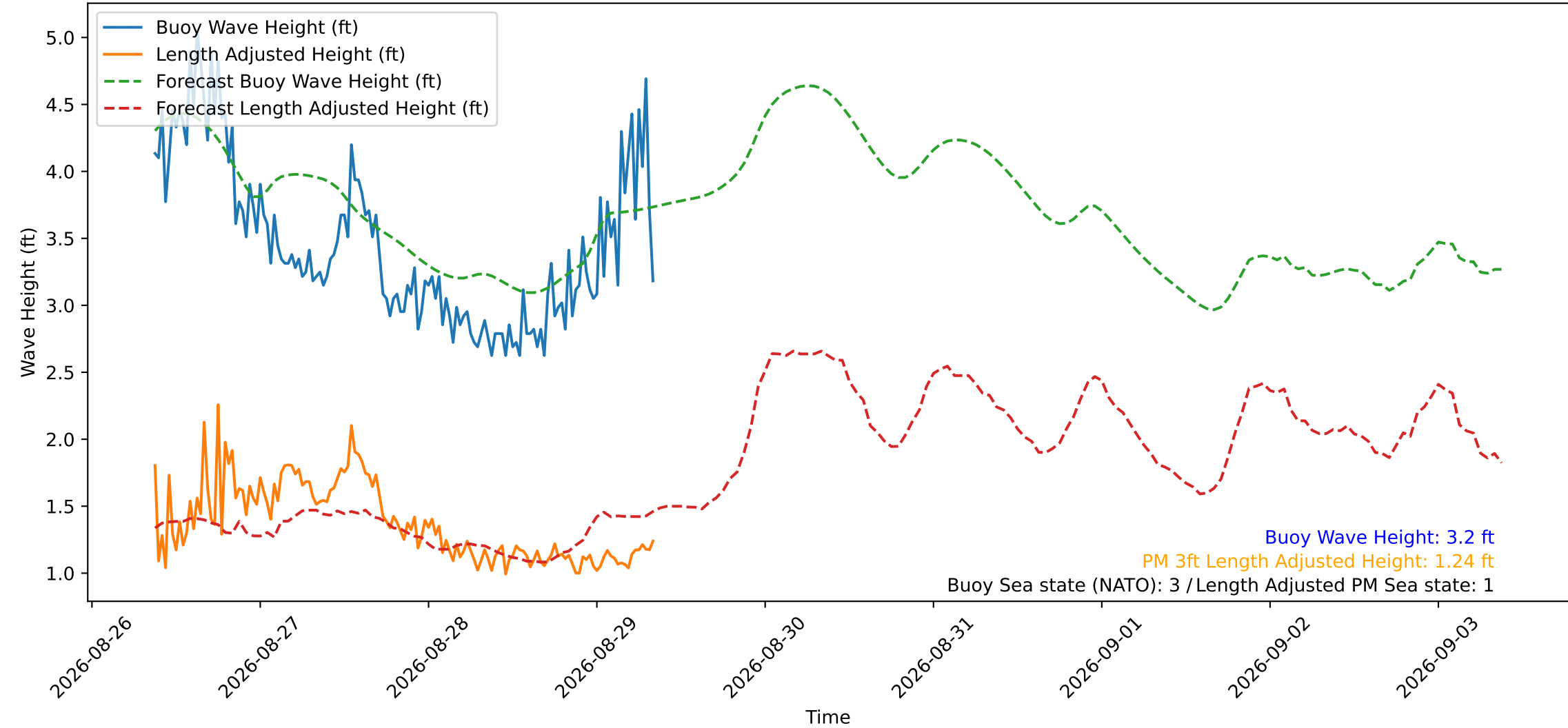
Wave Heights over Time for Red Beach at 2026-08-29 08:40:50
