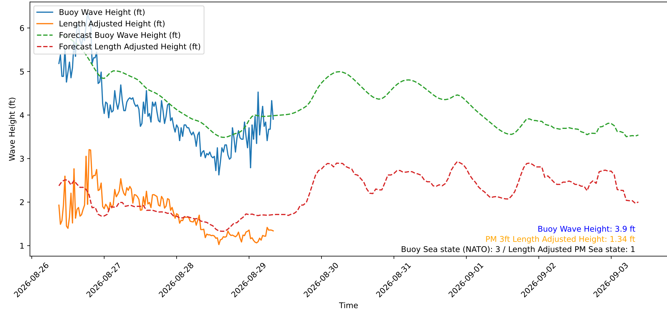
Wave Heights over Time for Green Beach at 2026-08-29 08:41:13
