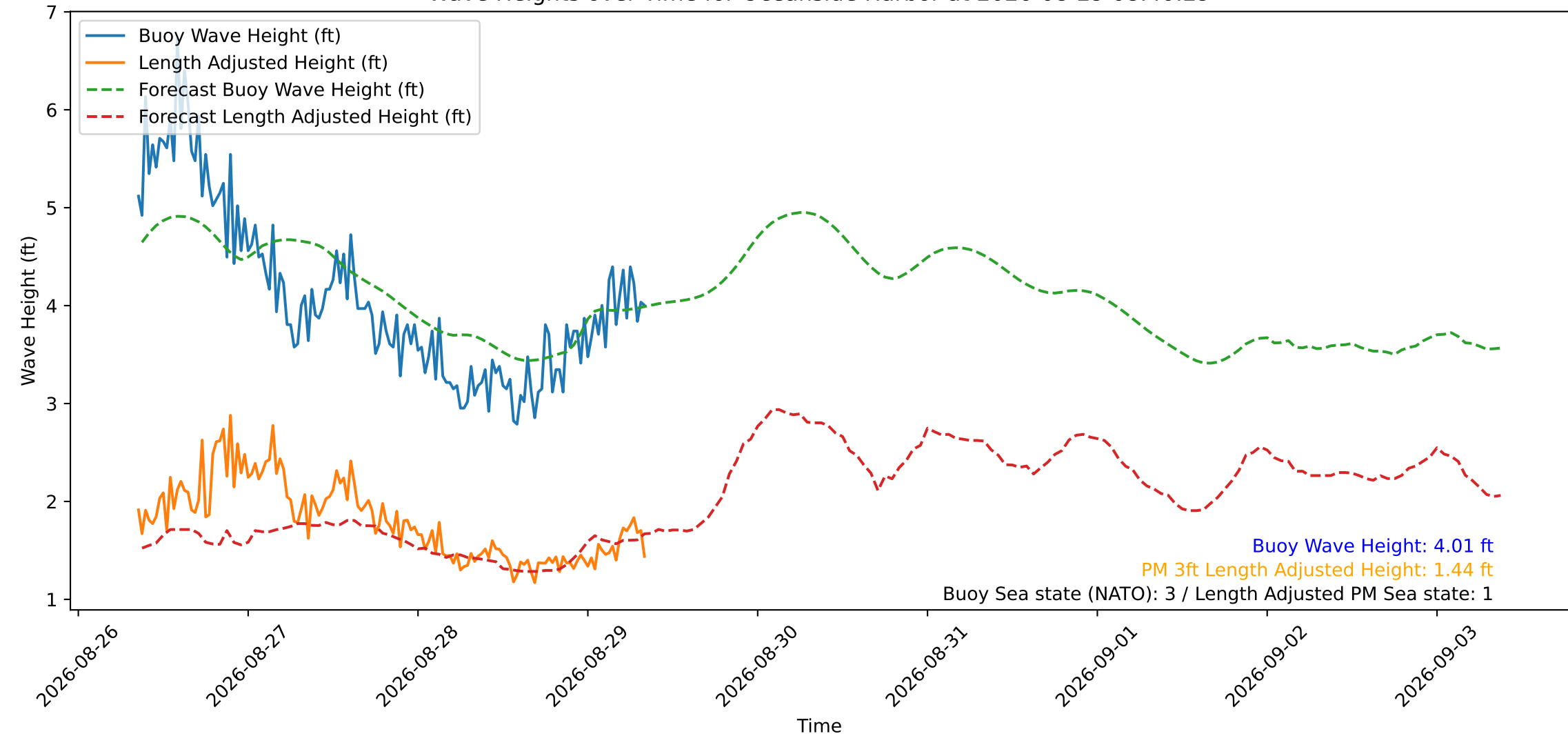
Wave Heights over Time for Oceanside Harbor at 2026-08-29 08:40:29
