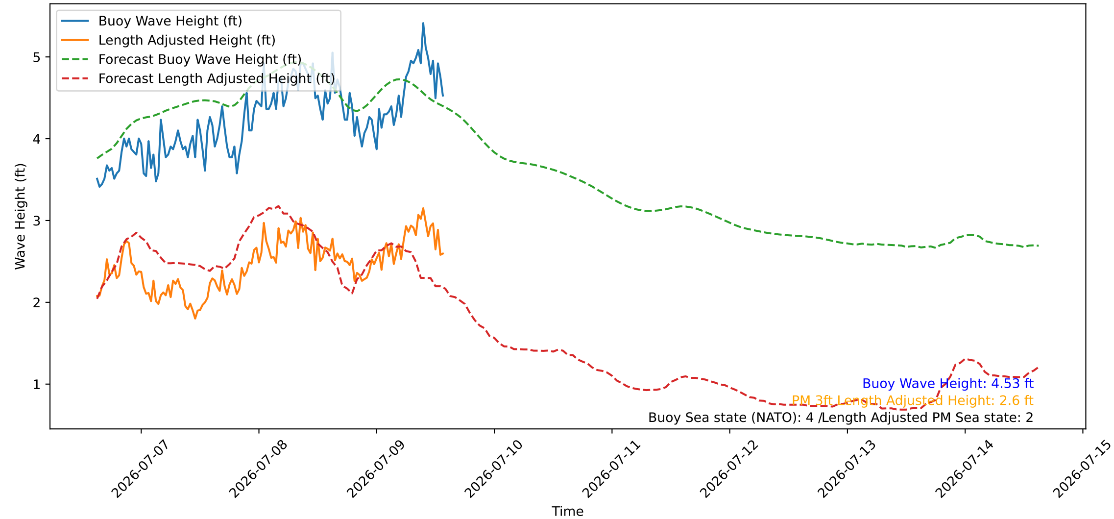
Wave Heights over Time for Oceanside Harbor at 2026-07-09 15:00:26
