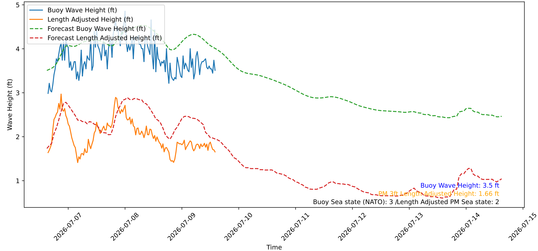
Wave Heights over Time for Red Beach at 2026-07-09 15:00:45
