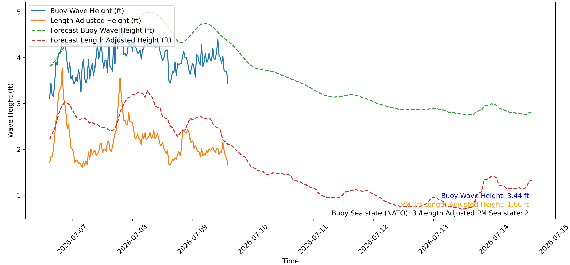
Wave Heights over Time for Green Beach at 2026-07-09 15:01:08
