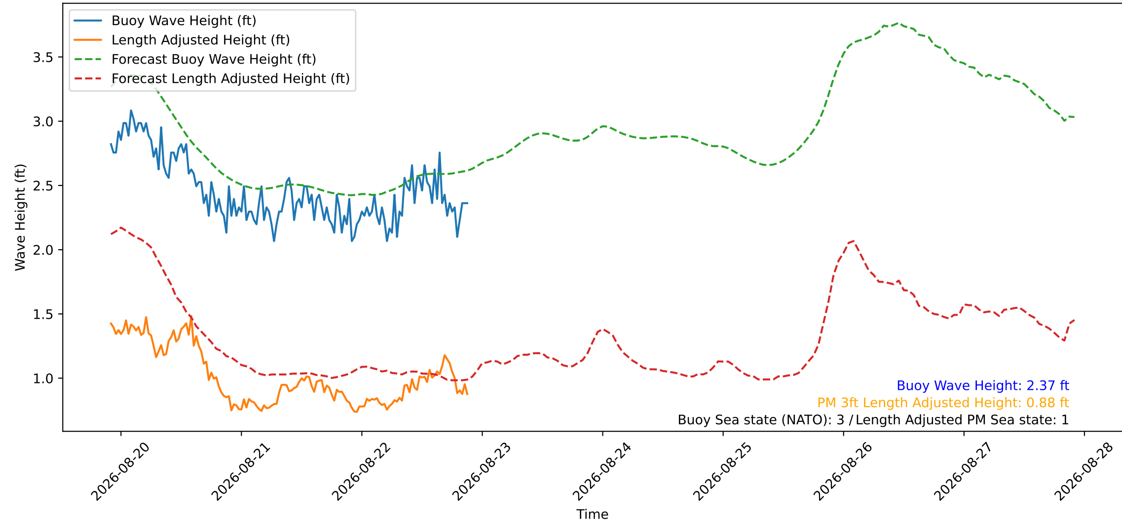
Wave Heights over Time for Red Beach at 2026-08-22 21:50:50
