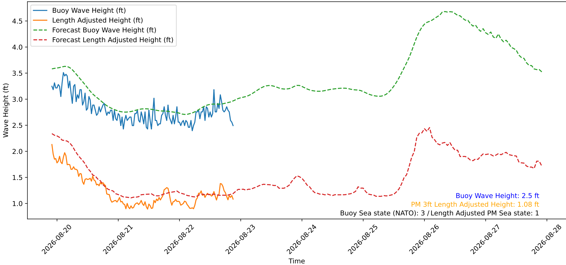
Wave Heights over Time for Green Beach at 2026-08-22 21:51:14
