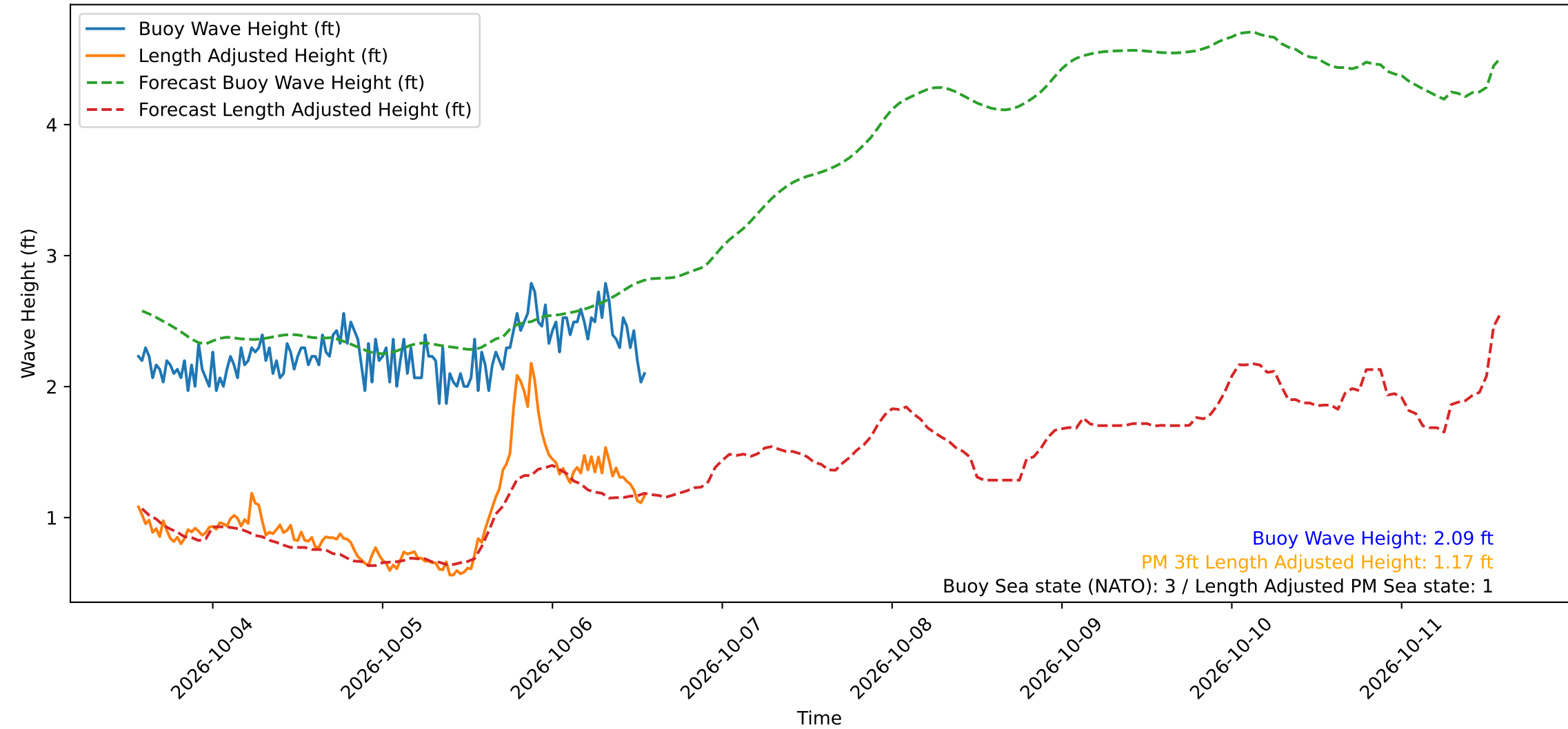
Wave Heights over Time for Oceanside Harbor at 2026-10-06 13:40:30
