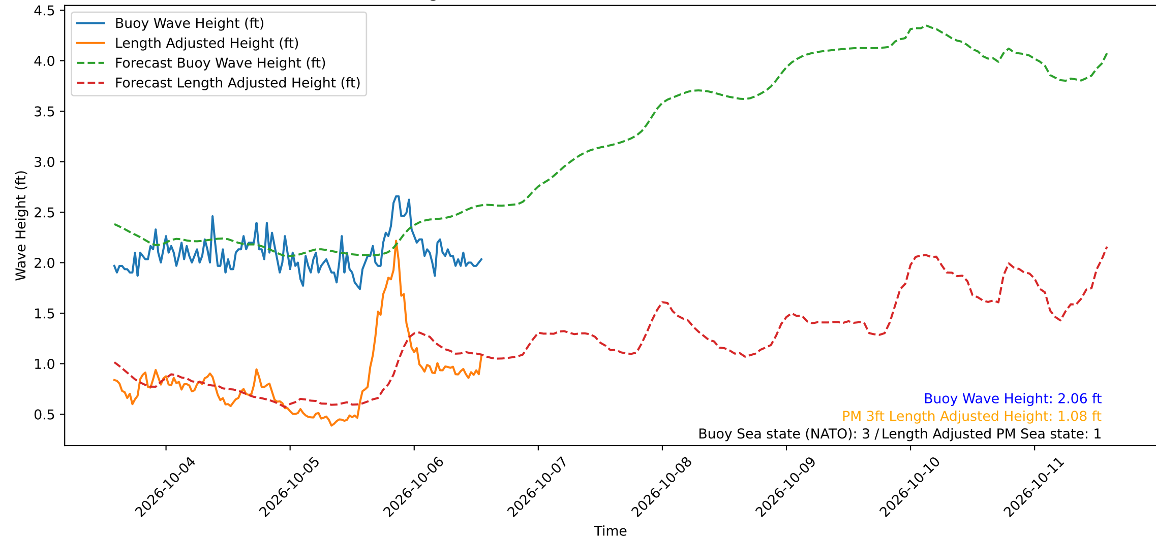
Wave Heights over Time for Red Beach at 2026-10-06 13:40:49
