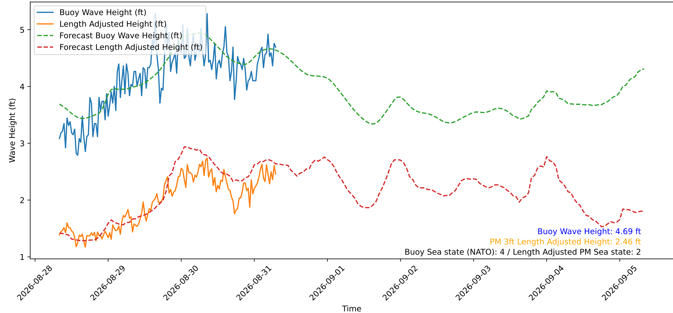
Wave Heights over Time for Oceanside Harbor at 2026-08-31 08:00:30
