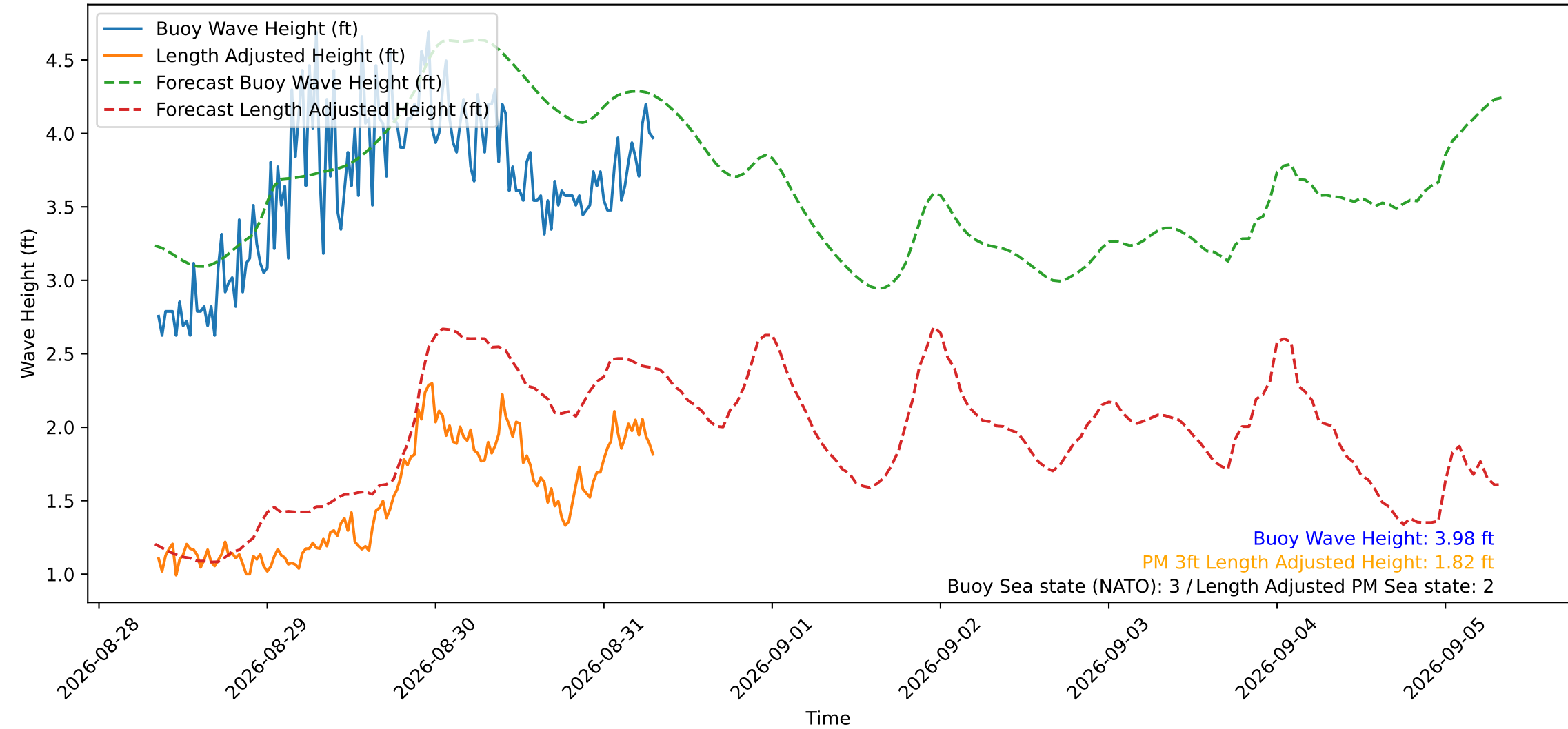
Wave Heights over Time for Red Beach at 2026-08-31 08:00:50
