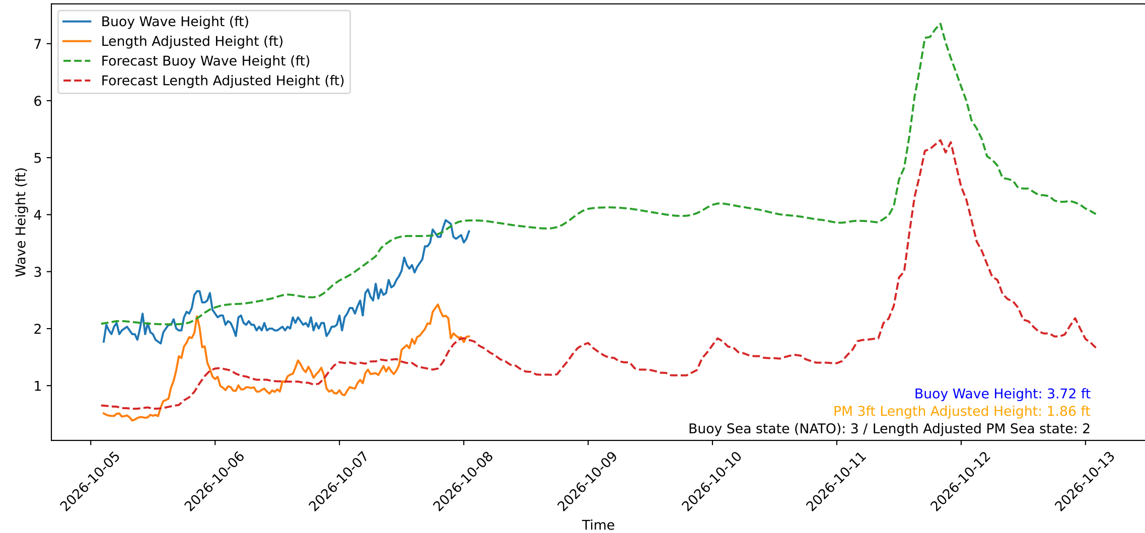
Wave Heights over Time for Red Beach at 2026-10-08 02:00:48
