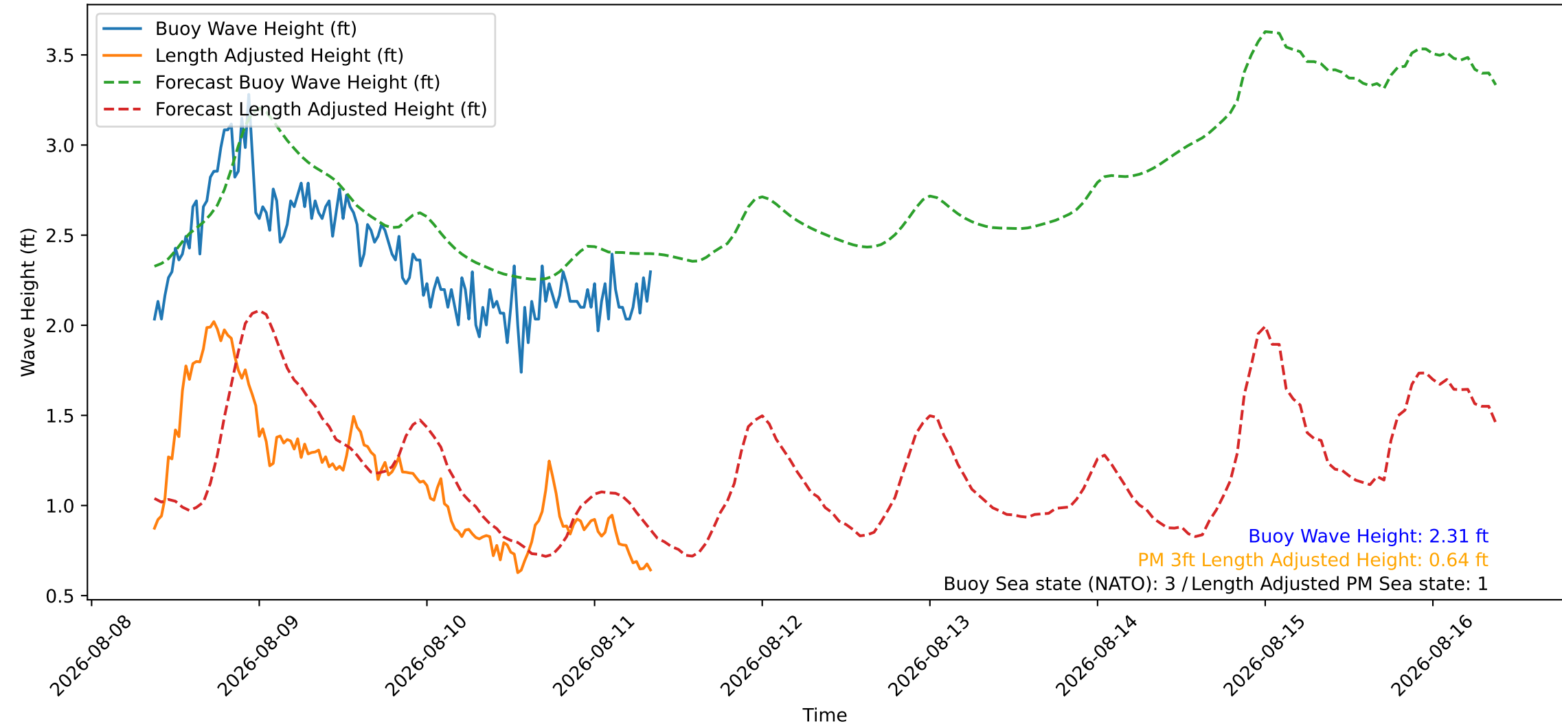
Wave Heights over Time for Red Beach at 2026-08-11 08:50:47
