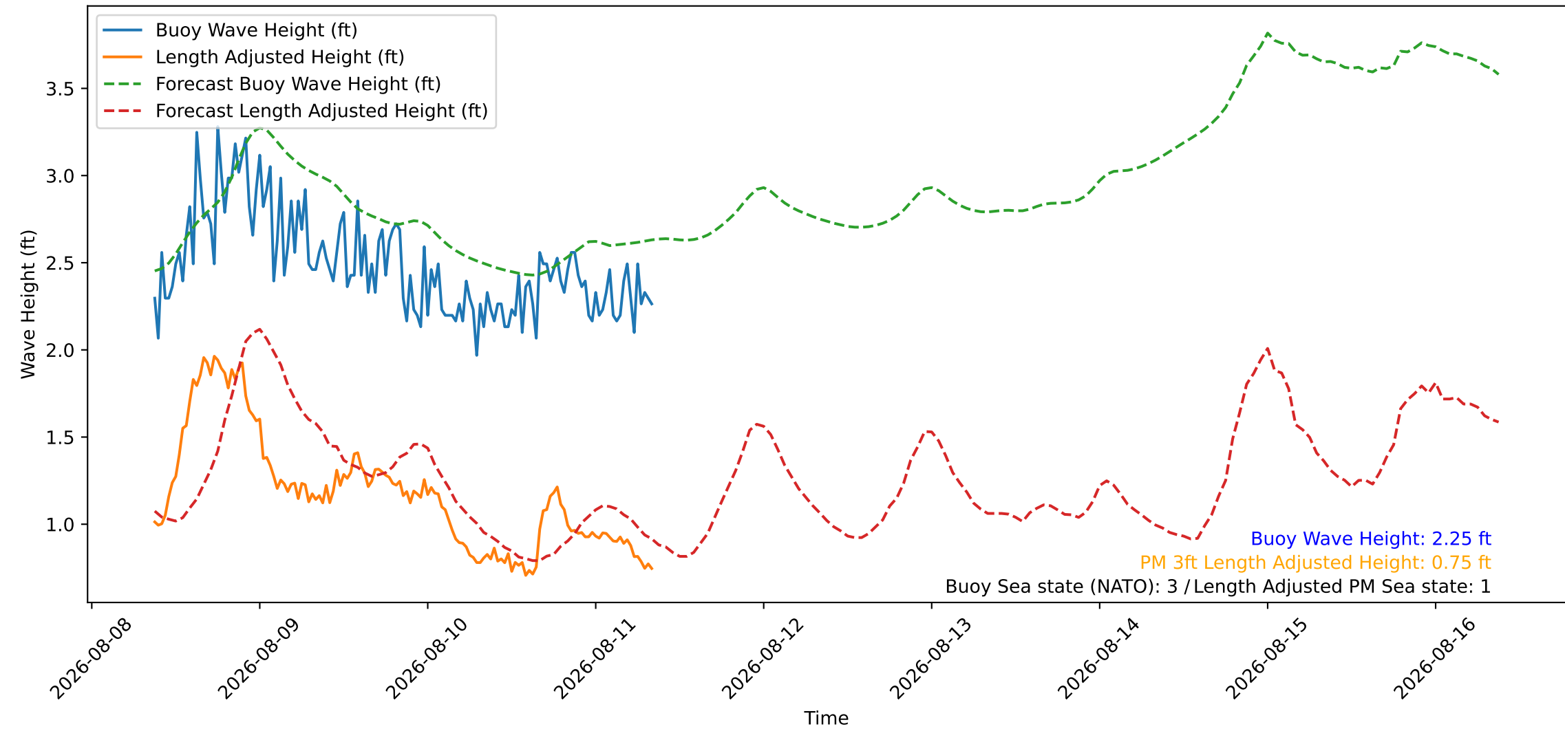
Wave Heights over Time for Oceanside Harbor at 2026-08-11 08:50:26
