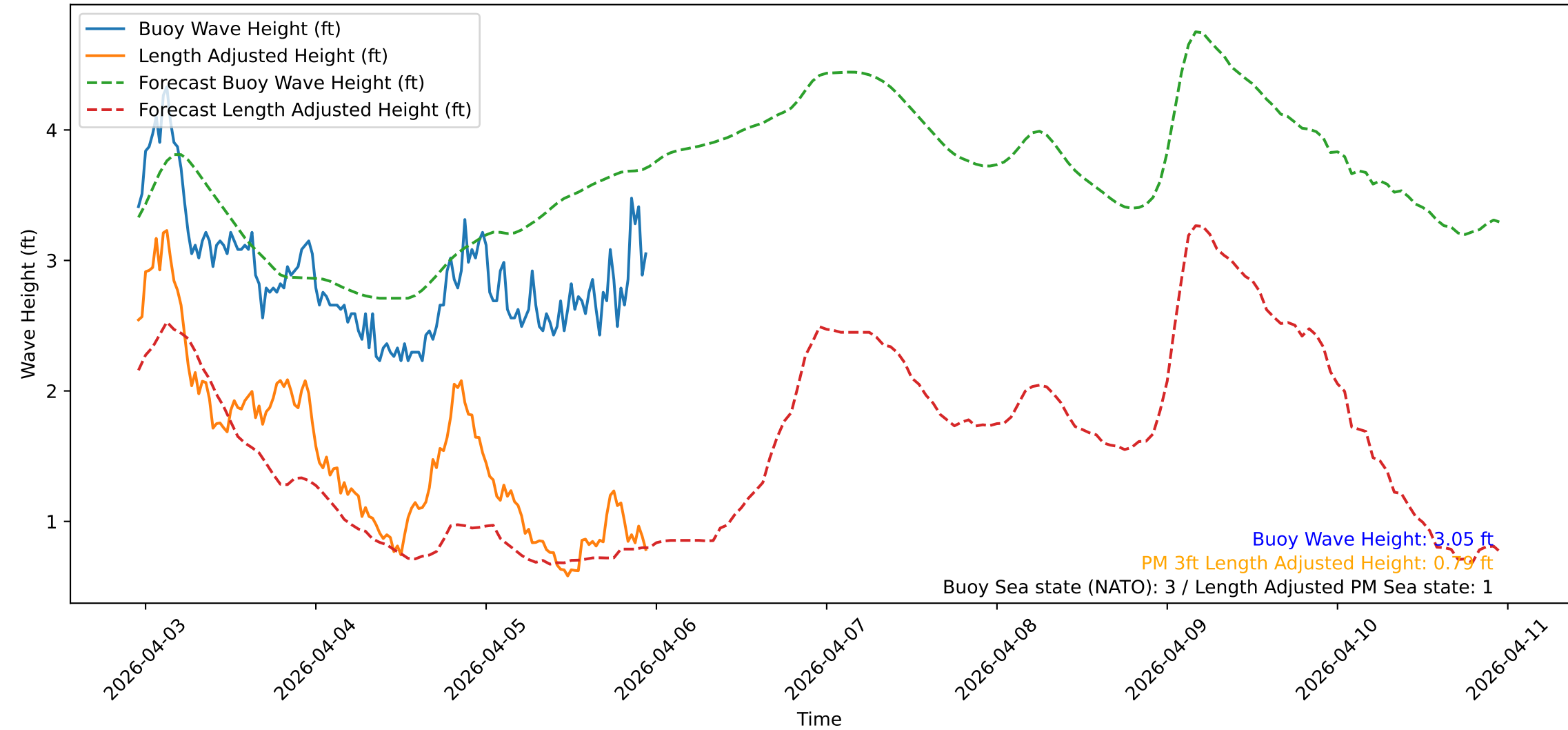
Wave Heights over Time for Green Beach at 2026-04-05 23:11:11
