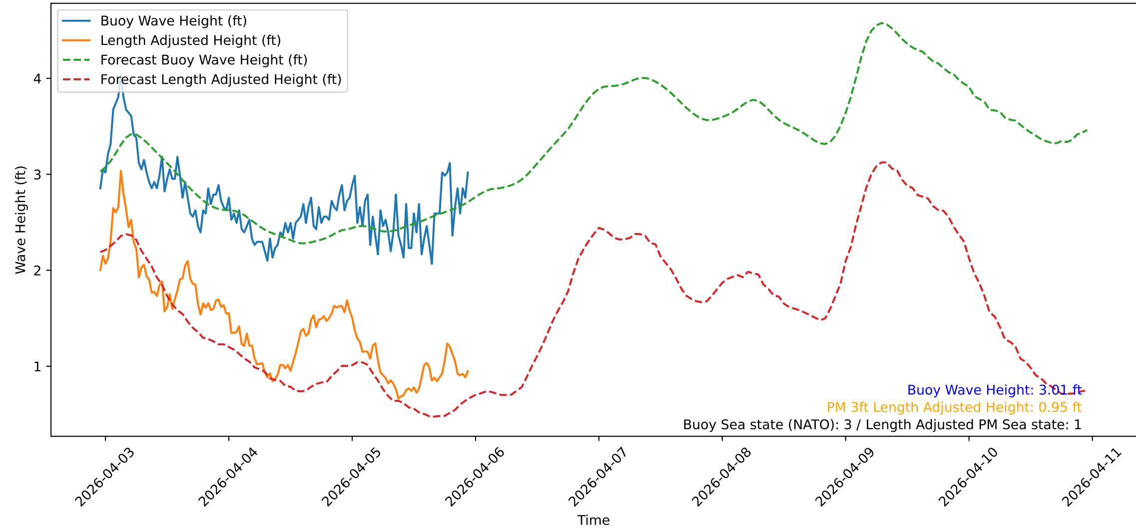
Wave Heights over Time for Oceanside Harbor at 2026-04-05 23:10:32
