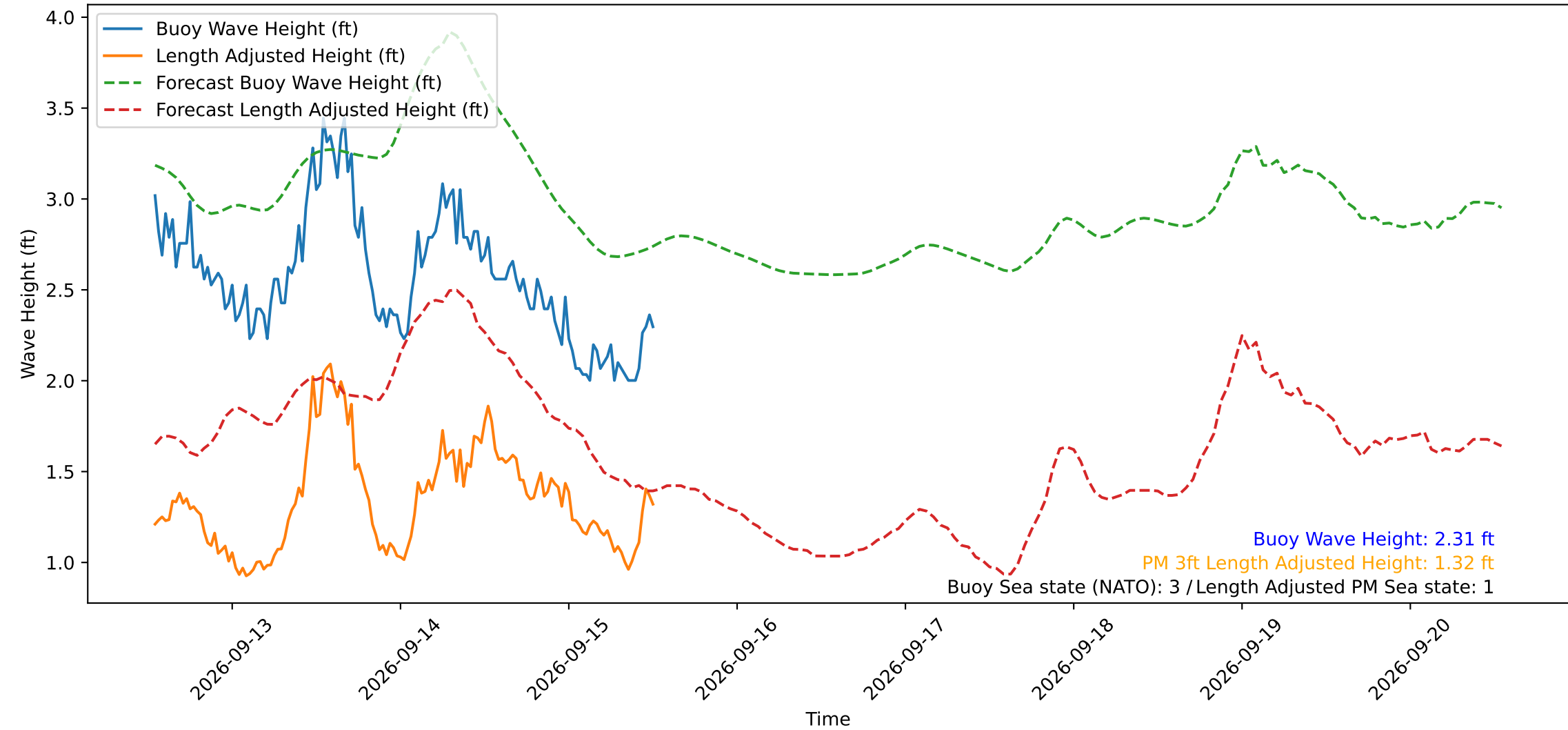
Wave Heights over Time for Red Beach at 2026-09-15 12:50:50
