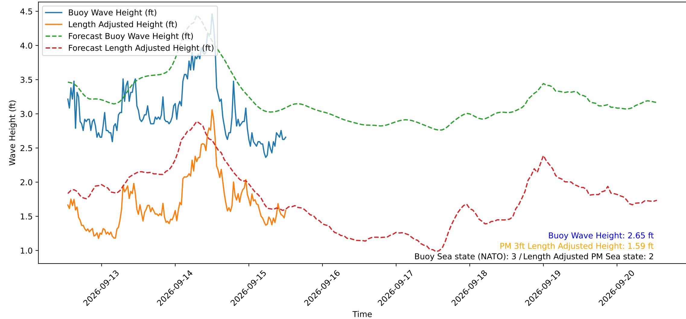
Wave Heights over Time for Oceanside Harbor at 2026-09-15 12:50:29
