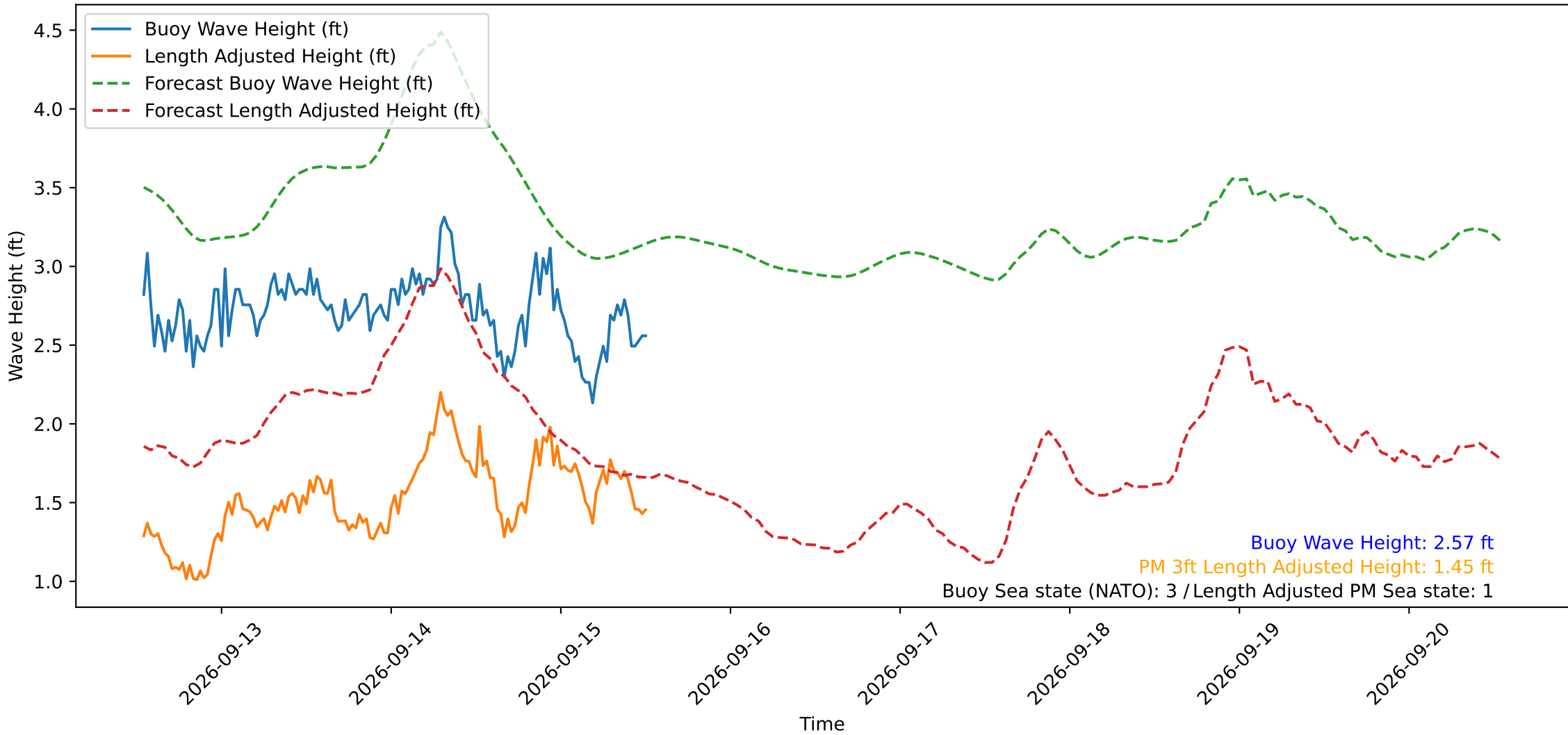
Wave Heights over Time for Green Beach at 2026-09-15 12:51:14
