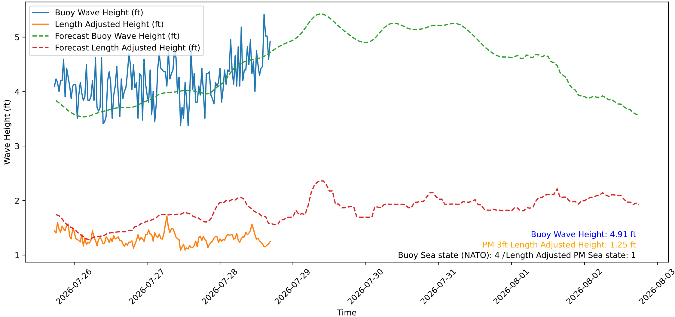
Wave Heights over Time for Green Beach at 2026-07-28 17:31:08
