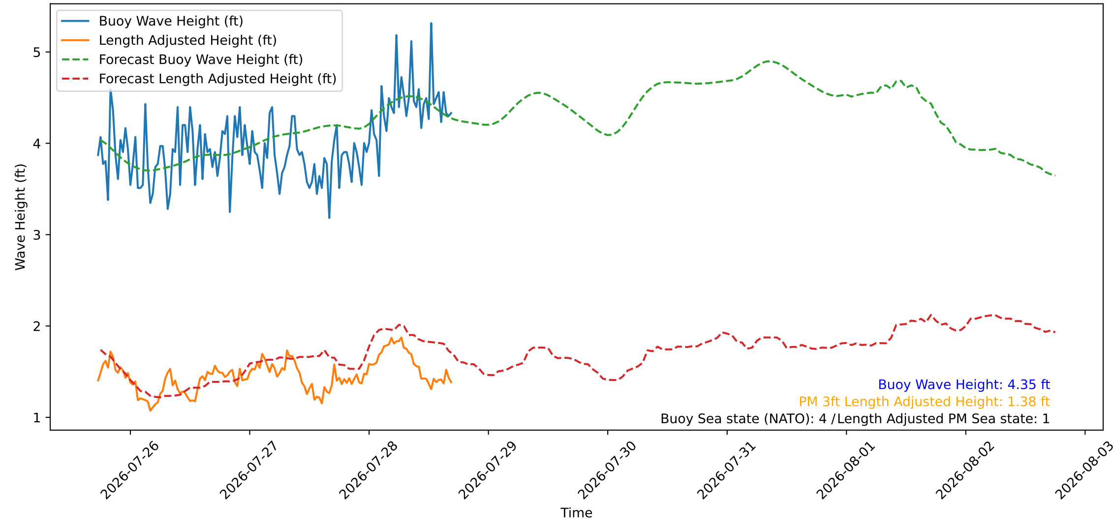
Wave Heights over Time for Oceanside Harbor at 2026-07-28 17:30:27
