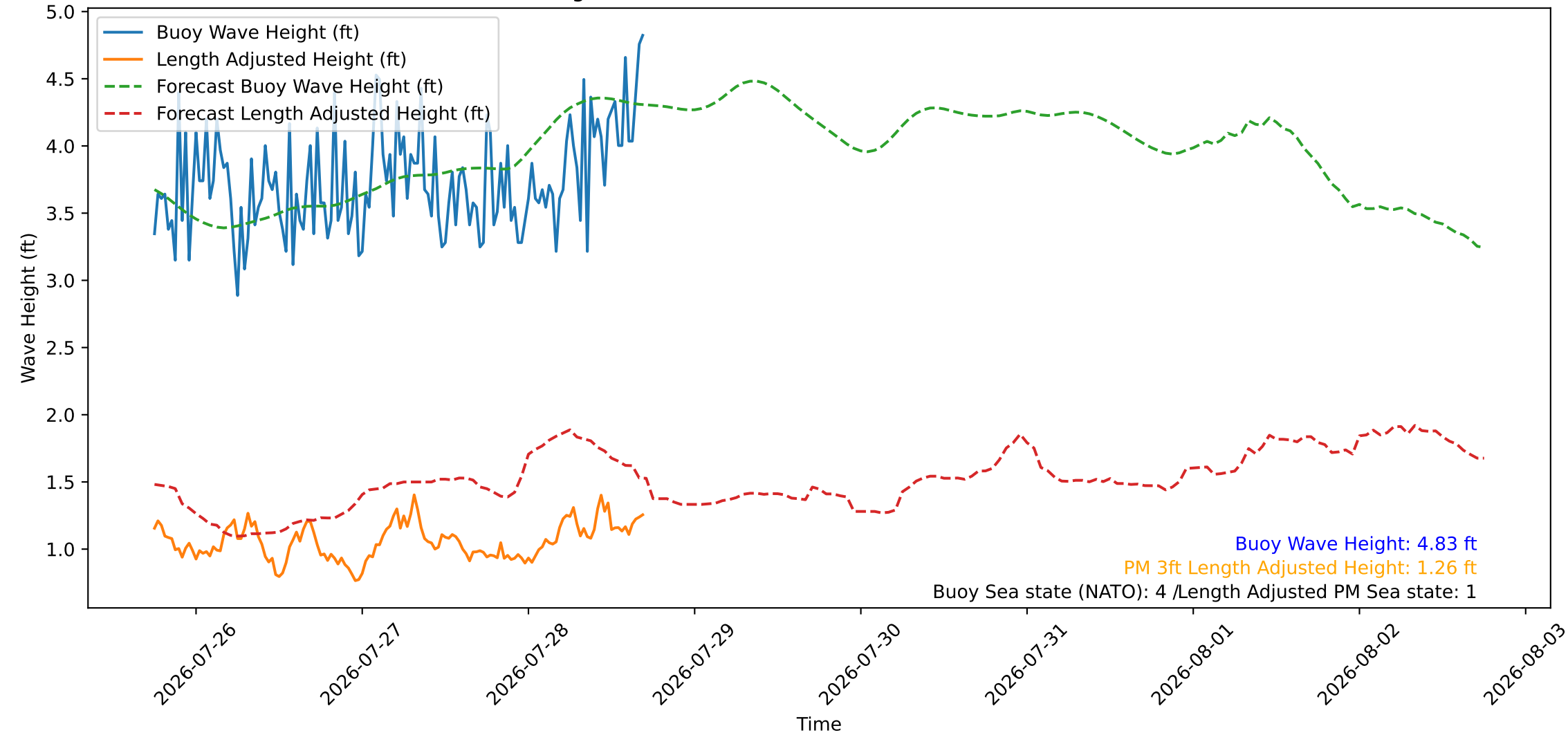
Wave Heights over Time for Red Beach at 2026-07-28 17:30:46
