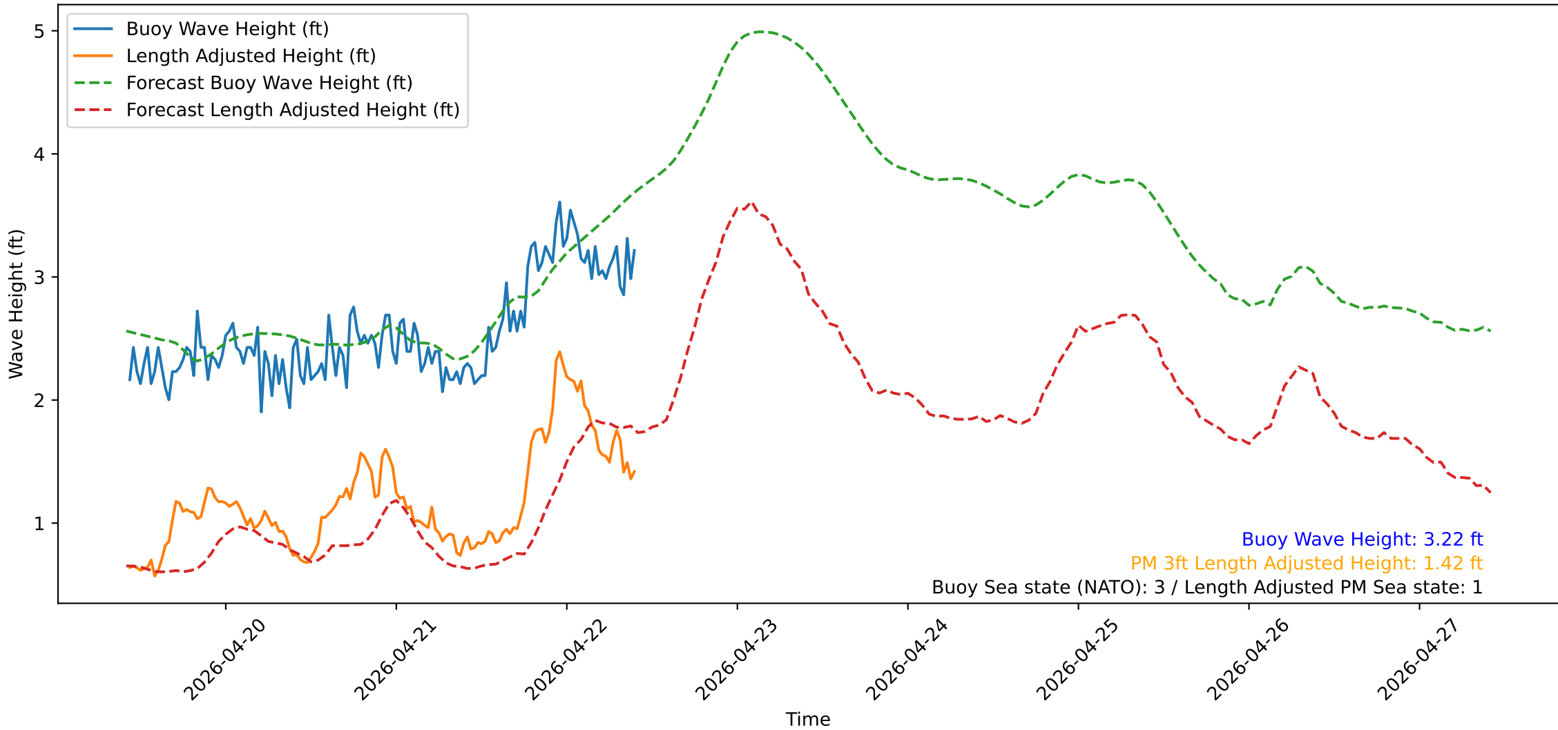
Wave Heights over Time for Oceanside Harbor at 2026-04-22 10:20:30
