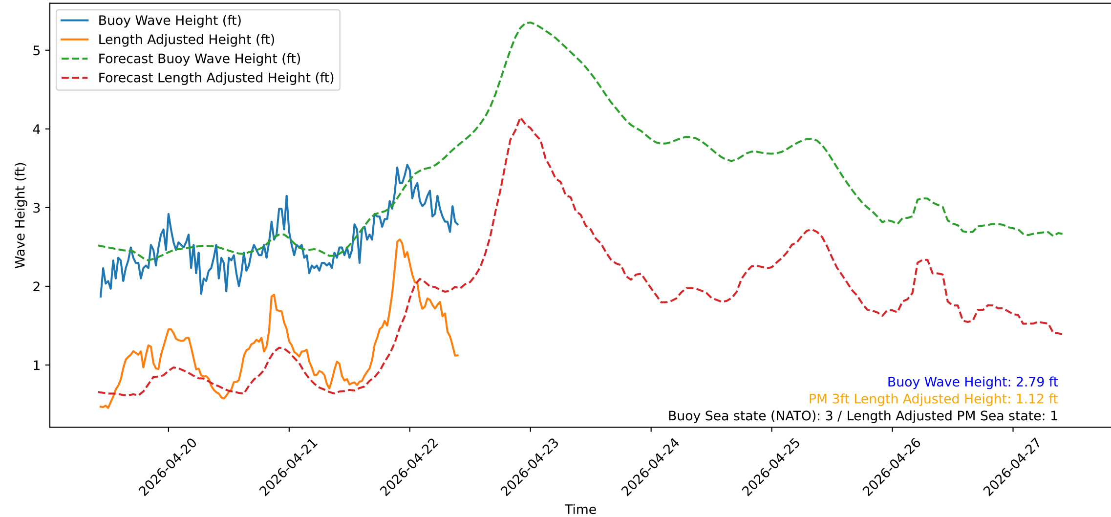
Wave Heights over Time for Green Beach at 2026-04-22 10:21:12
