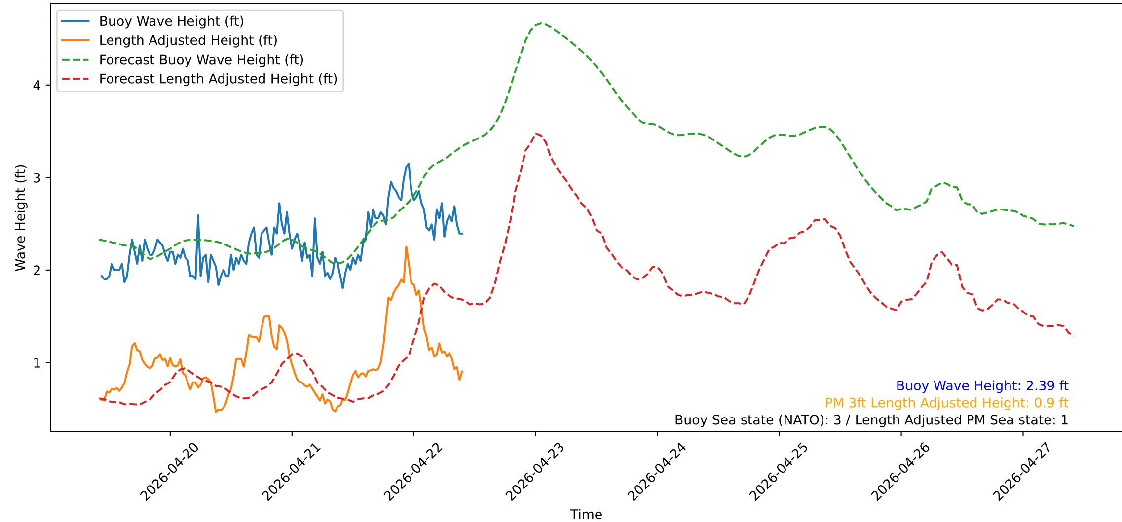
Wave Heights over Time for Red Beach at 2026-04-22 10:20:50
