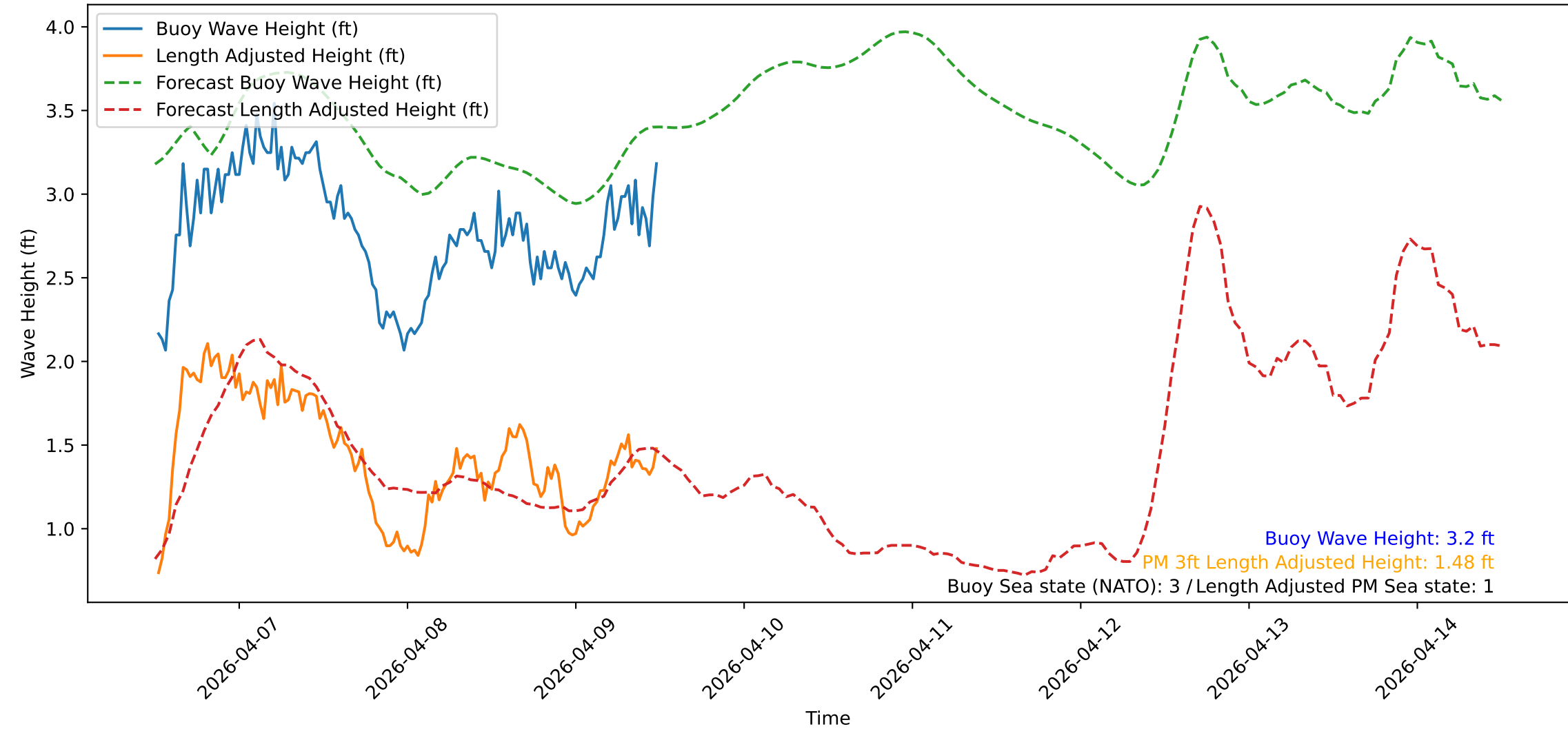
Wave Heights over Time for Red Beach at 2026-04-09 12:20:47
