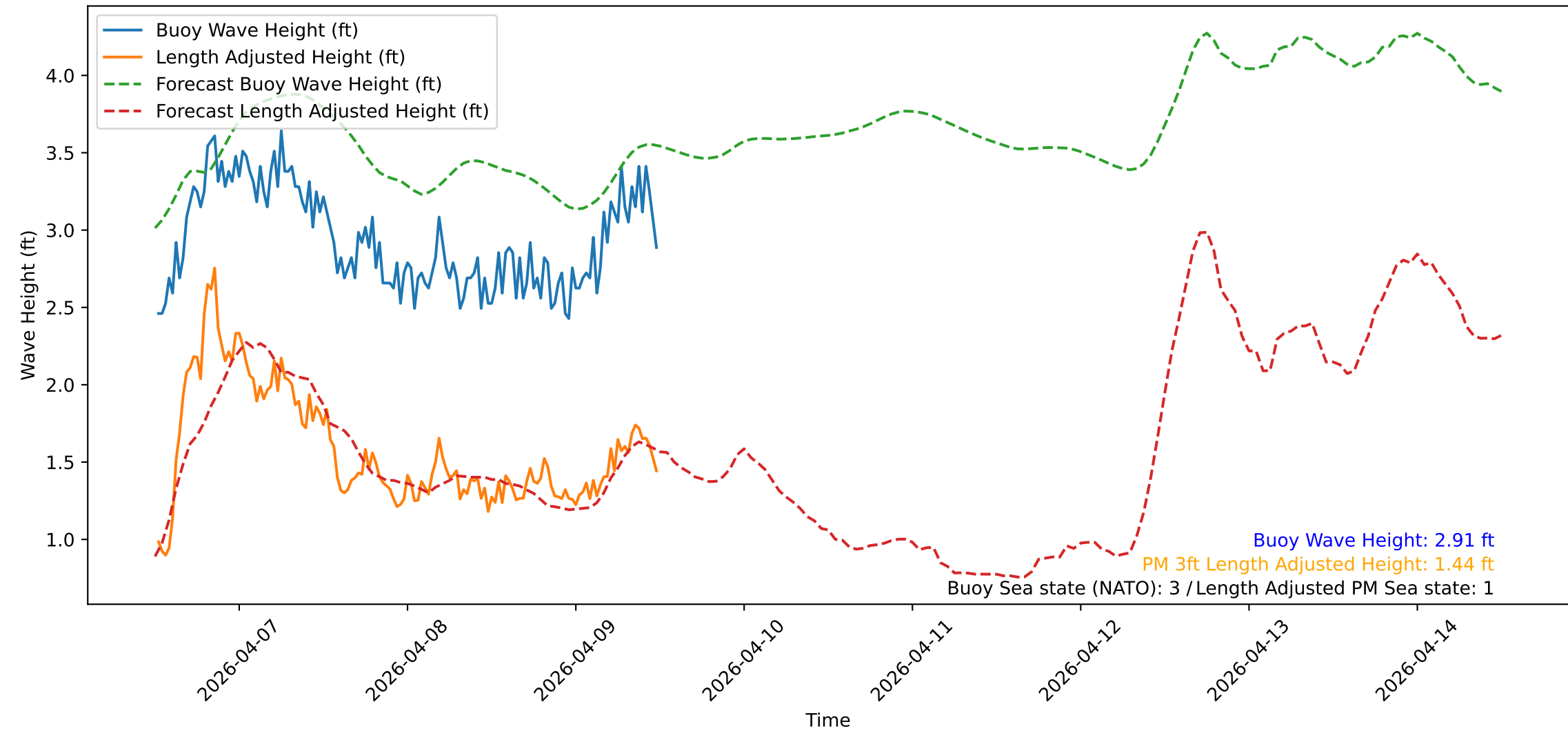
Wave Heights over Time for Oceanside Harbor at 2026-04-09 12:20:31
