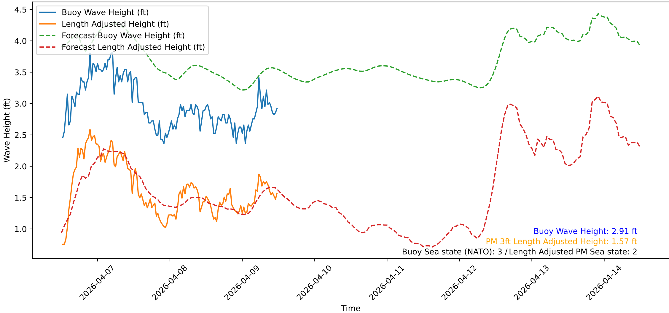
Wave Heights over Time for Green Beach at 2026-04-09 12:21:09
