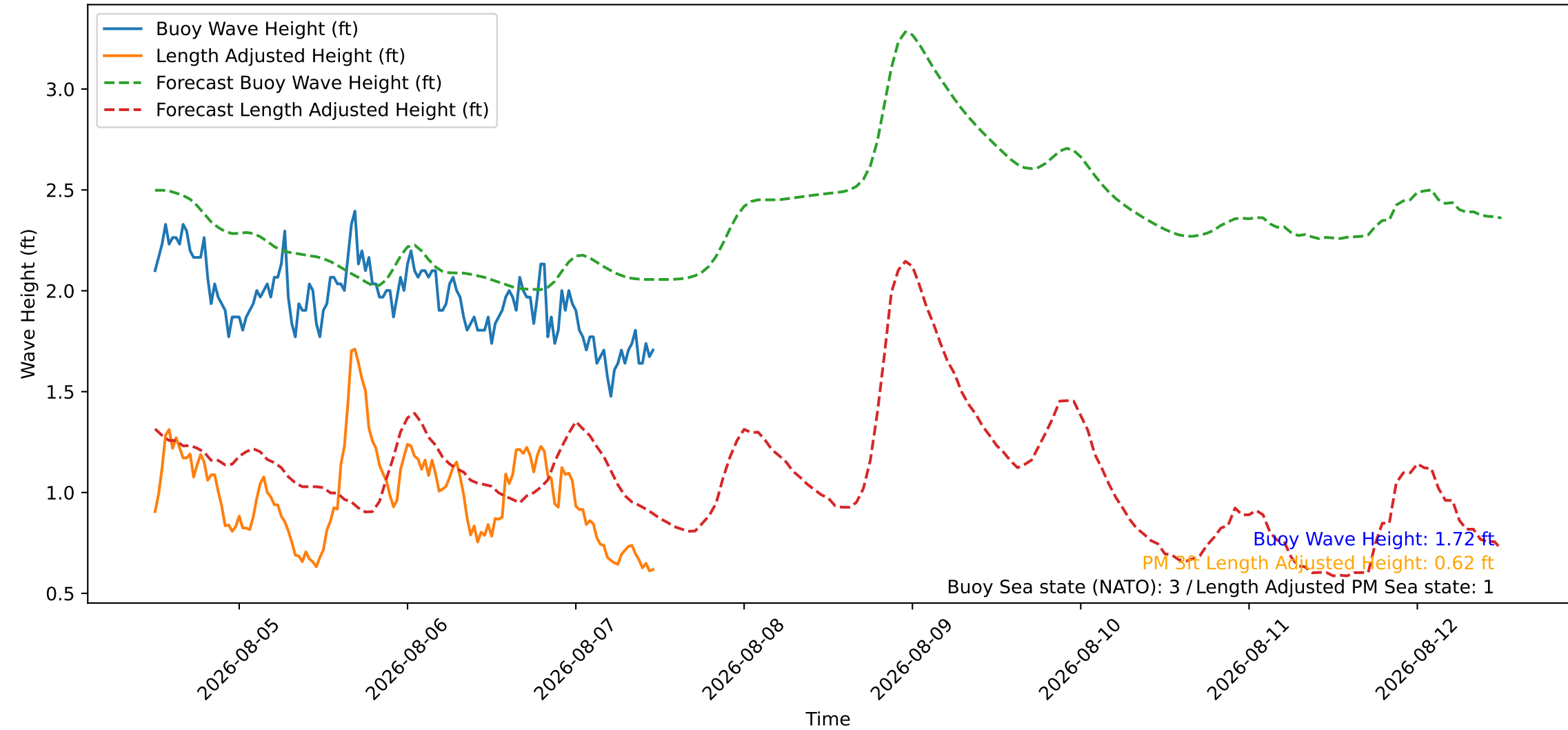
Wave Heights over Time for Red Beach at 2026-08-07 11:50:47
