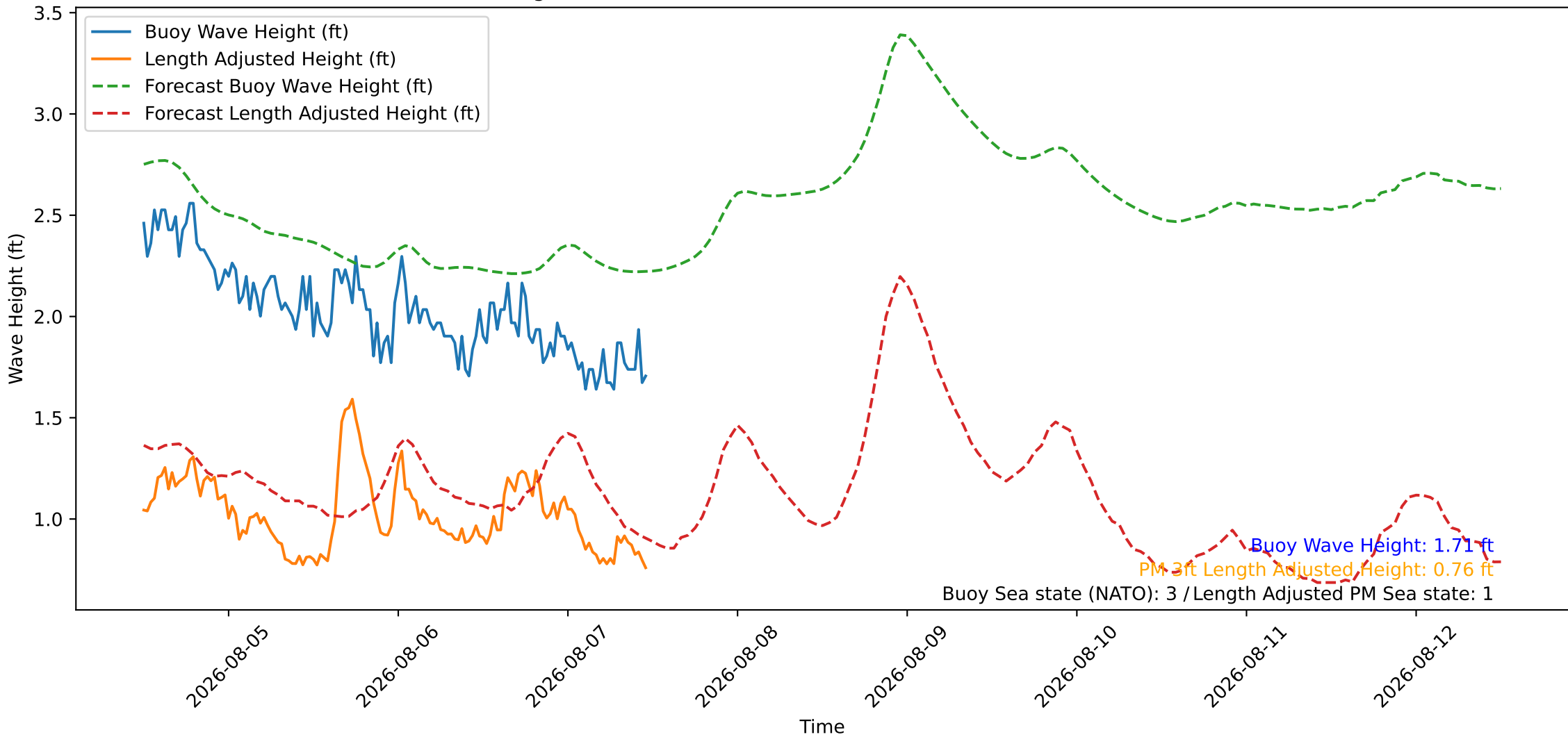
Wave Heights over Time for Oceanside Harbor at 2026-08-07 11:50:27
