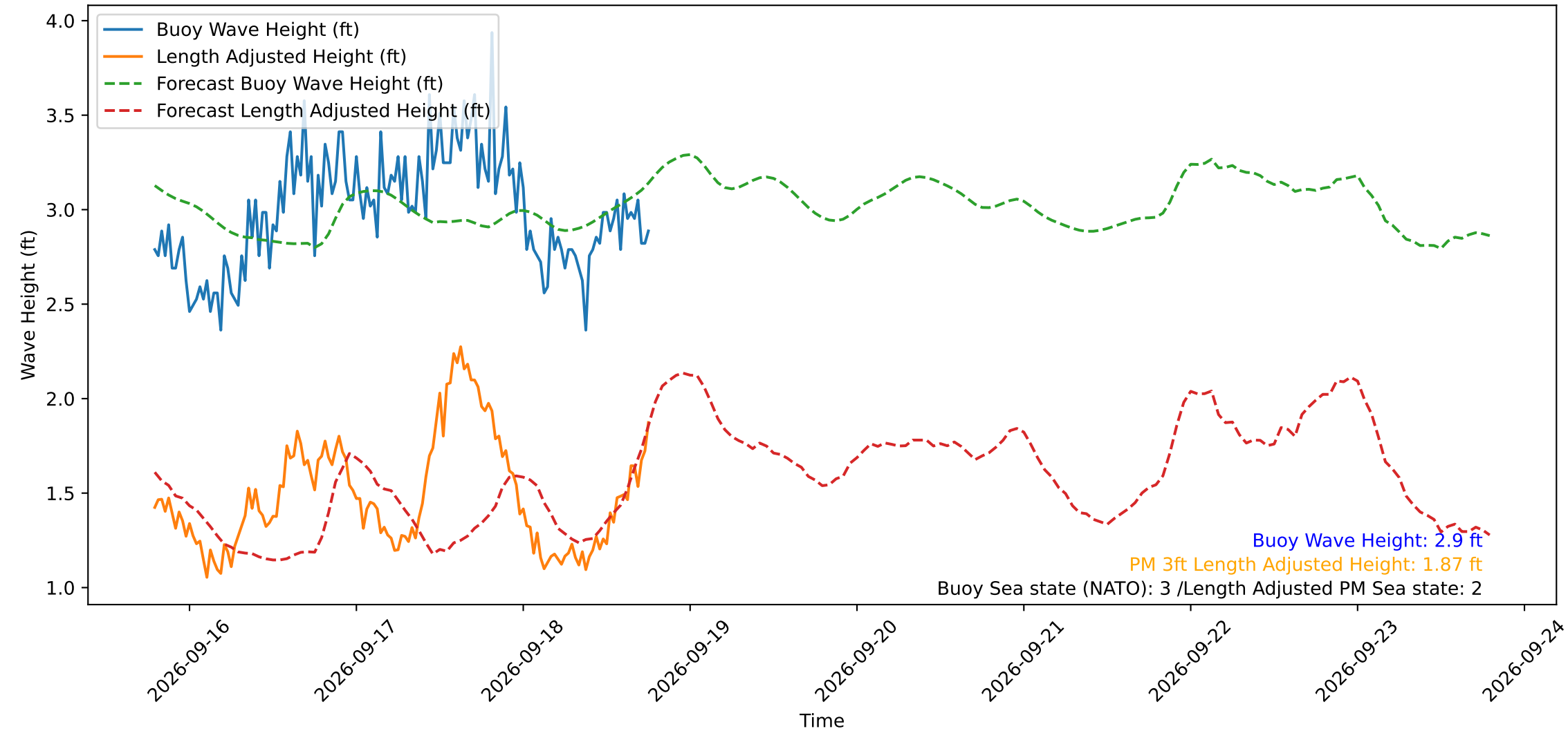
Wave Heights over Time for Oceanside Harbor at 2026-09-18 19:00:29
