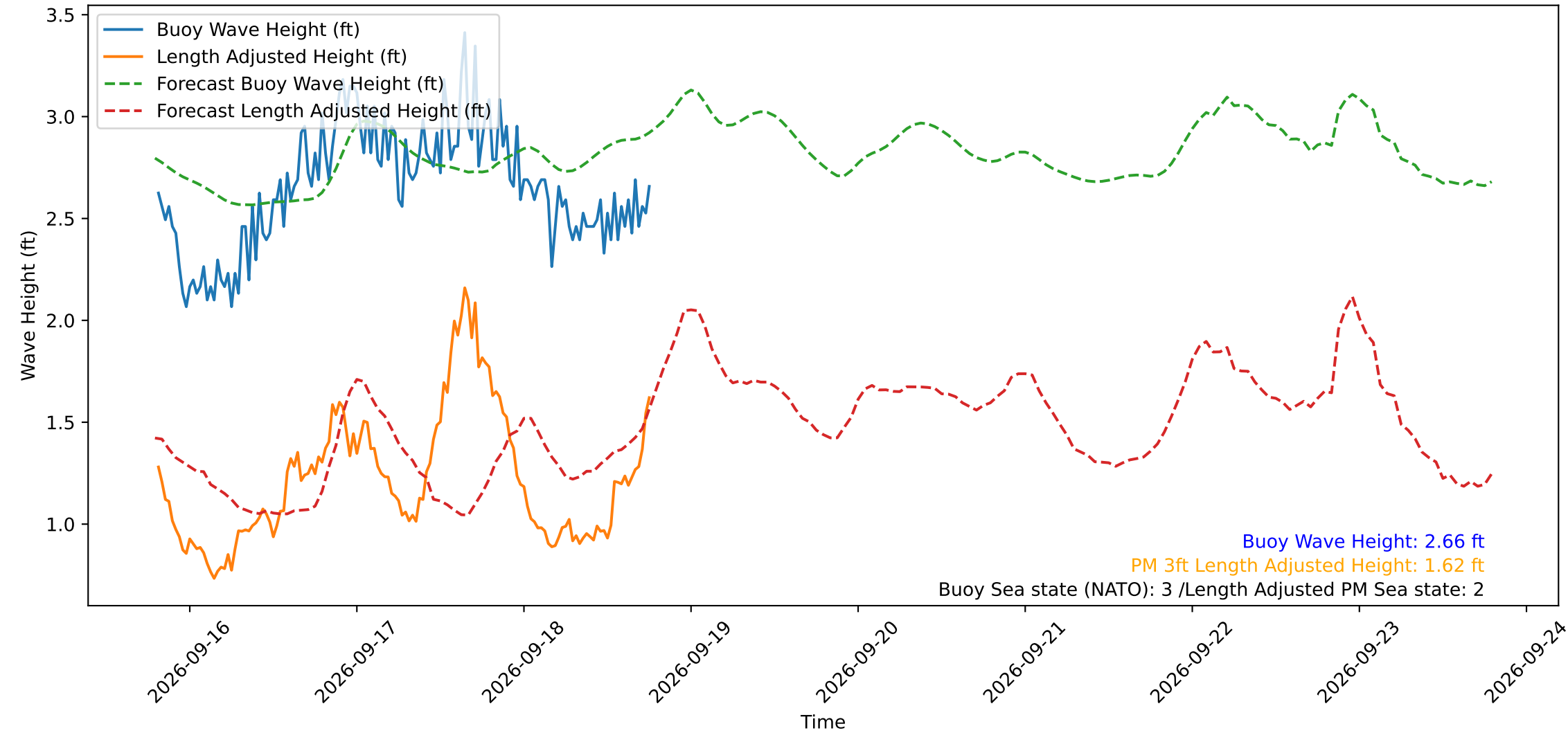
Wave Heights over Time for Red Beach at 2026-09-18 19:00:49
