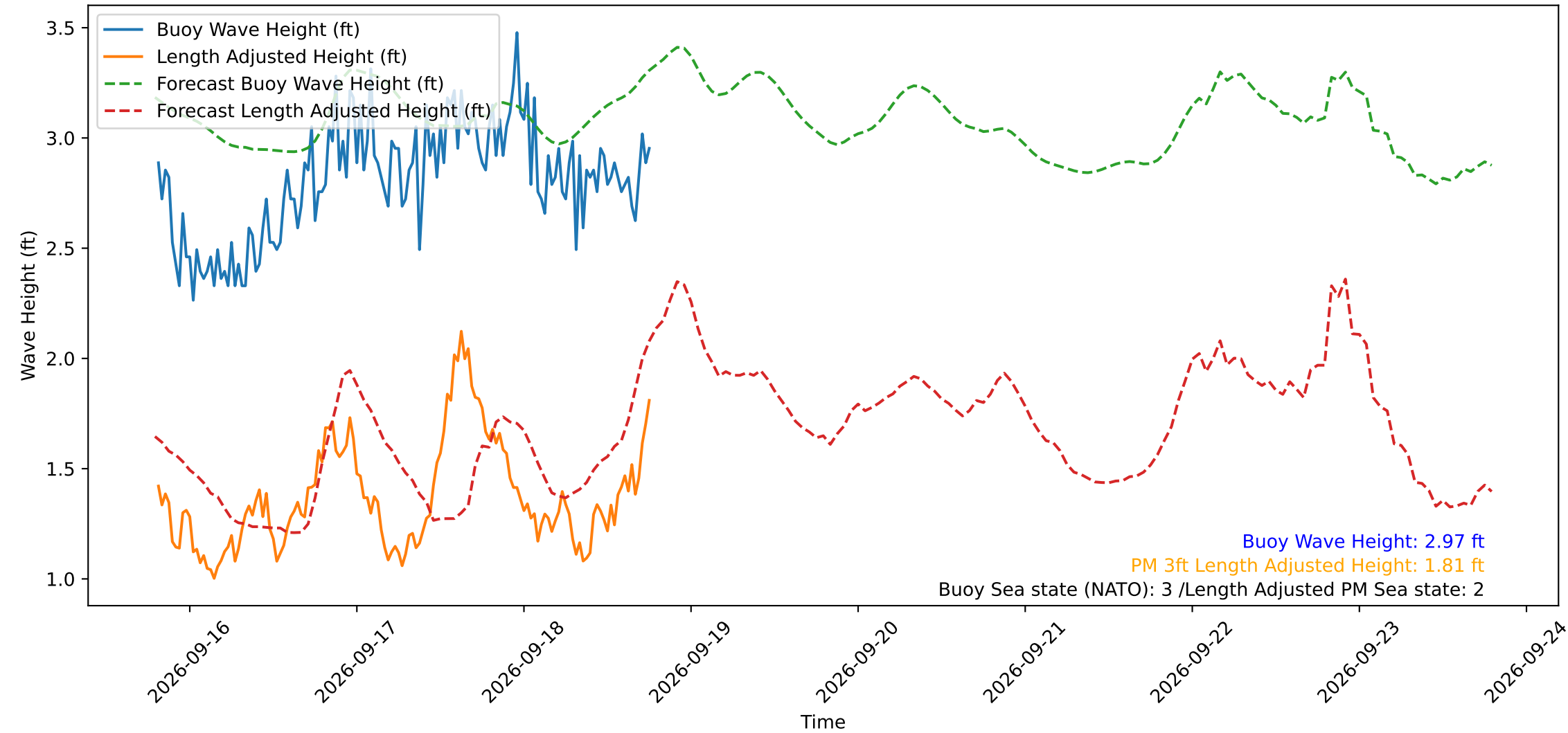
Wave Heights over Time for Green Beach at 2026-09-18 19:01:11
