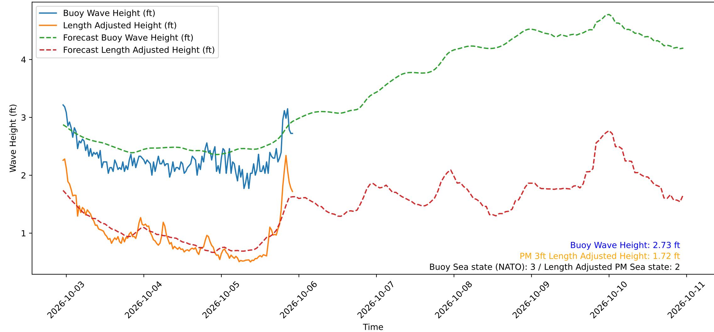
Wave Heights over Time for Green Beach at 2026-10-05 22:51:14
