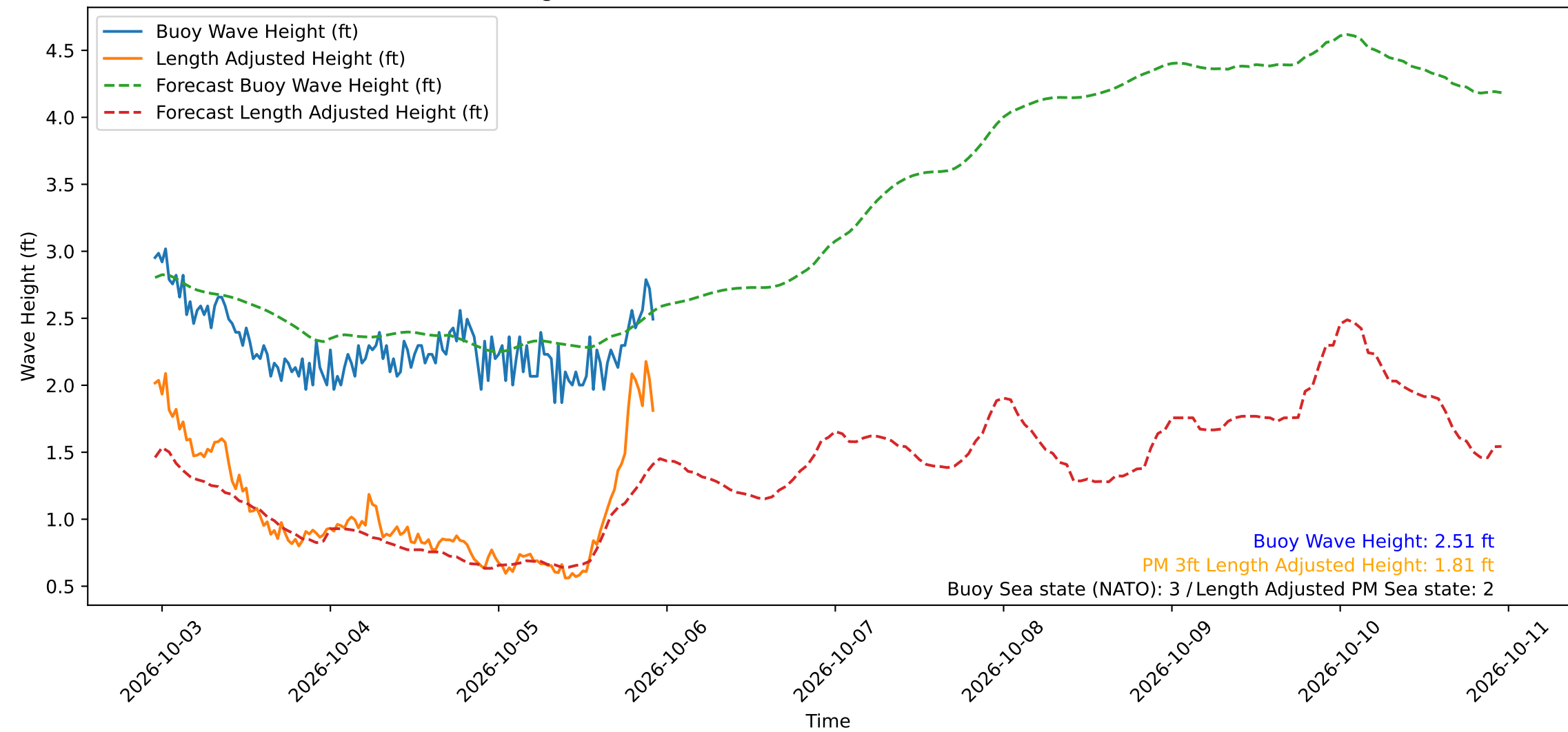
Wave Heights over Time for Oceanside Harbor at 2026-10-05 22:50:30
