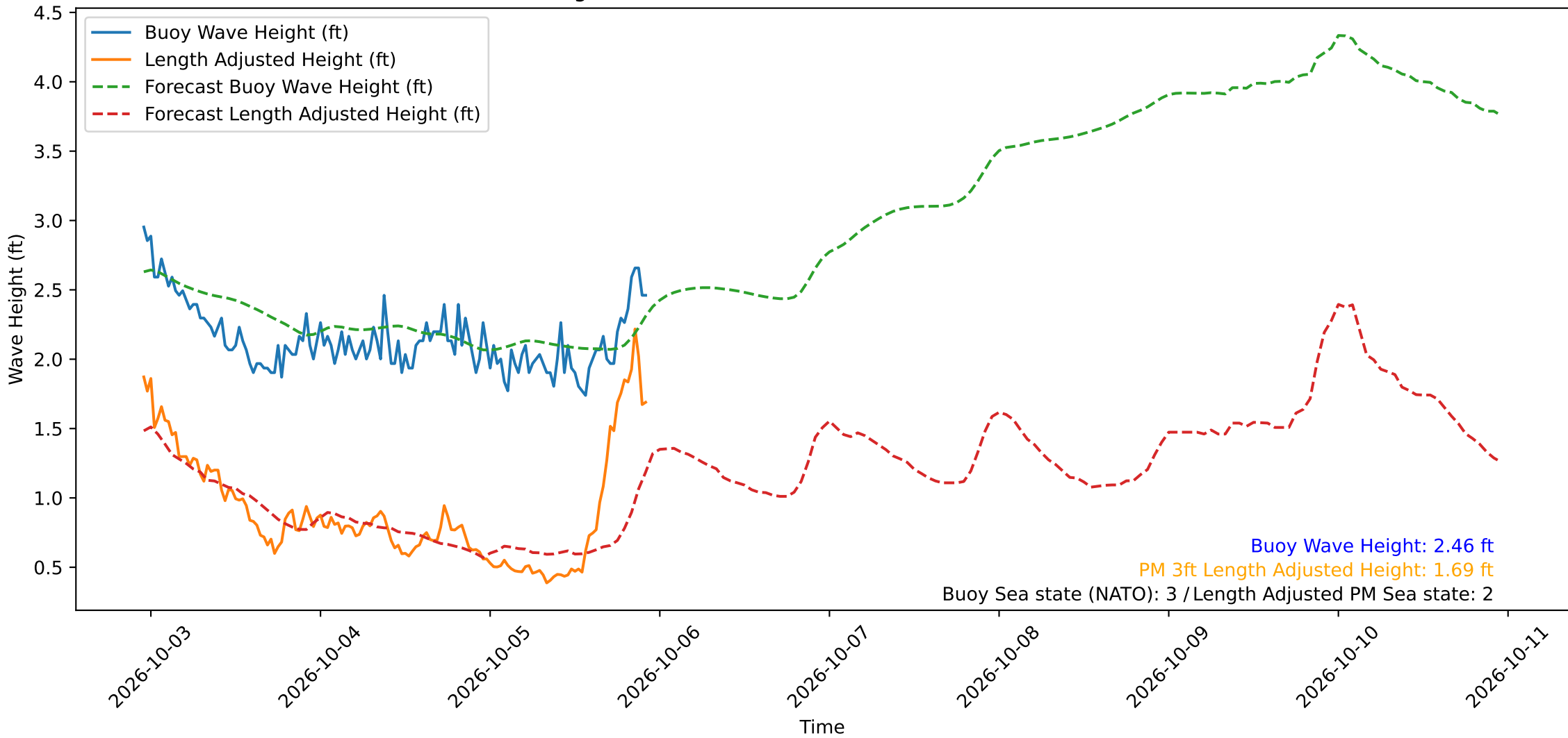
Wave Heights over Time for Red Beach at 2026-10-05 22:50:50
