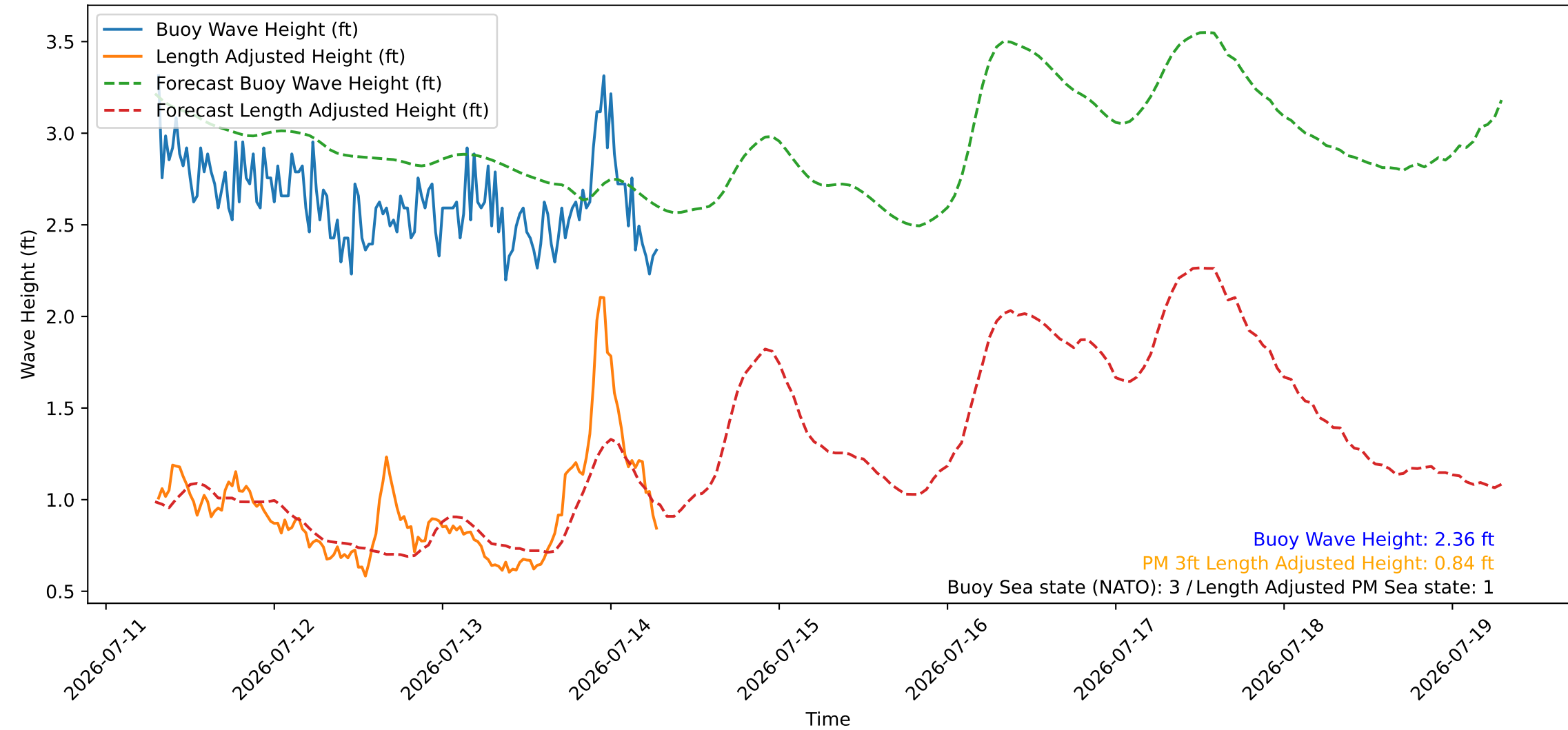
Wave Heights over Time for Green Beach at 2026-07-14 07:21:09
