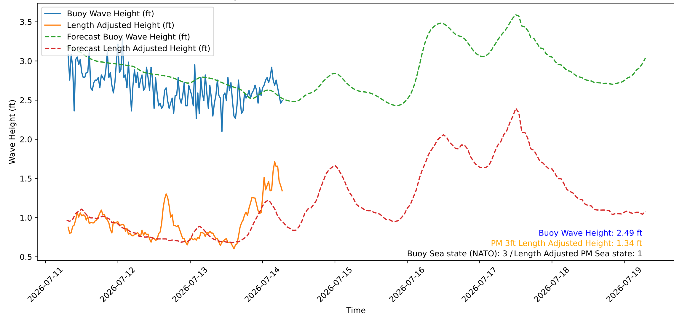
Wave Heights over Time for Oceanside Harbor at 2026-07-14 07:20:26
