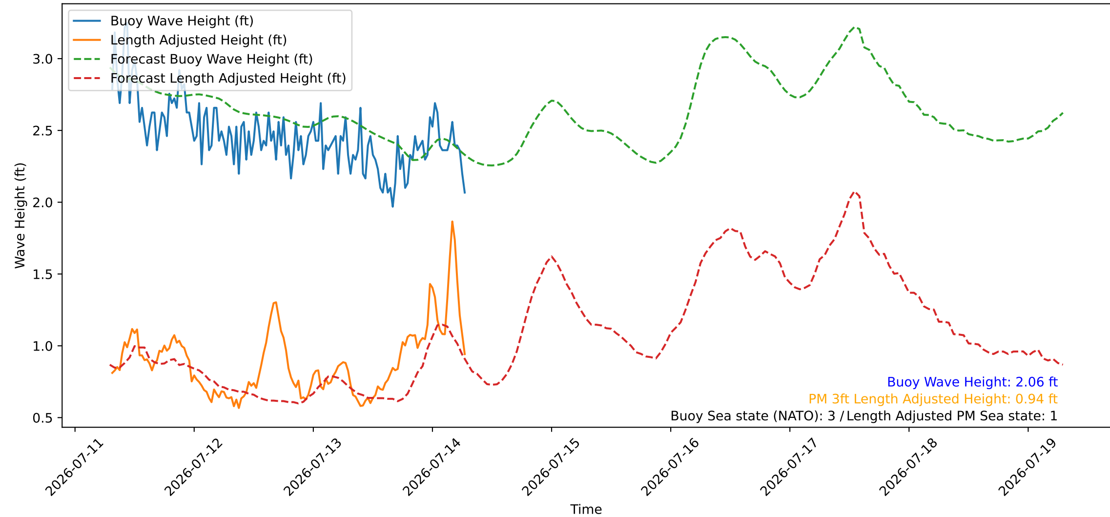
Wave Heights over Time for Red Beach at 2026-07-14 07:20:47
