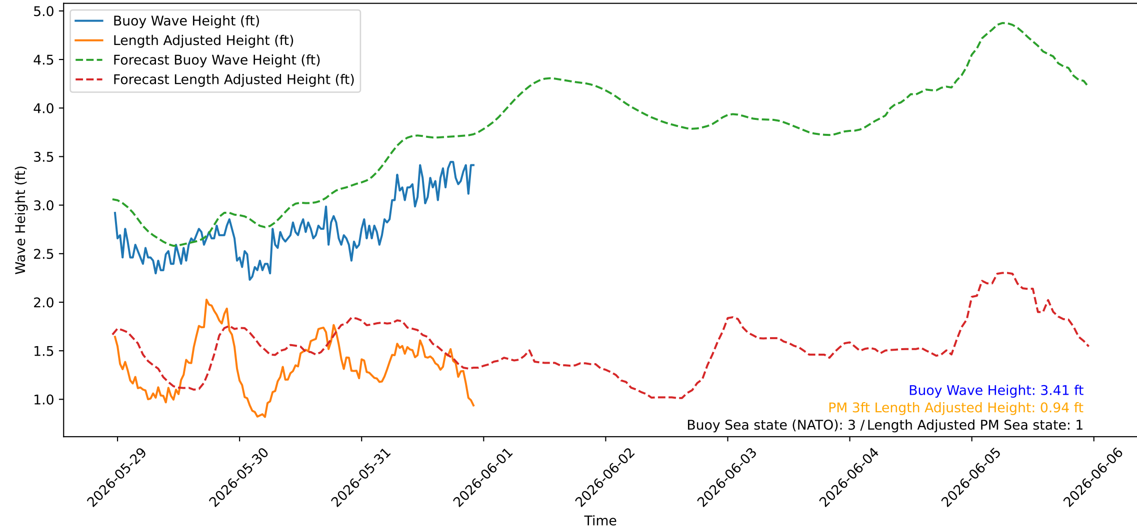
Wave Heights over Time for Red Beach at 2026-05-31 23:00:44
