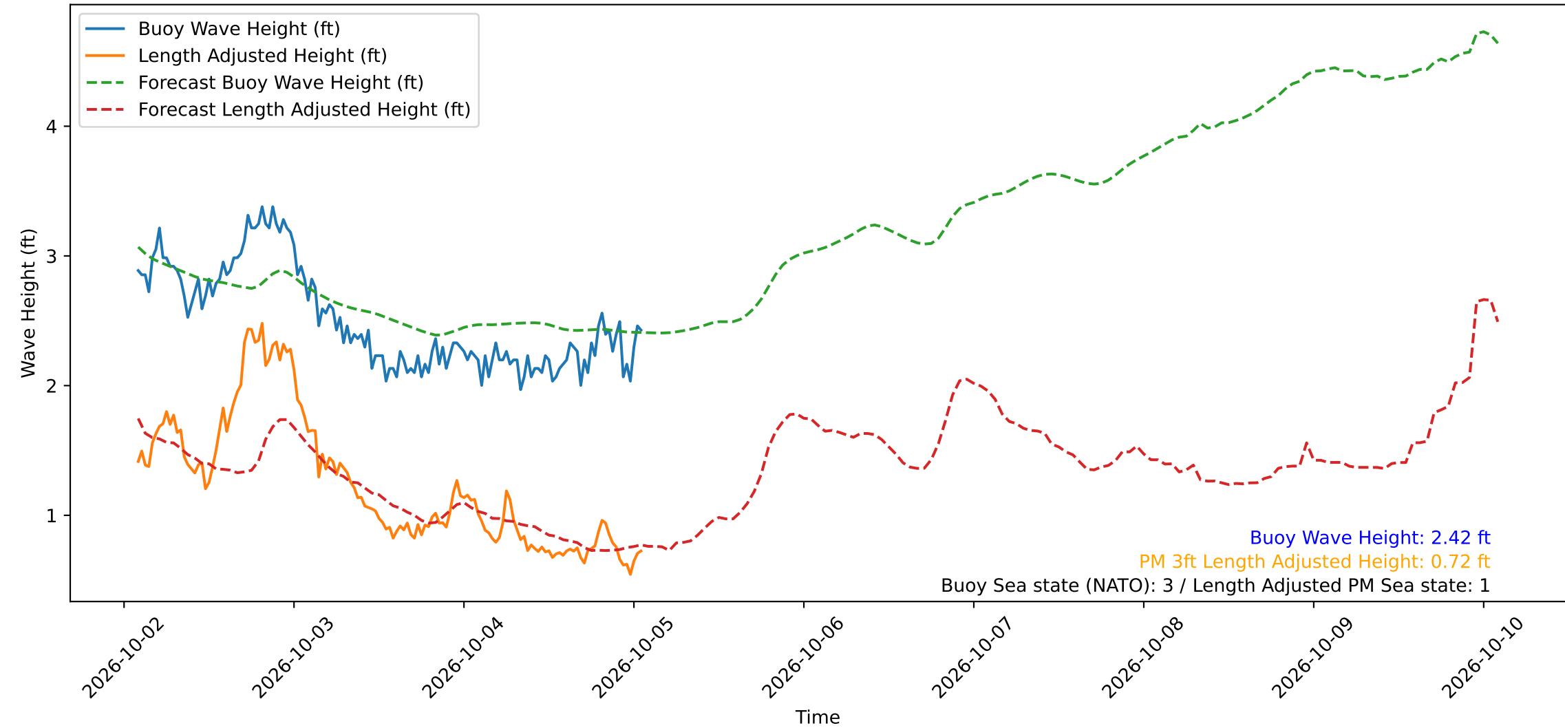
Wave Heights over Time for Green Beach at 2026-10-05 01:51:14
