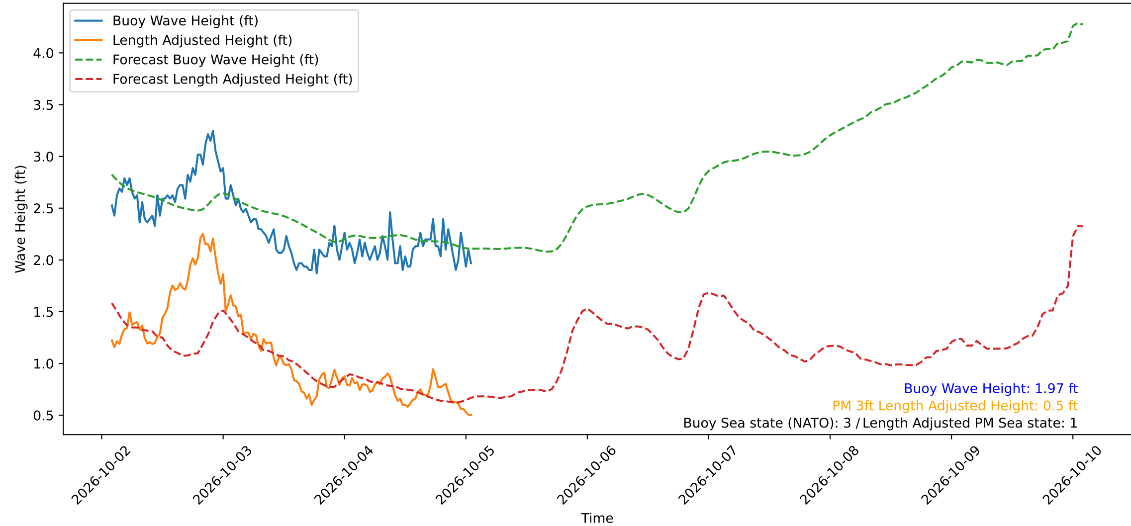
Wave Heights over Time for Red Beach at 2026-10-05 01:50:50
