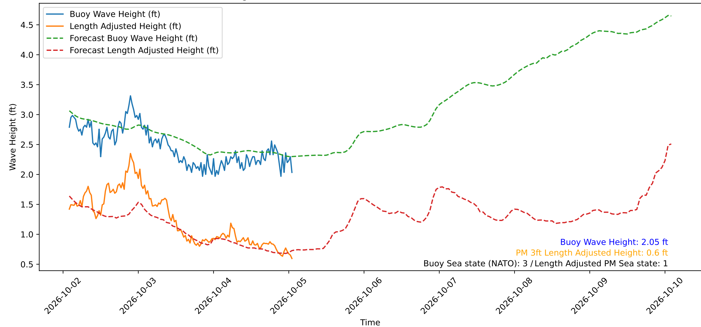
Wave Heights over Time for Oceanside Harbor at 2026-10-05 01:50:29
