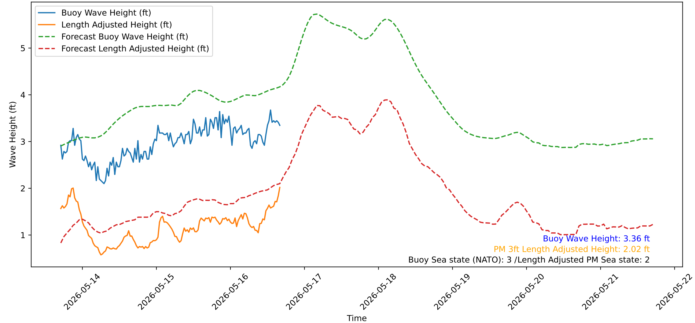
Wave Heights over Time for Green Beach at 2026-05-16 16:51:15
