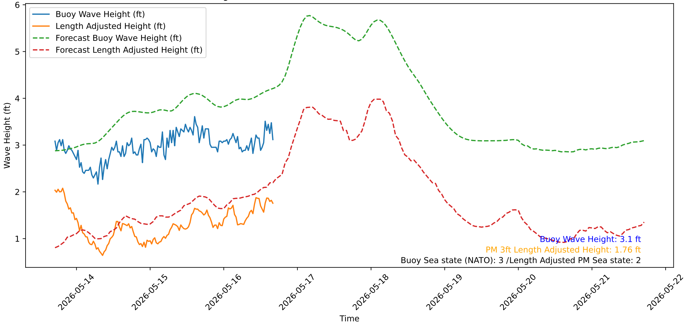
Wave Heights over Time for Oceanside Harbor at 2026-05-16 16:50:31
