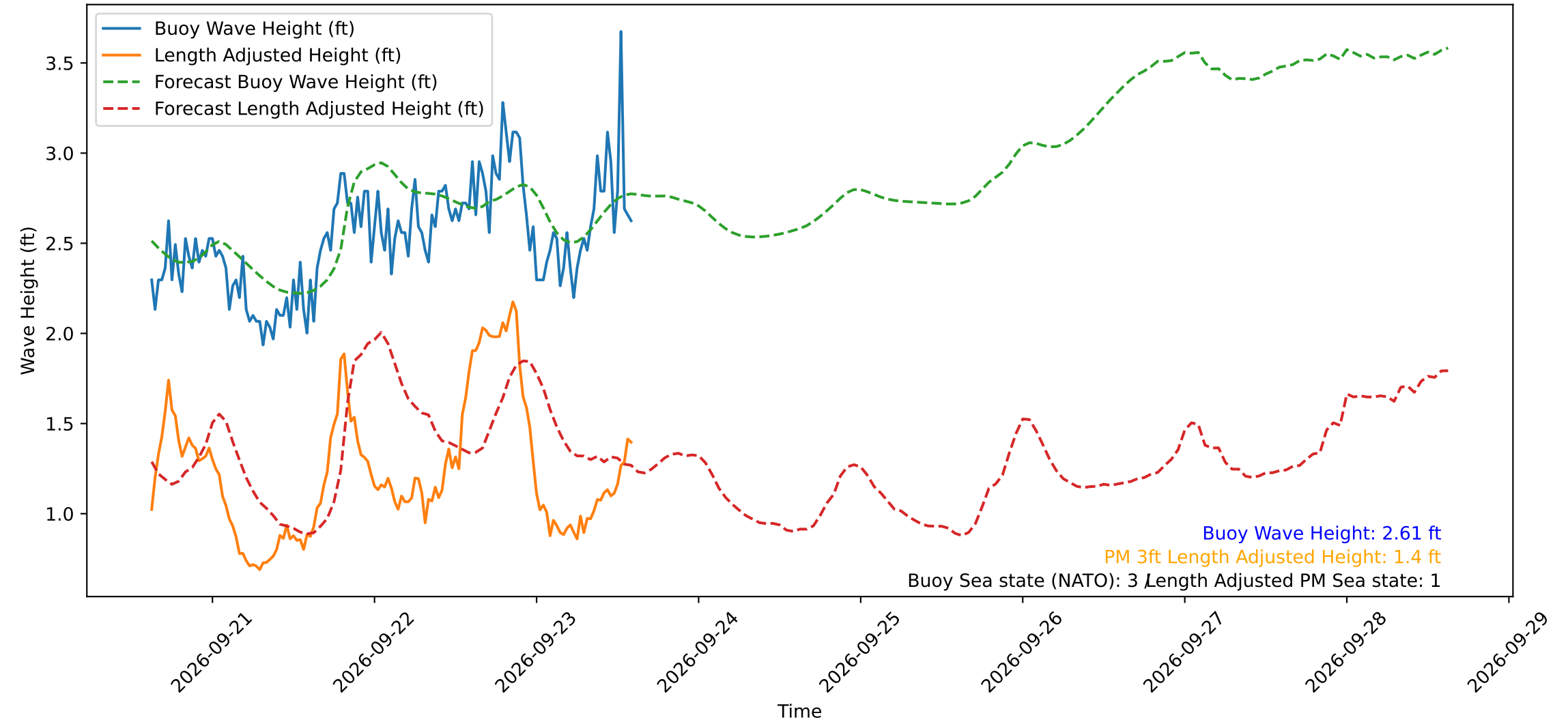
Wave Heights over Time for Red Beach at 2026-09-23 14:50:50
