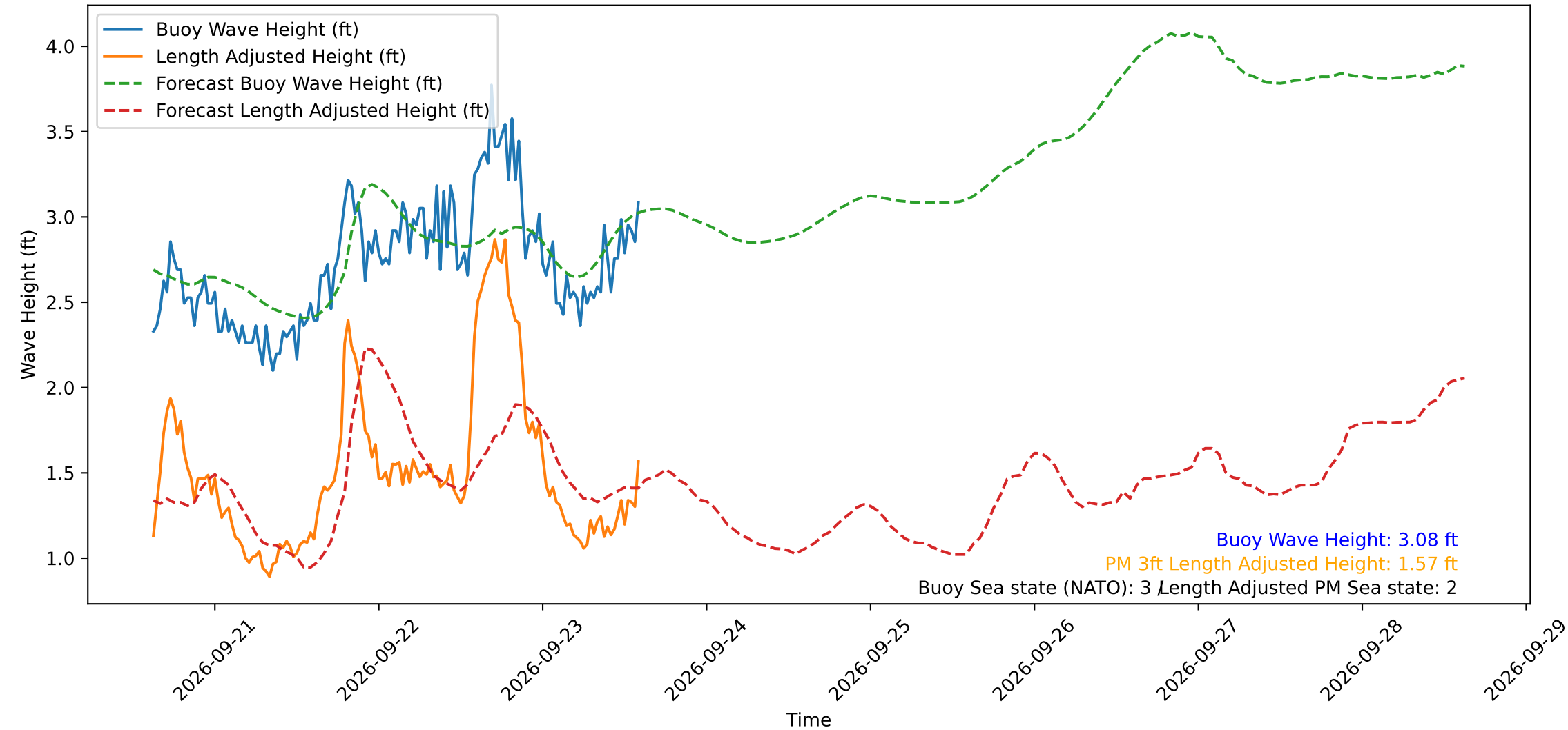
Wave Heights over Time for Oceanside Harbor at 2026-09-23 14:50:30
