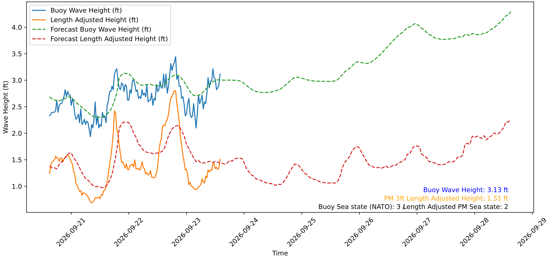
Wave Heights over Time for Green Beach at 2026-09-23 14:51:15
