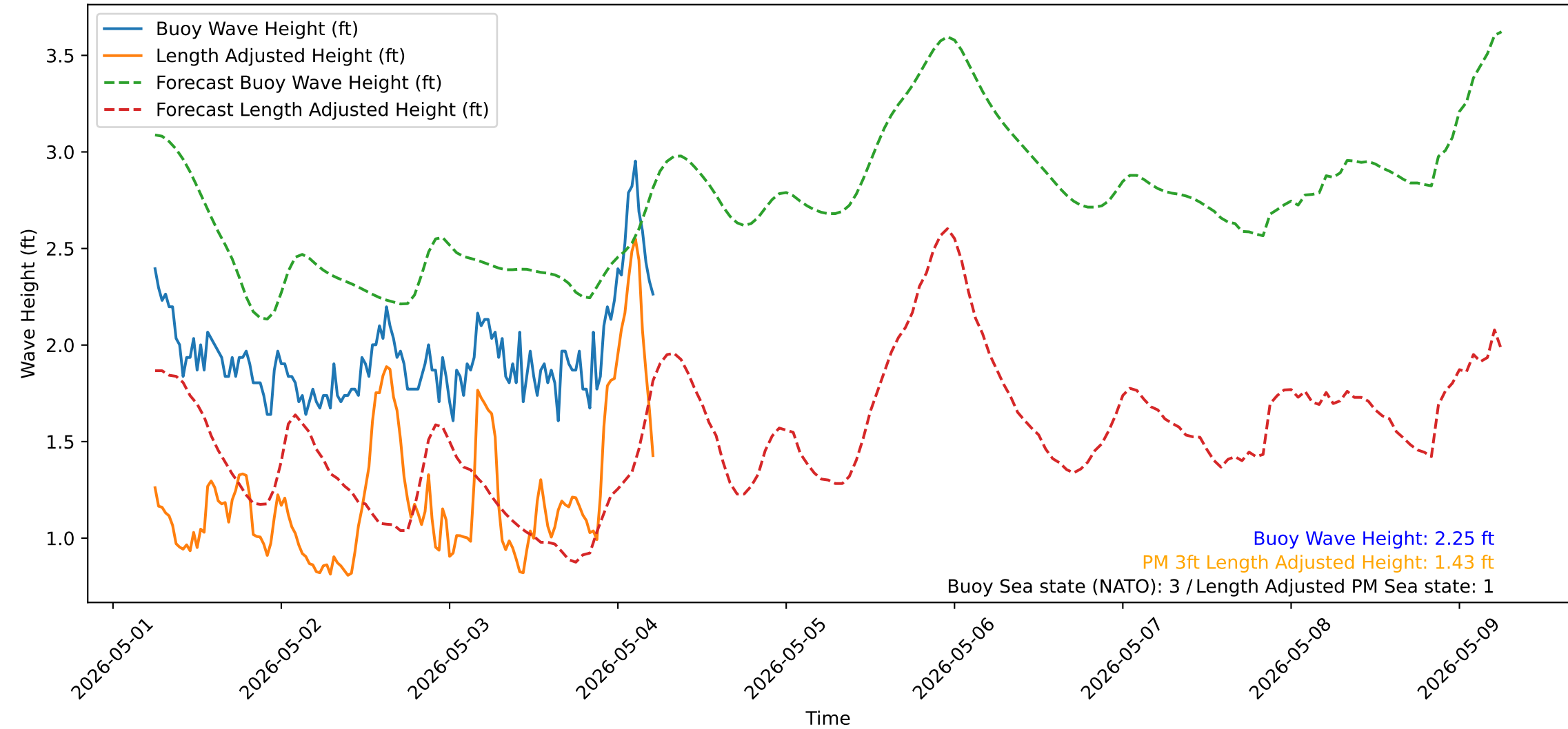
Wave Heights over Time for Red Beach at 2026-05-04 05:40:50
