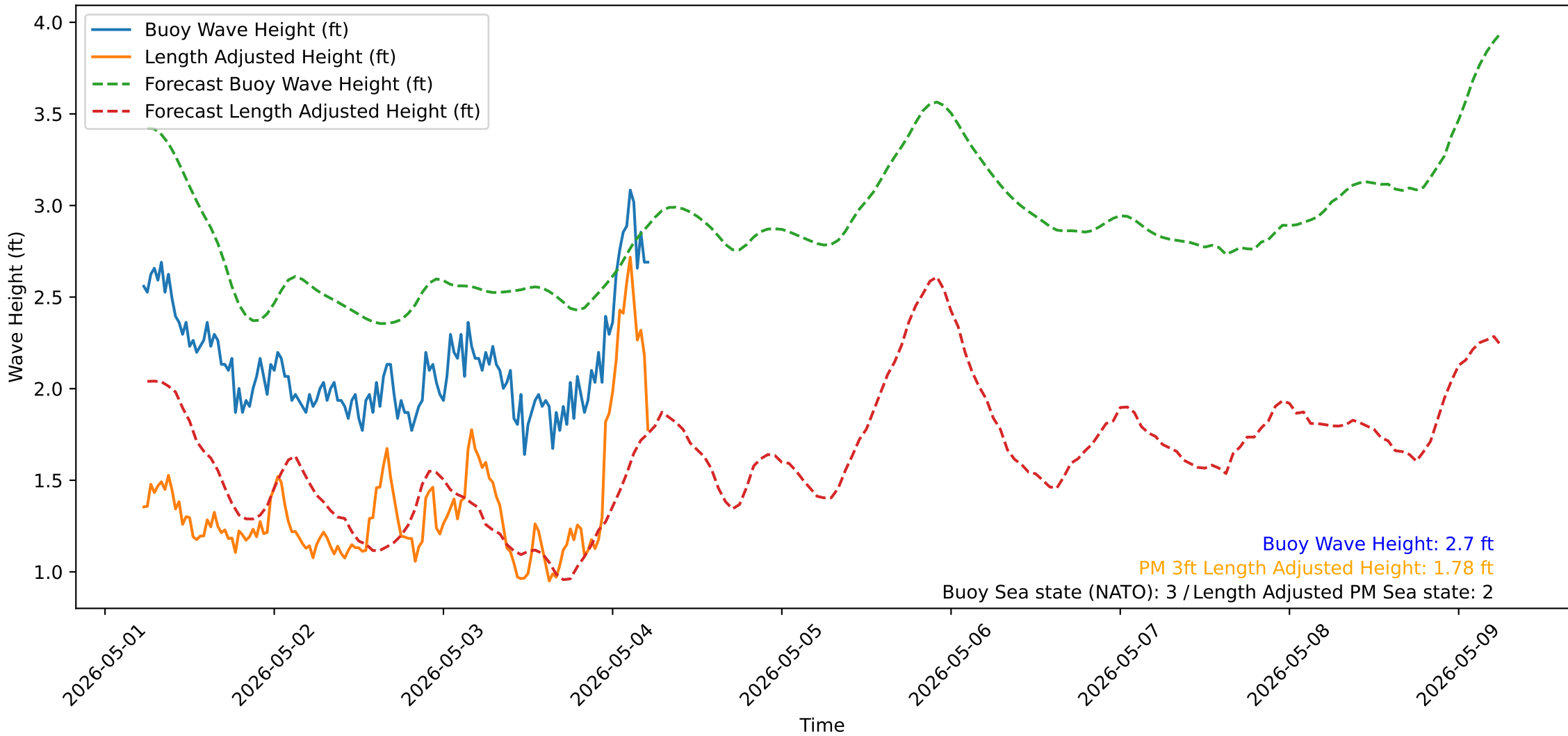
Wave Heights over Time for Oceanside Harbor at 2026-05-04 05:40:31
