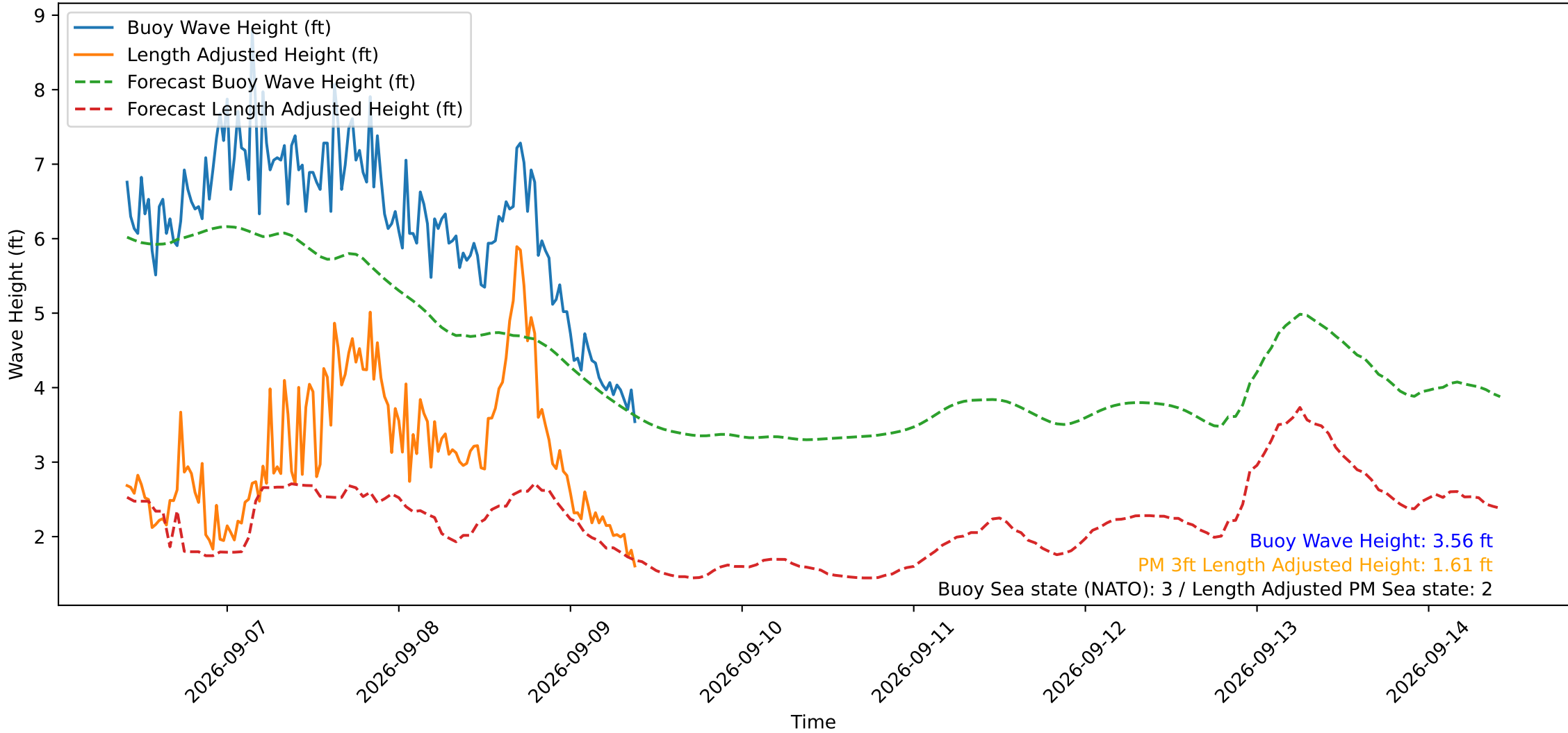
Wave Heights over Time for Green Beach at 2026-09-09 09:41:11
