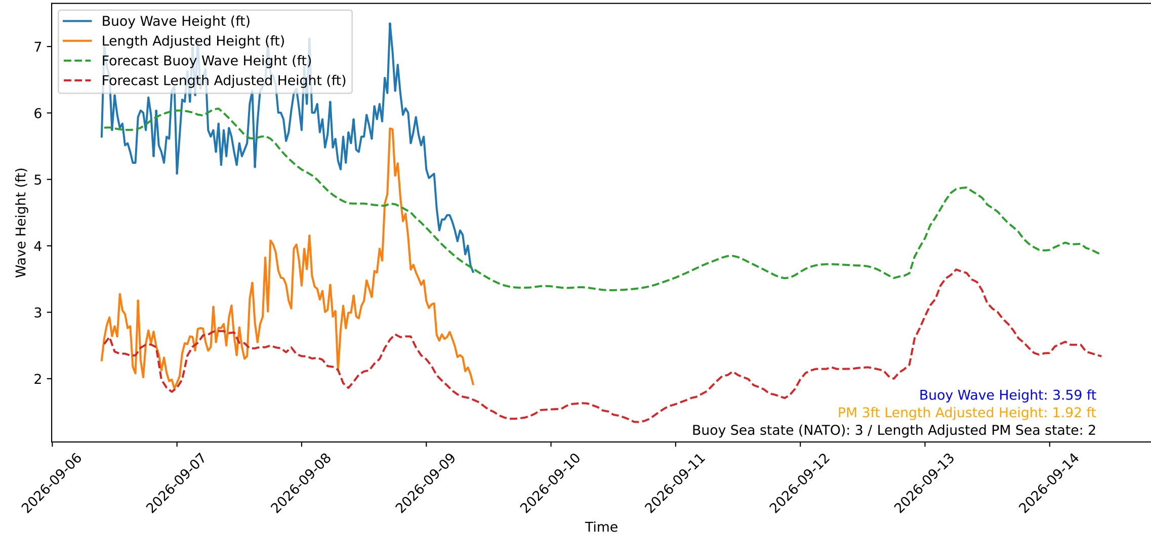
Wave Heights over Time for Oceanside Harbor at 2026-09-09 09:40:29
