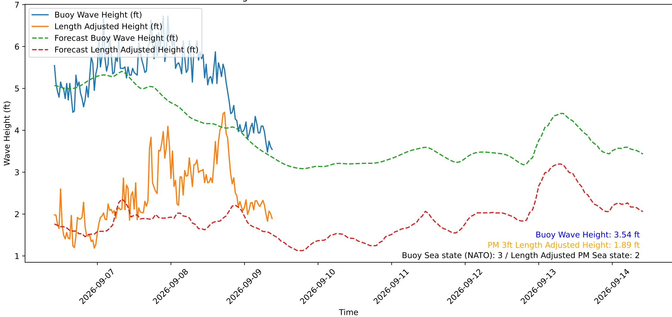
Wave Heights over Time for Red Beach at 2026-09-09 09:40:49
