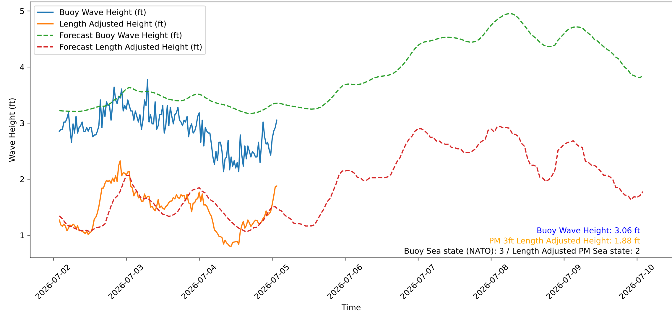
Wave Heights over Time for Oceanside Harbor at 2026-07-05 02:10:26
