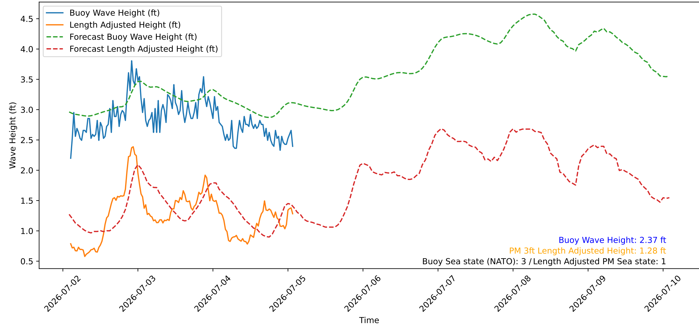
Wave Heights over Time for Red Beach at 2026-07-05 02:10:46
