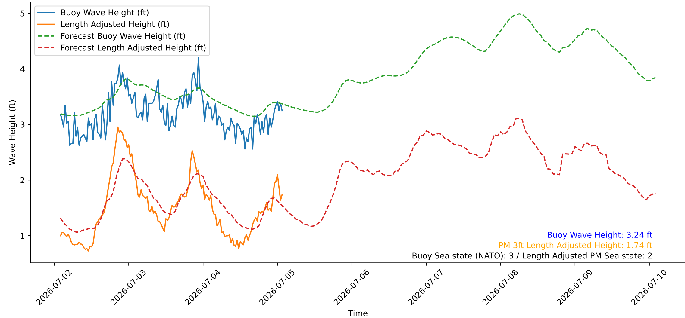
Wave Heights over Time for Green Beach at 2026-07-05 02:11:08
