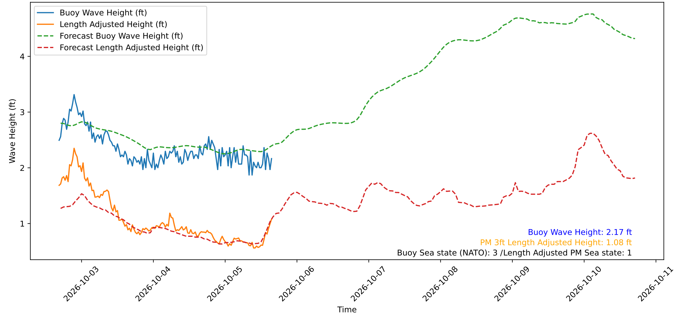
Wave Heights over Time for Oceanside Harbor at 2026-10-05 16:30:30
