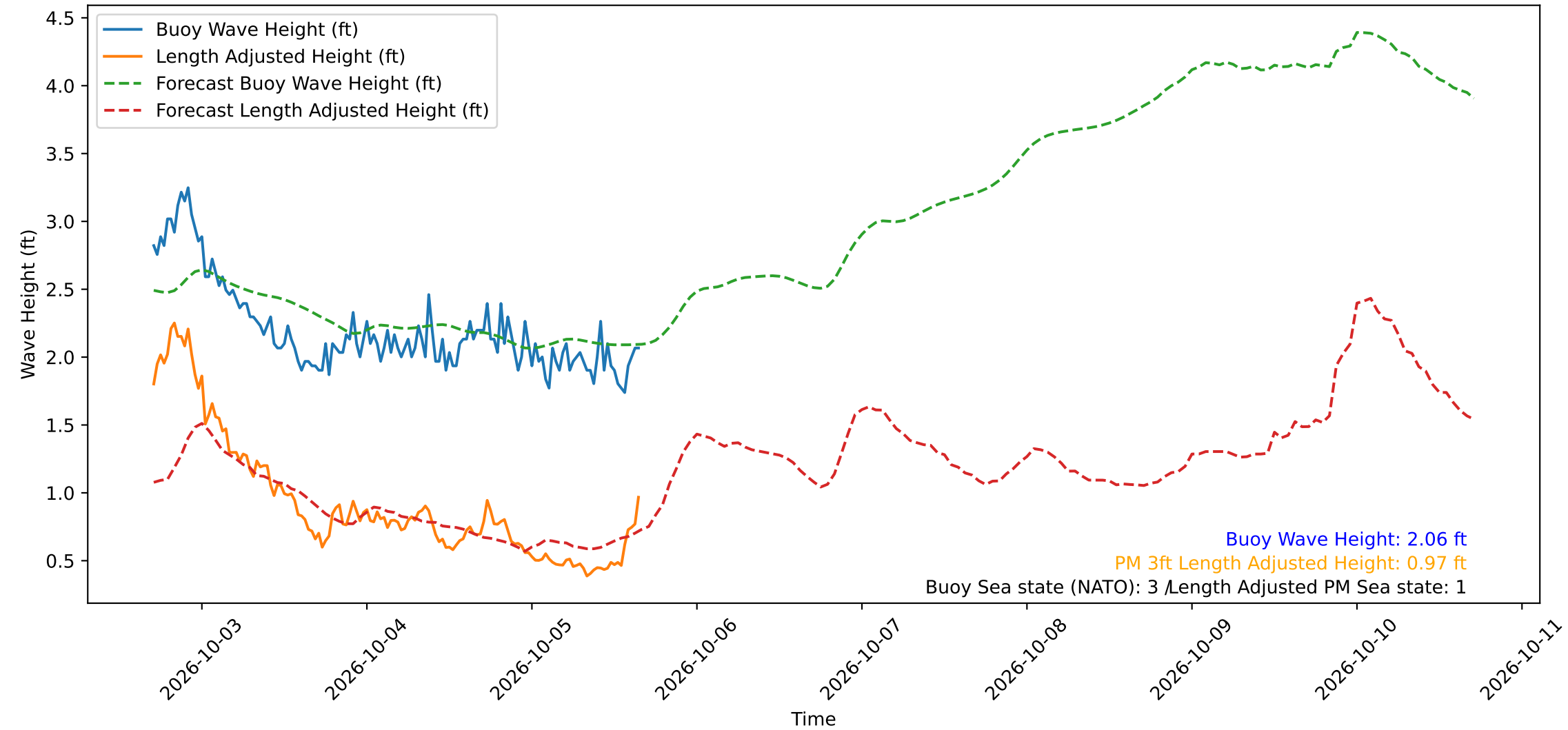
Wave Heights over Time for Red Beach at 2026-10-05 16:30:49
