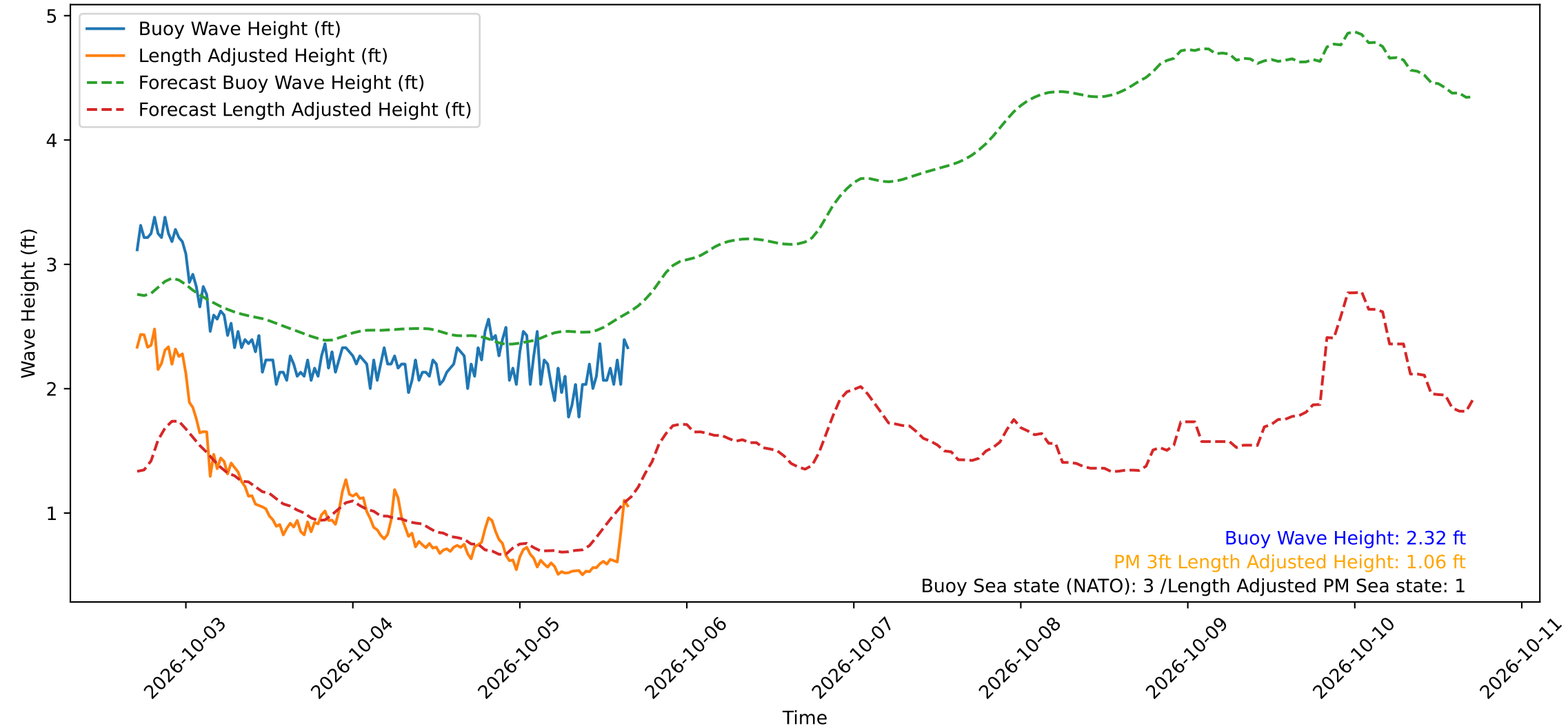
Wave Heights over Time for Green Beach at 2026-10-05 16:31:11
